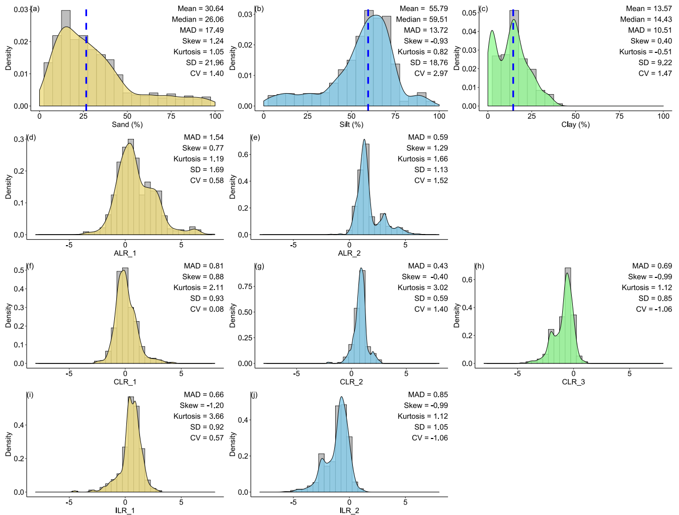
“Figure 2. Descriptive statistical analysis for the original and log ratio transformed soil sampling data of (a) sand, (b) silt, (c) clay, (d) ALR_1, (e) ALR_2, (f) CLR_1, (g) CLR_2, (h) CLR_3, (i) ILR_1 and (j) ILR_2. SD is standard deviation, CV is the coefficient of variation, and the Median is multivariate median based on depth measures. ALR and ILR transformed S^3 (the simplex) to R^2 (the real space), and CLR transformed S^3 to R^3 . Blue dashed lines showed the multivariate medians of original data.”
