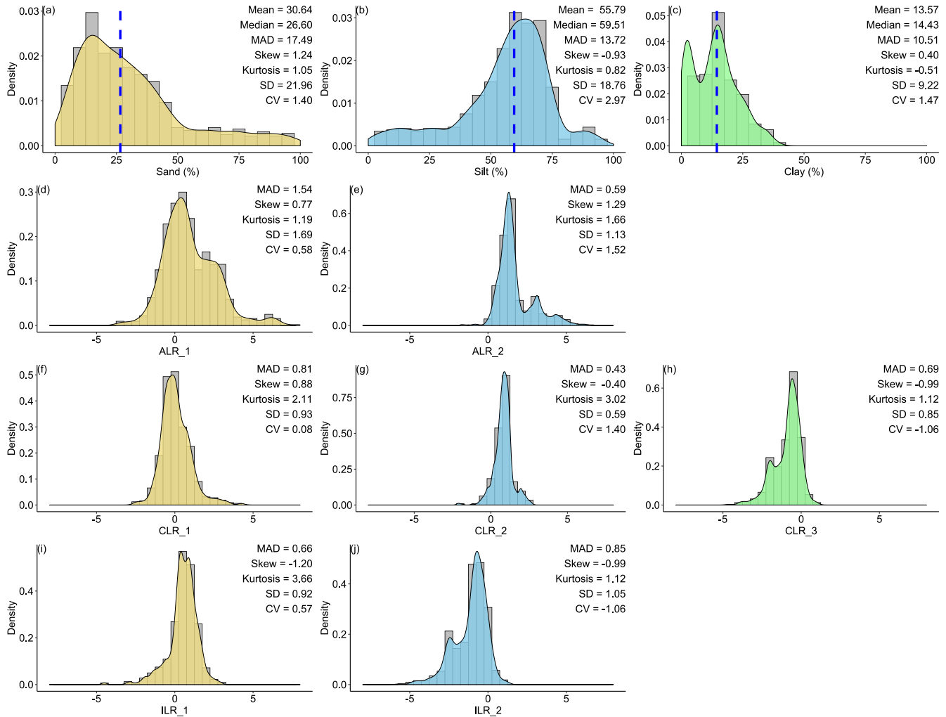
10 “Figure 2. Descriptive statistical analysis for the original and log ratio transformed soil sampling data of (a) sand, (b) silt, (c) clay, (d) ALR_1, (e) ALR_2, (f) CLR_1, (g) CLR_2, (h) CLR_3, (i) ILR_1 and (j) ILR_2. SD is standard deviation, CV is the coefficient of variation, and the Median is multivariate median based on depth measures. ALR and ILR transformed S^3 (the
