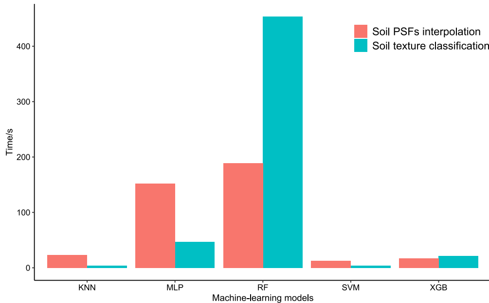
Figure 10. Average time spent running 30 times of KNN, MLP, RF, SVM and XGB of soil texture classification and soil PSFs interpolation.
