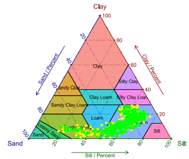
(i) SVM_ORI (66.4%)
