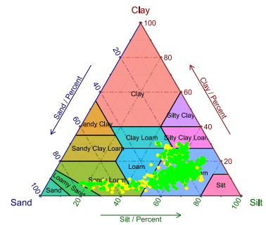
(f) RF_ILR (83.9%)
