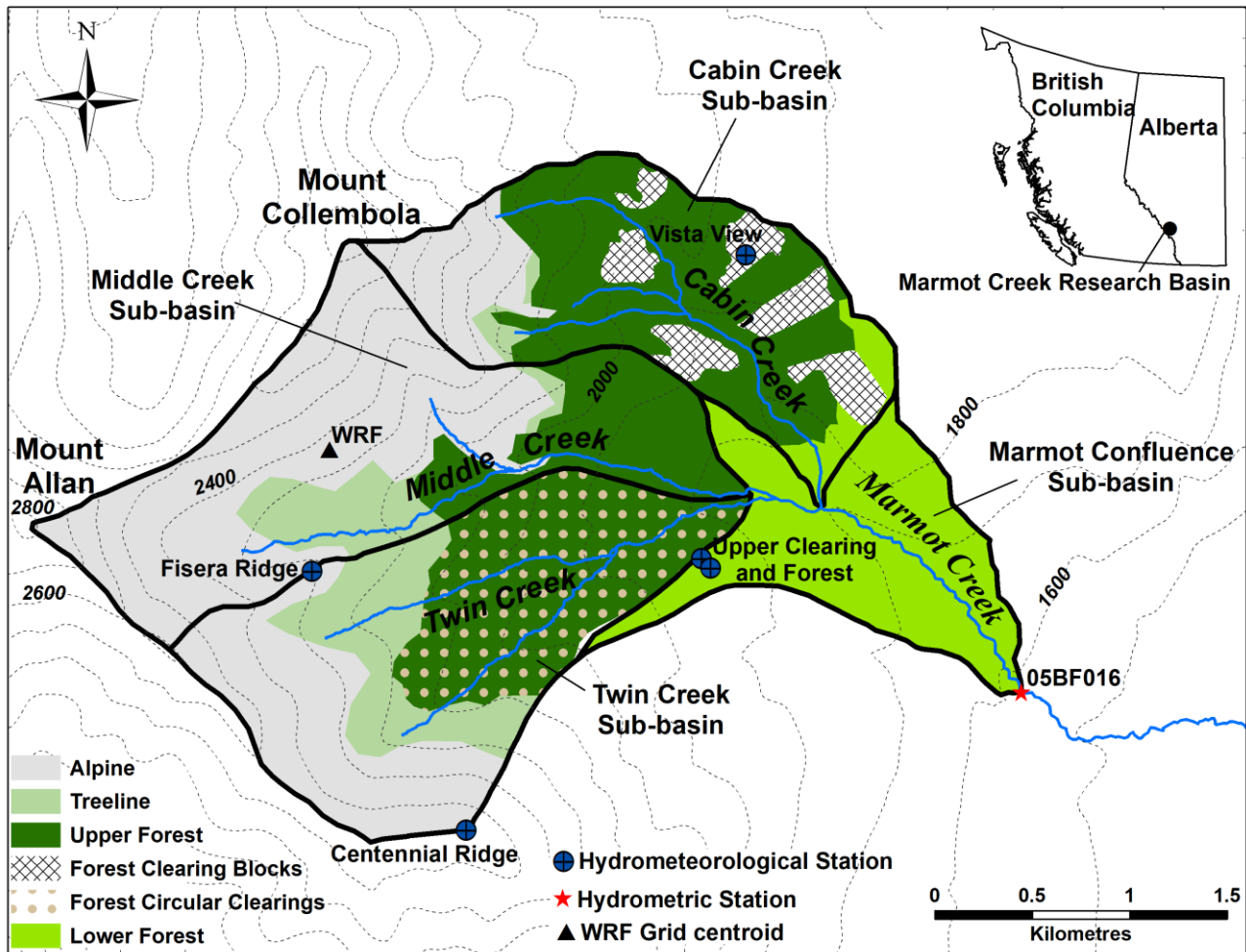
Figure 1. Location and contour map of the Marmot Creek Research Basin (MCRB), showing hydrometeorological stations, hydrometric station, WRF grid centroid, and ecozones of the MCRB: alpine, treeline, upper forest, forest clearing blocks, forest circular clearings, and lower forest. Note that WRF grid centroid represents the centre of the 4-km WRF grid, and the size and areas of circular clearings in Twin Creek are meant to represent a honeycomb pattern and are not to scale.
