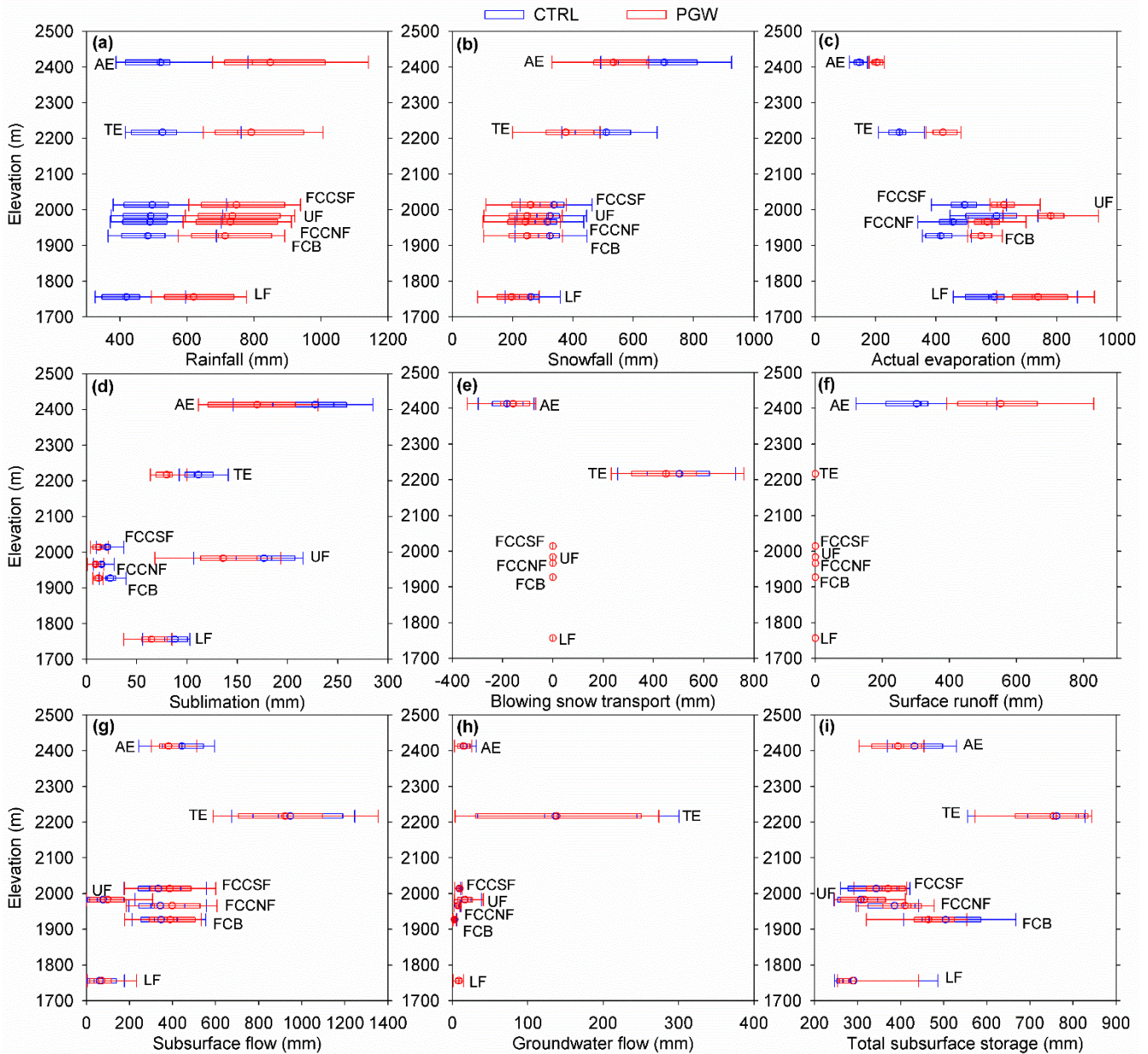
Figure 7. Boxplots of the simulated annual water balance variables for WRF CTRL and PGW for alpine (AE), treeline (TE), upper forest (UF), forest clearing blocks (FCB), forest circular clearing north-facing (FCCNF), forest circular clearing south-facing (FCCSF) and lower forest (LF) ecozones. (a) Rainfall, (b) snowfall, (c) actual evaporation, (d) sublimation, (e) blowing snow transport, (f) surface runoff, (g) subsurface flow, (h) groundwater flow, and (i) storage change. The vertical line within the box = median value of the eight-water year data, box = interquartile range (Q1: 25% to Q3: 75%) of the eight-water year data, whiskers = minimum and maximum, circle = mean value of the eight-water year data.
