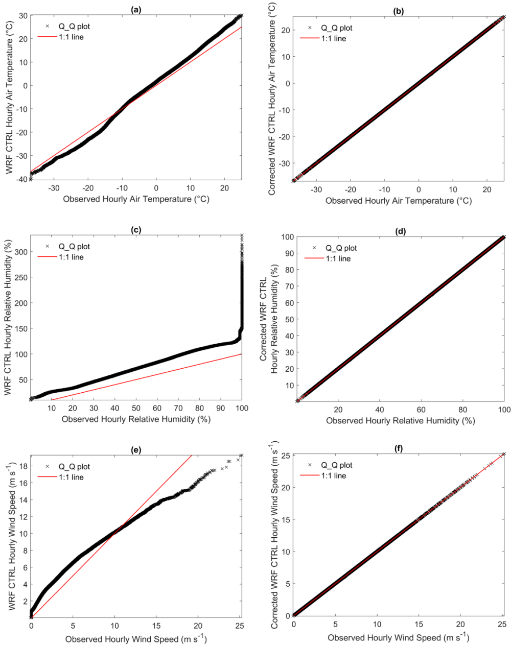
Figure 3. Quantile-quantile plots of observations and WRF CTRL outputs for the Fisera Ridge station in MCRB: (a) WRF CTRL and observed air temperature, (b) corrected WRF CTRL and observed air temperature, (c) WRF CTRL and observed relative humidity (d) corrected WRF CTRL and observed relative humidity, (e) WRF CTRL and observed wind speed (f) corrected WRF CTRL and observed wind speed, (g) WRF CTRL and observed incoming solar radiation (h) corrected WRF CTRL and observed incoming solar radiation, (i) WRF CTRL and observed precipitation (j) corrected WRF CTRL and observed precipitation.
