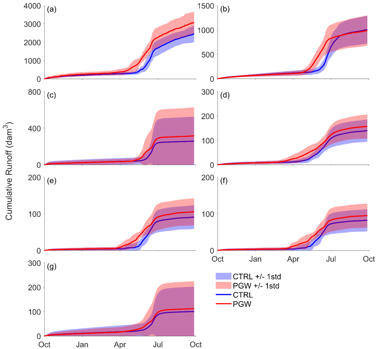
Figure 13. Simulated mean annual cumulative runoff for WRF CTRL and PGW. (a) Alpine, (b) treeline, (c) upper forest, (d) forest clearing blocks, (e) forest circular clearing north-facing, (f) forest circular clearing south-facing, and (g) lower forest ecoregions. The line represents the mean and the shadow represents the standard deviation of the eight-water year runoff.
