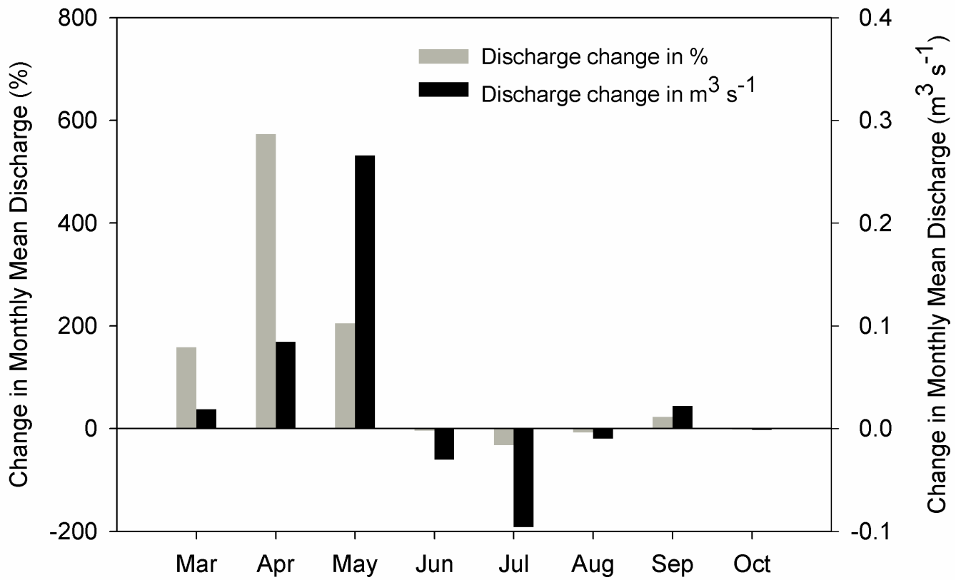
Figure 11. Change between WRF CTRL and PGW periods in the simulated mean Marmot Creek monthly streamflow discharges during March to October for the eight-water years.
