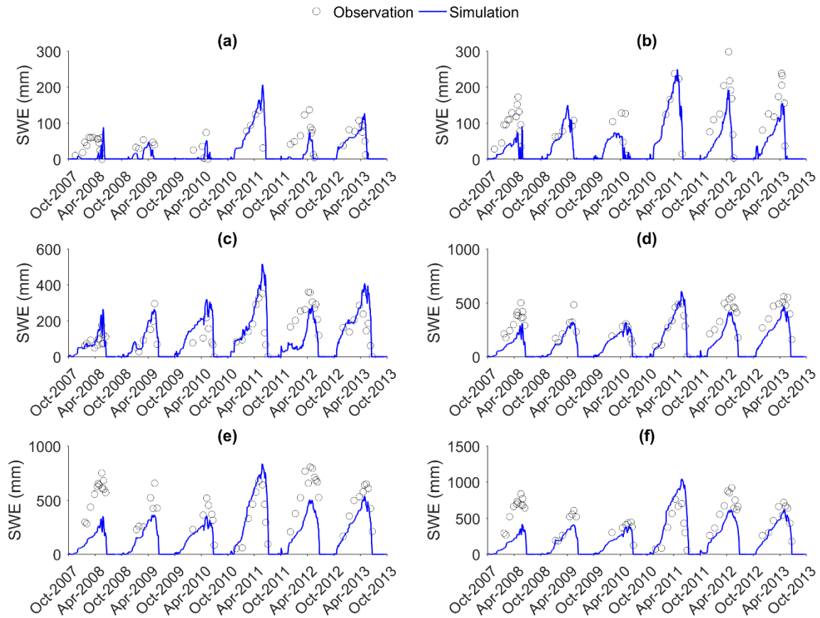
Figure 4. Comparison of the observed and simulated snow accumulation (SWE) for 2007-2013 at the sheltered, mid-elevation Upper Forest/Clearing and the wind-blown, high-elevation Fisera Ridge sites in MCRB. (a) Mature spruce forest, (b) forest clearing, (c) ridge top, (d) upper alpine south-facing slope, (e) lower upper alpine south-facing slope, and (f) larch forest treeline.
