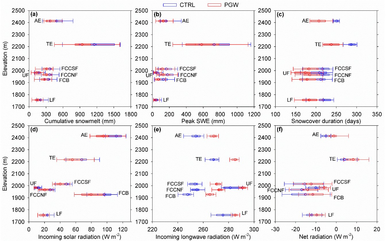
Figure 9. Boxplots of the simulated water year (a) cumulative snowmelt, (b) peak snow accumulation (SWE), (c) snowcover duration, (d) incoming solar radiation to snow, (e) longwave irradiance to snow, and (f) net radiation to snow for WRF CTRL and PGW for alpine (AE), treeline (TE), upper forest (UF), forest clearing blocks (FCB), forest circular clearing north-facing (FCCNF), forest circular clearing south-facing (FCCSF), lower forest (LF) ecozones. The vertical line within the box = median value of the eight-water year data, box = interquartile range (Q1: 25% to Q3: 75%) of the eight-water year data, whiskers = minimum and maximum, circle = mean value of the eight-water year data.
