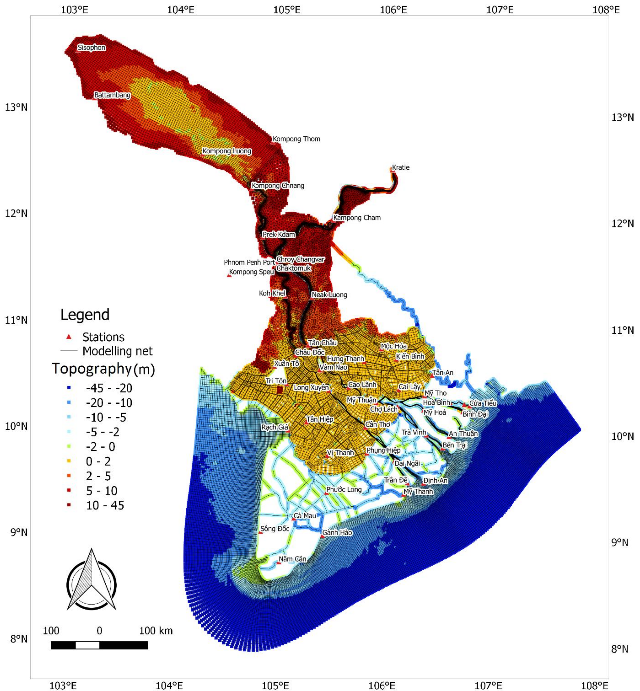
Figure 6. Mekong Delta modelling grid and river interpolated topography from 1D ISIS cross-section data and shelf topography of the Mekong Delta.
