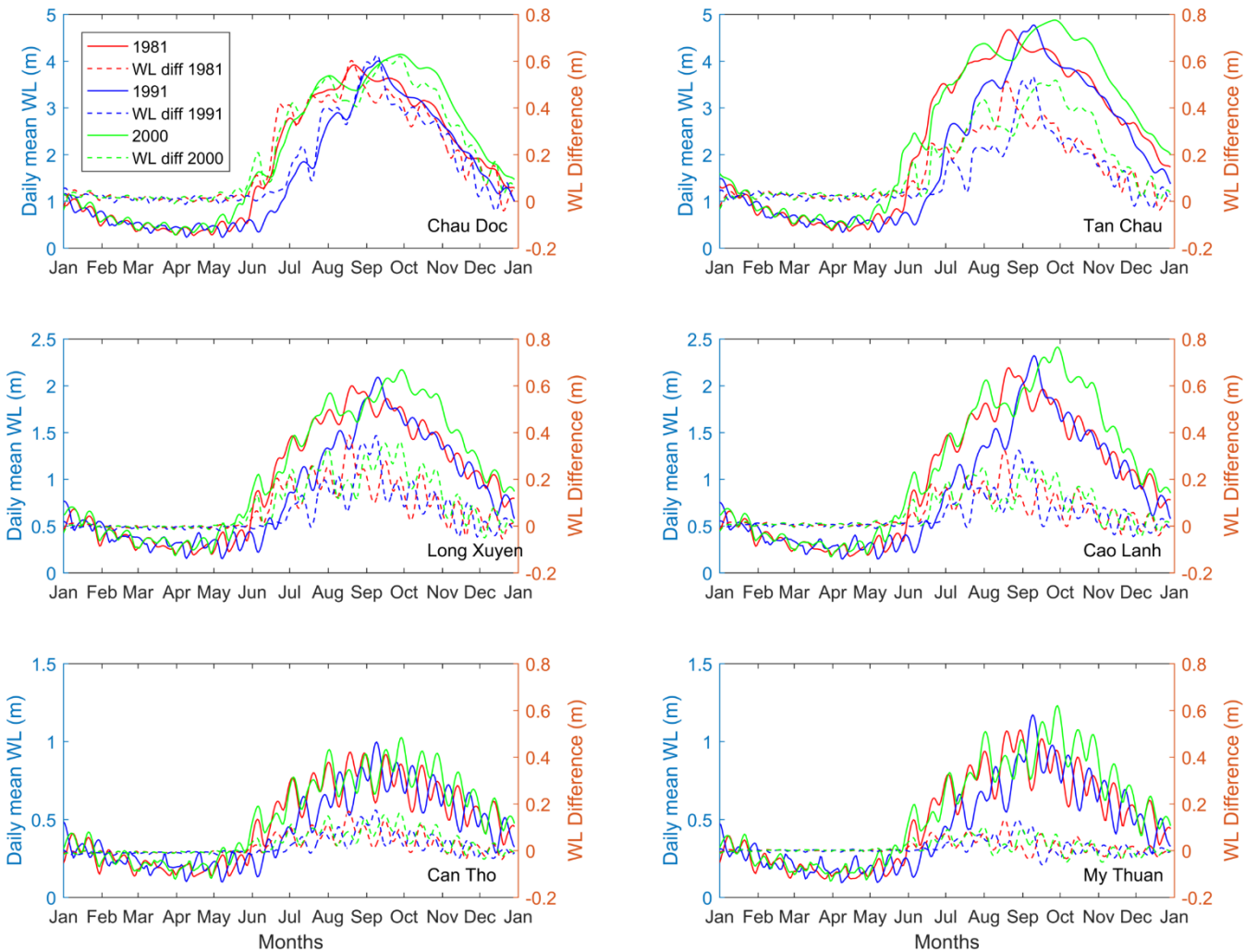
Figure 12. Simulated daily mean water levels in high-flood years of 1981, 1991 and 2000 at selected stations on the Mekong River. The dashed lines indicate water level differences due to impacts of high dykes.
