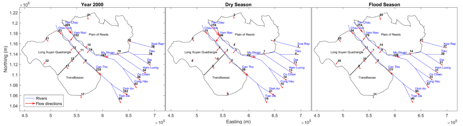
Figure 7. Spatial distribution of water volume (km³) throughout the VMD in 2000. The low flow season is calculated from 01/Jan to 30/Jun and the high flow season is from 01/Jul to 30/Oct.
