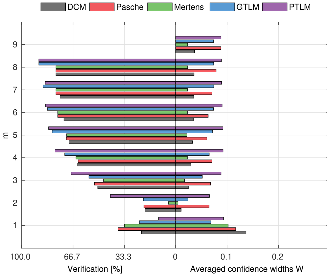
Figure 10. Percentage of verification set ( M - m ) enclosed by confidence intervals and average width of confidence intervals for different number of data points for model identification ( m ); flume data set, case 1.
