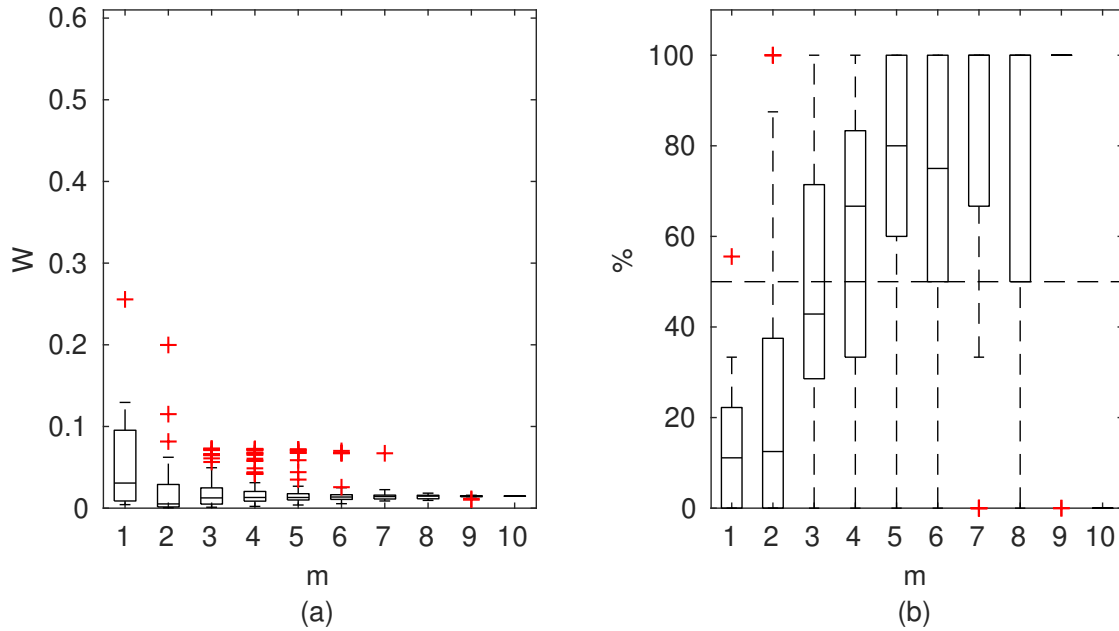
Figure 7. Pasche results for the flume data set, case 2: (a) Averaged relative confidence widths W as a function of observation set size m used for model identification; (b) Percentage of verification points enclosed by confidence intervals (100% denotes all points within intervals, box spans over 25% and 75% quantile, median is given with horizontal line, whiskers indicate the result extent, cross marks are for extreme values)
