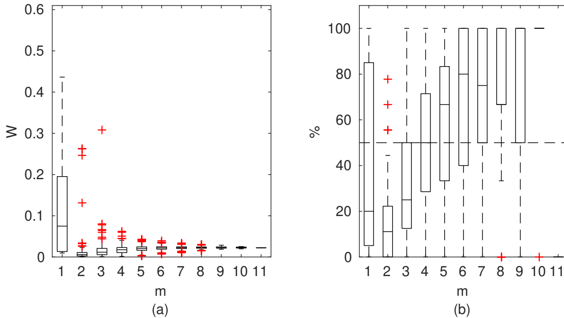
Figure 6. GTLM results for Ritobacken case study, Spring 2012: (a) Averaged relative confidence widths W as a function of observation set size m used for model identification; (b) Percentage of verification points enclosed by the confidence intervals (100% denotes all points within intervals, box spans over 25% and 75% quantile, median is given with horizontal line, whiskers indicate the result extent, cross marks are for extreme values)
