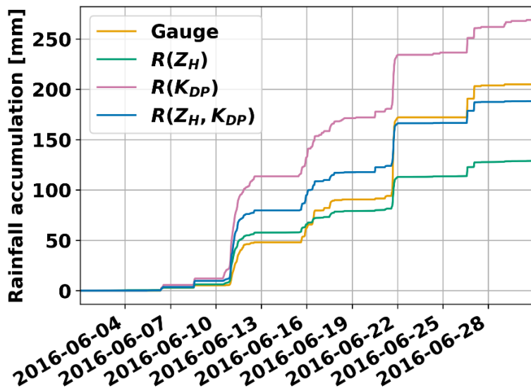
Figure 3. One month 1-hour rainfall cumulative accumulations, Sürgavere radar data, Tartu-Tõravere station gauge data. Z_H not corrected for attenuation.
