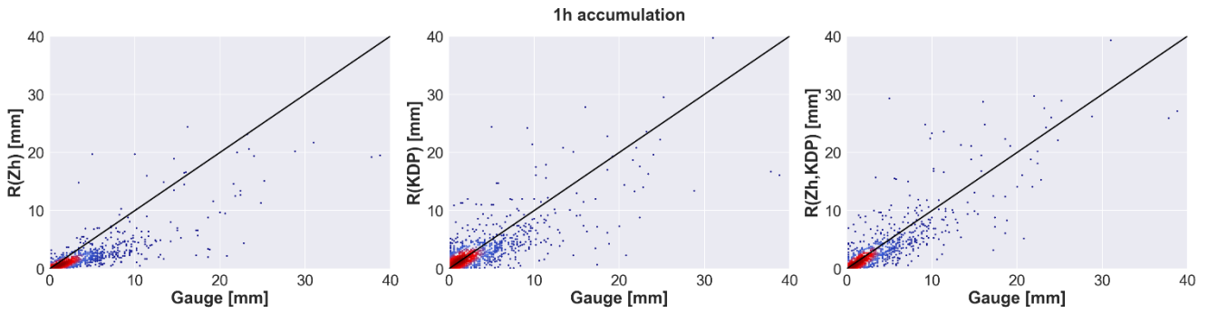
Figure 6. Italy 1-hour accumulations 2012-2016. The corresponding verification measures are presented in Table 4. The number of radar-gauge data pairs with 42 gauges and accumulations > 0.1 mm is 1,233. Z_H not corrected for attenuation.
