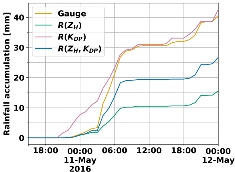
Figure 4. 1-hour rainfall cumulative accumulations from Verolengo gauge, located at 29 km from the radar, and co-located Bric della Croce radar QPE. Z_H not corrected for attenuation.
