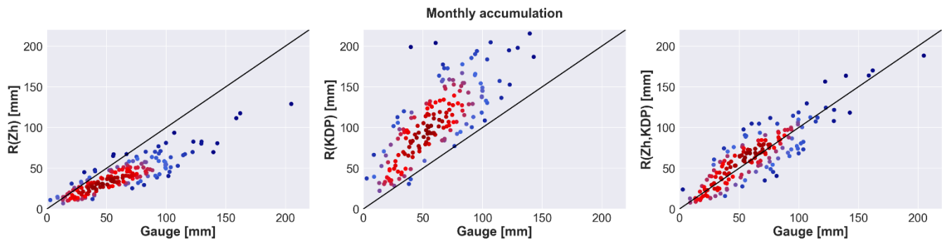
415 Figure 9. Estonia monthly accumulations 2011-2018. The corresponding verification measures are presented in Table 7. The number of radar-gauge data pairs with 8 gauges is 179. Z_H not corrected for attenuation.
