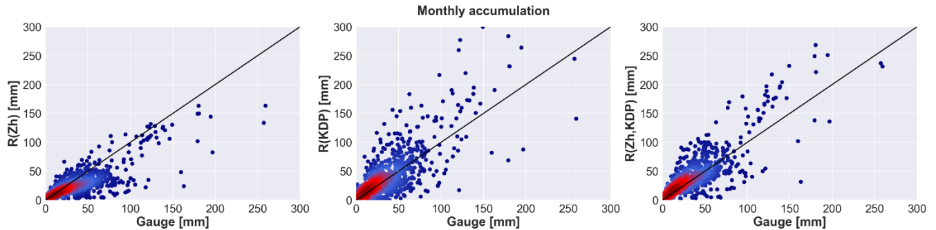
430 Figure 10. Italy monthly accumulations 2012-2016. The corresponding verification measures are presented in Table 8. The number of radar-gauge data pairs with 42 gauges is 675. Z_H not corrected for attenuation.
