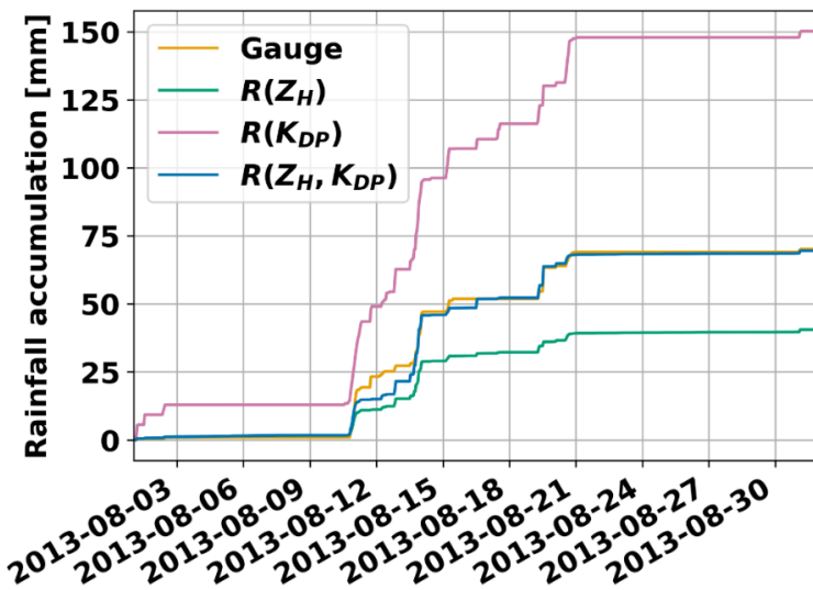
265 Figure 2. One month 1-hour rainfall cumulative accumulations, Sürgavere radar data, Jõgeva station gauge data. Z_H not corrected for attenuation.
