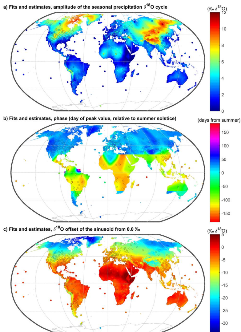
Figure 6. Maps of fitted station values (markers) and the residual-adjusted maps of sine-curve parameters (shaded) that describe the seasonal cycles in precipitation \delta^{18}\text{O} : a) amplitude, b) phase, and c) offset. The interpolated surface is the sum of the infilled surfaces in Figures 3 and 4 (see Methods).
