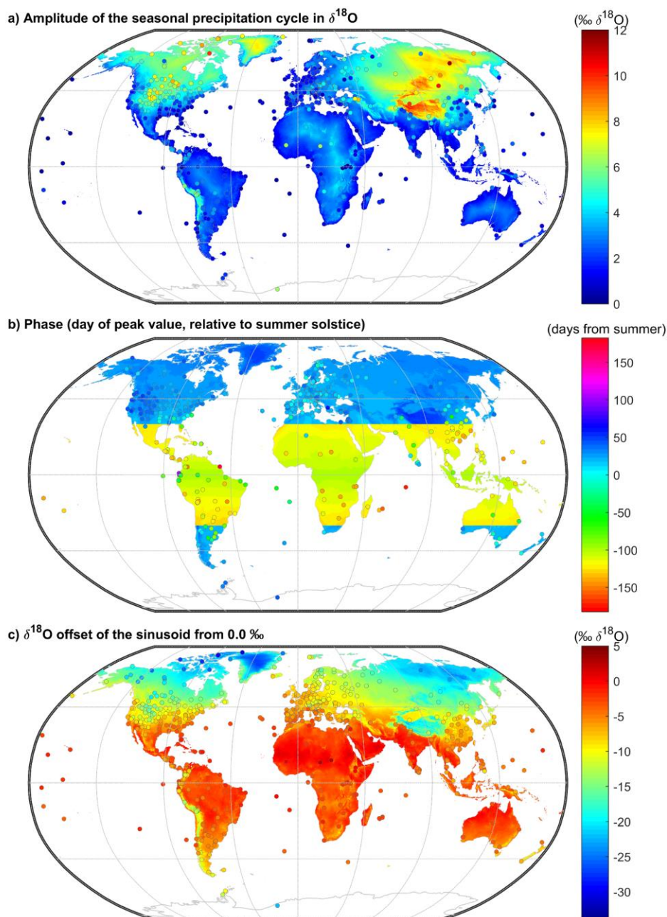
Figure 3. Maps of fitted station values (markers) and regression-based sine-curve parameters (shaded) that describe the seasonal cycles in precipitation \delta^{18}\text{O} a) amplitude, b) phase, and c) offset. The shading reflects multiple-regression models based on landscape characteristics, described in Table 2; for phase, separate models were used in absolute latitudes > 30^\circ versus latitudes < 30^\circ (see methods). Here, residuals were not yet added back into the model.
