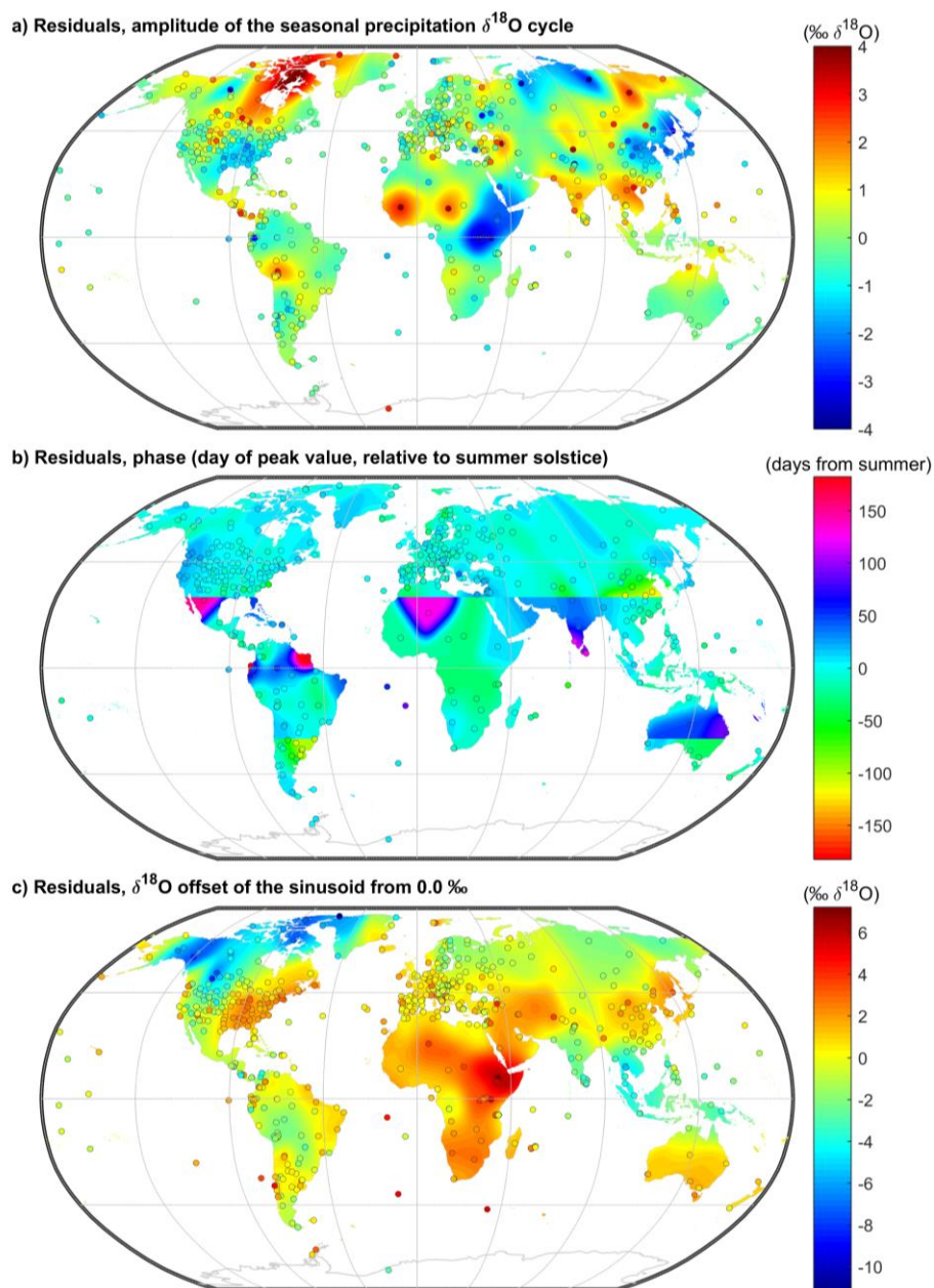
Figure 4. Maps of \delta^{18}\text{O} a) amplitude, b) phase, and c) offset residuals, where the sine parameter values predicted from the multiple regression equations (shown in the interpolated maps in Figure 3) were subtracted from those of parameter values fitted to measurements at each precipitation isotope monitoring site (also shown in Figure 3). The shading shows the smoothed residual layers (see Methods).
