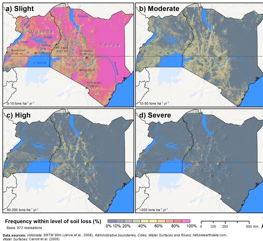
Figure 4. Frequency of USLE model ensemble members to predict one of the four soil loss classes slight ( 0 - 10 \text{ tons ha}^{-1} \text{ yr}^{-1} ) (a), moderate ( 10 - 50 \text{ tons ha}^{-1} \text{ yr}^{-1} ) (b), high ( 50 - 200 \text{ tons ha}^{-1} \text{ yr}^{-1} ) (c), and severe ( >200 \text{ tons ha}^{-1} \text{ yr}^{-1} ) (d), based on the soil loss classification after FAO-PNUMA-UNESCO (1980). The pixel color illustrates the percentage of models from the model ensemble that calculated a soil loss in between the respective class boundaries.
