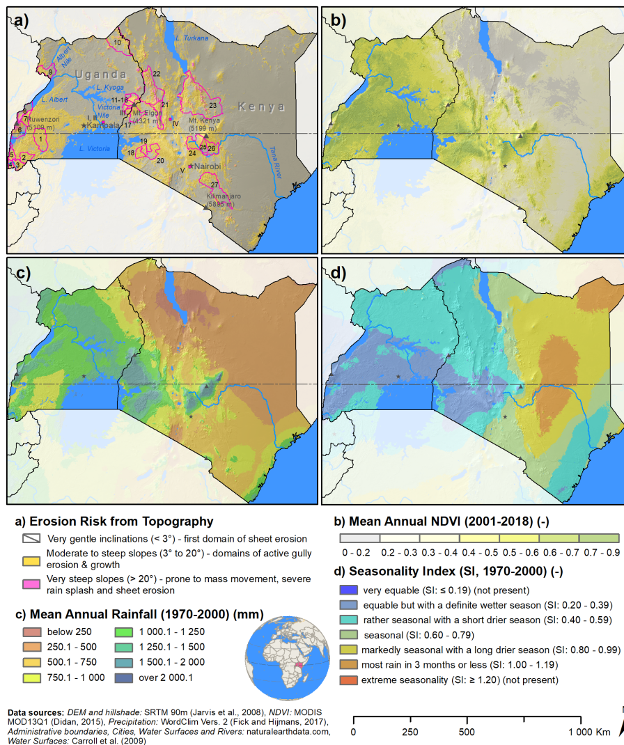
Figure 1. Study area of Kenya and Uganda. A classification of the soil erosion risk after Ebisemiju (1988) (a), the mean annual MODIS NDVI as a proxy for vegetation cover (b), mean annual rainfall (c), and the rainfall seasonality index (SI, Walsh and Lawler, 1981) (d) are plotted to characterize spatial properties of the study region. The boundaries for administrative units where the mean soil loss was assessed are shown with pink outlines in panel a). Locations of soil loss assessments from previous studies that were used for comparison are shown as pink squares. The hillshade is plotted in grey in the background to characterize the terrain topography.
