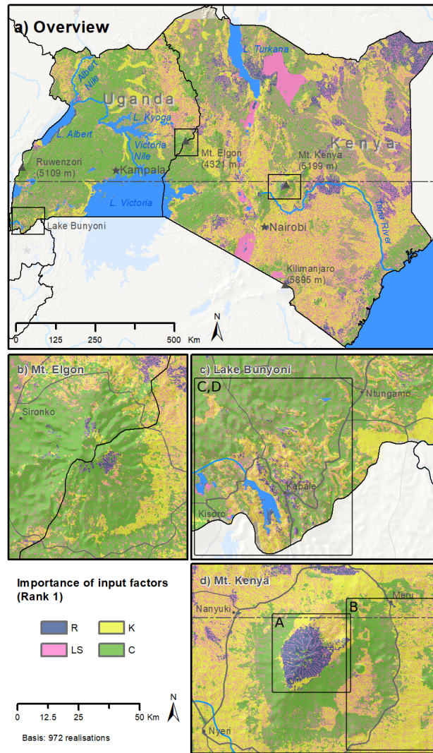
Figure 6. Most important USLE model input factors for the calculation of the soil loss A . The colours blue, yellow, pink, and green indicate whether the input factors R , K , LS , or C caused the largest range in the calculation of A in a grid cell. Panel a) shows the study area of Kenya and Uganda. The panels b), c), and d) show critical erosion hot spots around Mt. Elgon, Lake Bunyoni, and Mt. Kenya, respectively. The insets A) to D) indicate the extents for which the input factor realizations for R , K , LS , and C were analyzed in Fig. 7.
