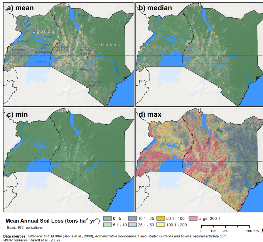
Figure 3. Descriptive statistics calculated for each grid cell based on the 972 USLE model realizations. Panels a) to d) show the mean, median, minimum, and maximum long-term annual soil erosion in each grid cell.
