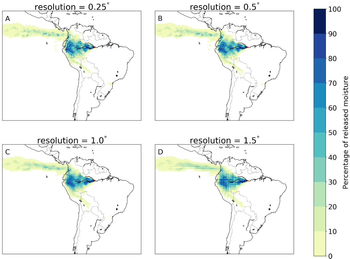
730 Figure 8: Different footprints of moisture releases from Manaus in July 2012 in a three-dimensional Lagrangian model with different horizontal resolutions. A) 0.25^\circ , with a mean latitudinal moisture flow of 1.5^\circ in northerly direction and mean longitudinal flow of 14.4^\circ in westerly direction; B) 0.5^\circ , with a mean latitudinal moisture flow of 1.6^\circ in northerly direction and mean longitudinal flow of 14.3^\circ in westerly direction; C) 1.0^\circ , with a mean latitudinal moisture flow of 1.7^\circ in northerly direction and mean longitudinal flow of 14.2^\circ in westerly direction; D) 1.5^\circ , with a mean latitudinal moisture flow of 1.7^\circ in northerly direction and mean longitudinal flow of 14.2^\circ in westerly direction.
