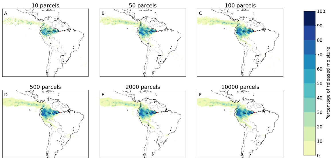
Figure 4: Different footprints of moisture releases from Manaus in July 2012 in a three-dimensional Lagrangian model with 10, 50, 100, 500, 2,000, and 10,000 tracked parcels \text{mm}^{-1} . A) 10 parcels, with a mean latitudinal moisture flow of 1.3^\circ in northerly direction and mean longitudinal flow of 14.2^\circ in westerly direction; B) 50 parcels, with a mean latitudinal moisture flow of 1.6^\circ in northerly direction and mean longitudinal flow of 14.3^\circ in westerly direction; C) 100 parcels, with a mean latitudinal moisture flow of 1.4^\circ in northerly direction and mean longitudinal flow of 14.2^\circ in westerly direction; D) 500 parcels, with a mean latitudinal moisture flow of 1.4^\circ in northerly direction and mean longitudinal flow of 14.3^\circ in westerly direction; E) 2,000 parcels, with a mean latitudinal moisture flow of 1.5^\circ in northerly direction and mean longitudinal flow of 14.4^\circ in westerly direction; F) 10,000 parcels, with a mean latitudinal moisture flow of 1.5^\circ in northerly direction and mean longitudinal flow of 14.3^\circ in westerly direction.
