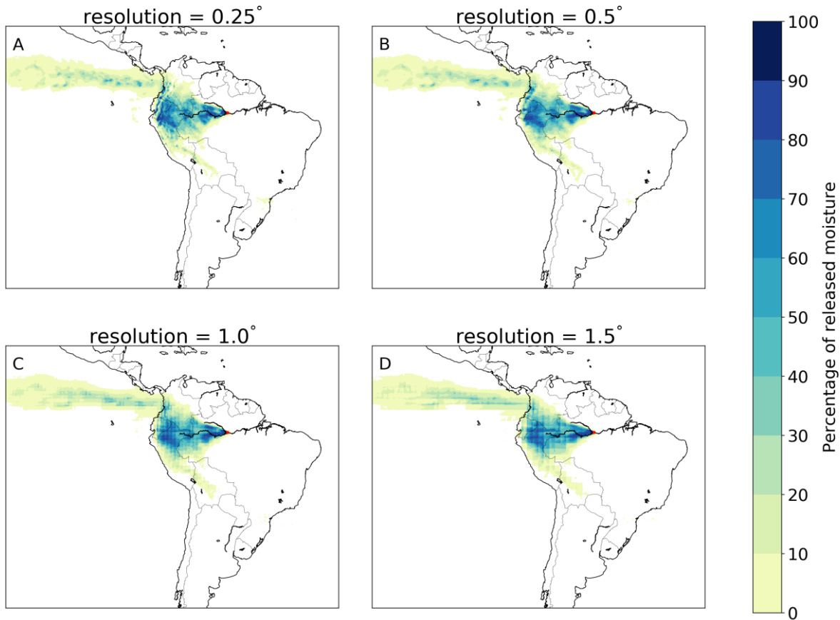
695 Figure 8: Different footprints of moisture releases from Manaus in July 2012 in a three-dimensional Lagrangian model with different horizontal resolutions. A) 0.25^\circ , with a mean latitudinal moisture flow of 1.5^\circ in northerly direction and mean longitudinal flow of 14.4^\circ in westerly direction; B) 0.5^\circ , with a mean latitudinal moisture flow of 1.6^\circ in northerly direction and mean longitudinal flow of 14.3^\circ in westerly direction; C) 1.0^\circ , with a mean latitudinal moisture flow of 1.7^\circ in northerly direction and mean longitudinal flow of 14.2^\circ in westerly direction; D) 1.5^\circ , with a mean latitudinal moisture flow of 1.7^\circ in northerly direction and mean longitudinal flow of 14.2^\circ in westerly direction.
