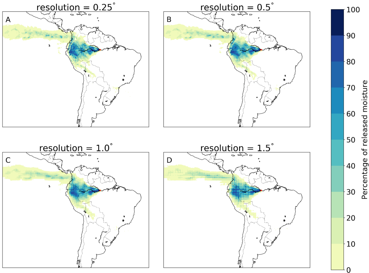
730 Figure 8: Different footprints of moisture releases from Manaus in July 2012 in a three-dimensional Lagrangian model with different horizontal resolutions. A) 0.25°, with a mean latitudinal moisture flow of 1.5° in northerly direction and mean longitudinal flow of 14.4° in westerly direction; B) 0.5°, with a mean latitudinal moisture flow of 1.6° in northerly direction and mean longitudinal flow of 14.3° in westerly direction; C) 1.0°, with a mean latitudinal moisture flow of 1.7° in northerly direction and mean longitudinal flow of 14.2° in westerly direction; D) 1.5°, with a mean latitudinal moisture flow of 1.7° in northerly direction and mean longitudinal flow of 14.2° in westerly direction.
