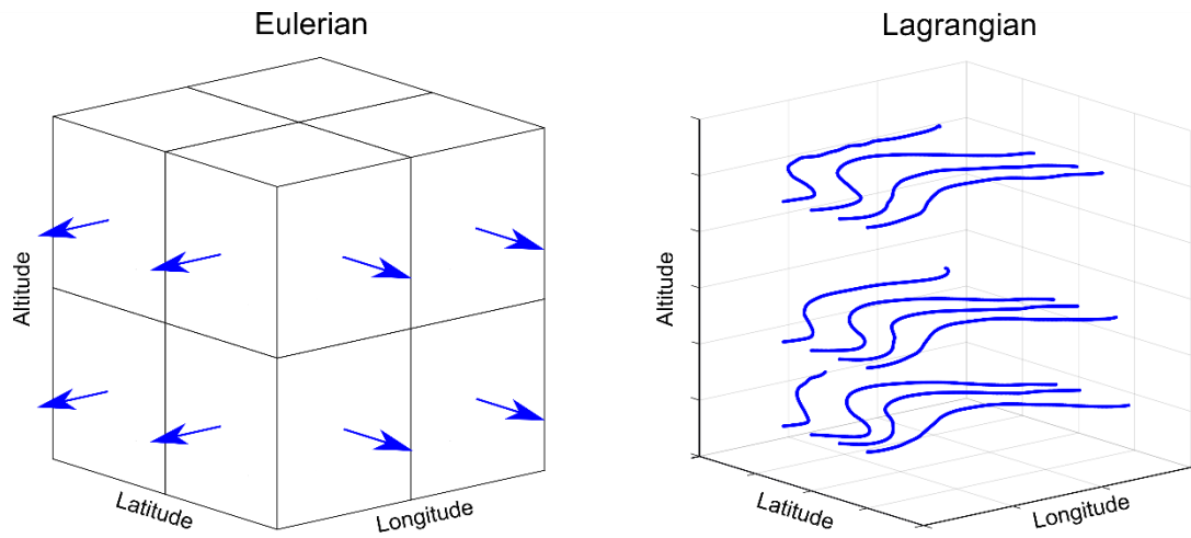
675 Figure 2: The difference between Eulerian and Lagrangian moisture tracking models. A) Eulerian models are grid- based, meaning that the study area is divided into a two- or three-dimensional grid of cells. At each time step, the tracked moisture content of each grid cell is updated based on estimated cell-to-cell winds, precipitation, and evaporation. B) Lagrangian models are trajectory-based, meaning that a number of moisture parcels have coordinates. At each time step, the coordinates and the tracked moisture content of the parcels are updated based on point-based 680 wind flows, precipitation, and evaporation.
