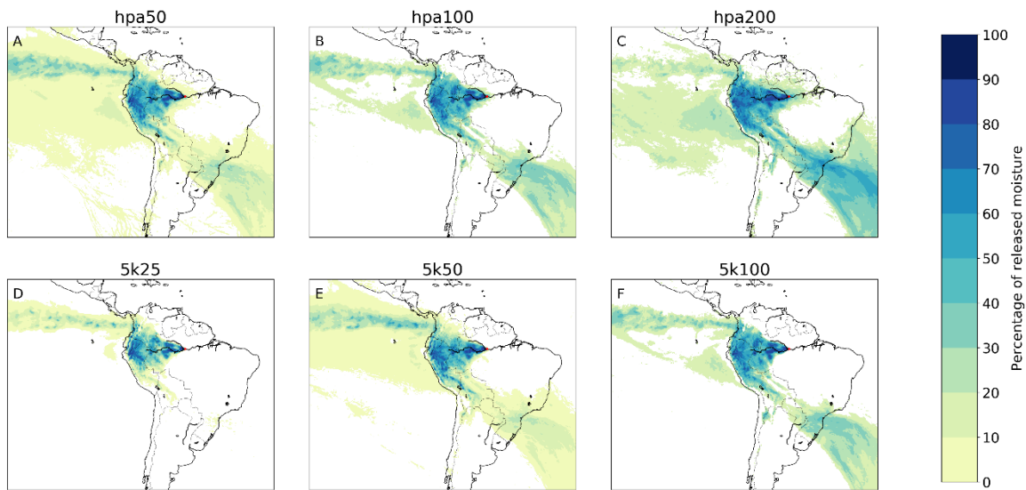
720 Figure 7: Different footprints of moisture releases from Manaus in July 2012 in a three-dimensional Lagrangian model with different degradations of the vertical moisture profile. A) hpa50, with a mean latitudinal moisture flow of 2.8^\circ in southerly direction and mean longitudinal flow of 11.0^\circ in westerly direction; B) hpa100, with a mean latitudinal moisture flow of 5.3^\circ in southerly direction and mean longitudinal flow of 9.2^\circ in westerly direction; C) hpa200, with a mean latitudinal moisture flow of 17.6^\circ in southerly direction and mean longitudinal flow of 1.8^\circ in westerly direction; D) 5k25, with a mean latitudinal moisture flow of 1.7^\circ in northerly direction and mean longitudinal flow of 14.4^\circ in westerly direction; E) 5k50, with a mean latitudinal moisture flow of 2.8^\circ in southerly direction and mean longitudinal flow of 11.6^\circ in westerly direction; F) 5k100, with a mean latitudinal moisture flow of 5.1^\circ in southerly direction and mean longitudinal flow of 9.6^\circ in westerly direction. 725
