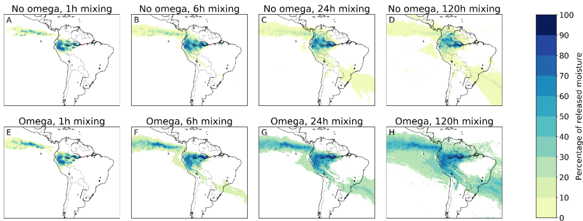
730 Figure 10: Different footprints of moisture releases from Manaus in July 2012 in a three-dimensional Lagrangian model with different mixing assumptions: without and with accounting for the three-dimensional moisture flows in the ERA5 data (termed omega), and with different assumptions of additional vertical mixing speed (full mixing every 1 h, every 6 h, every 24 h, and every 120 h). A) Without omega, every 1 h mixing, with a mean latitudinal moisture flow of 2.4^\circ in northerly direction and mean longitudinal flow of 16.4^\circ in westerly direction; B) Without omega, every 6 h mixing, with a mean latitudinal moisture flow of 1.4^\circ in northerly direction and mean longitudinal flow of 14.3^\circ in westerly direction; C) Without omega, every 24 h mixing, with a mean latitudinal moisture flow of 0.1^\circ in northerly direction and mean longitudinal flow of 11.6^\circ in westerly direction; D) Without omega, every 120 h mixing, with a mean latitudinal moisture flow of 1.2^\circ in northerly direction and mean longitudinal flow of 9.0^\circ in westerly direction; E) With omega, every 1 h mixing, with a mean latitudinal moisture flow of 3.0^\circ in northerly direction and mean longitudinal flow of 16.7^\circ in westerly direction; F) With omega, every 6 h mixing, with a mean latitudinal moisture flow of 0.3^\circ in northerly direction and mean longitudinal flow of 14.5^\circ in westerly direction; G) With omega, every 24 h mixing, with a mean latitudinal moisture flow of 5.0^\circ in northerly direction and mean longitudinal flow of 12.3^\circ in westerly direction; H) With omega, every 120 h mixing, with a mean latitudinal moisture flow of 6.9^\circ in northerly direction and mean longitudinal flow of 11.5^\circ in westerly direction.
