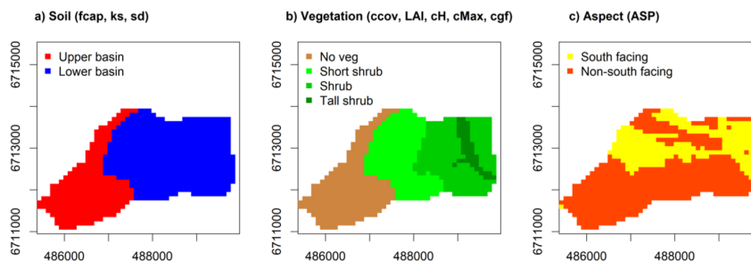
Figure 3. Aggregation used to set the spatially variable parameters: a) soil classification for two calibrated parameters ( fcap = volumetric field capacity, ks = recession coefficient) and one fixed parameter ( sd = soil depth); b) vegetation classification for 5 fixed parameters ( ccov =canopy coverage, LAI = leaf area index, cH = canopy height, cMax = maximum canopy storage and cgf = canopy gap fraction); c) aspect classification for ASP parameter that was calibrated if south-facing or set to 1 for any non-south-facing aspect.
