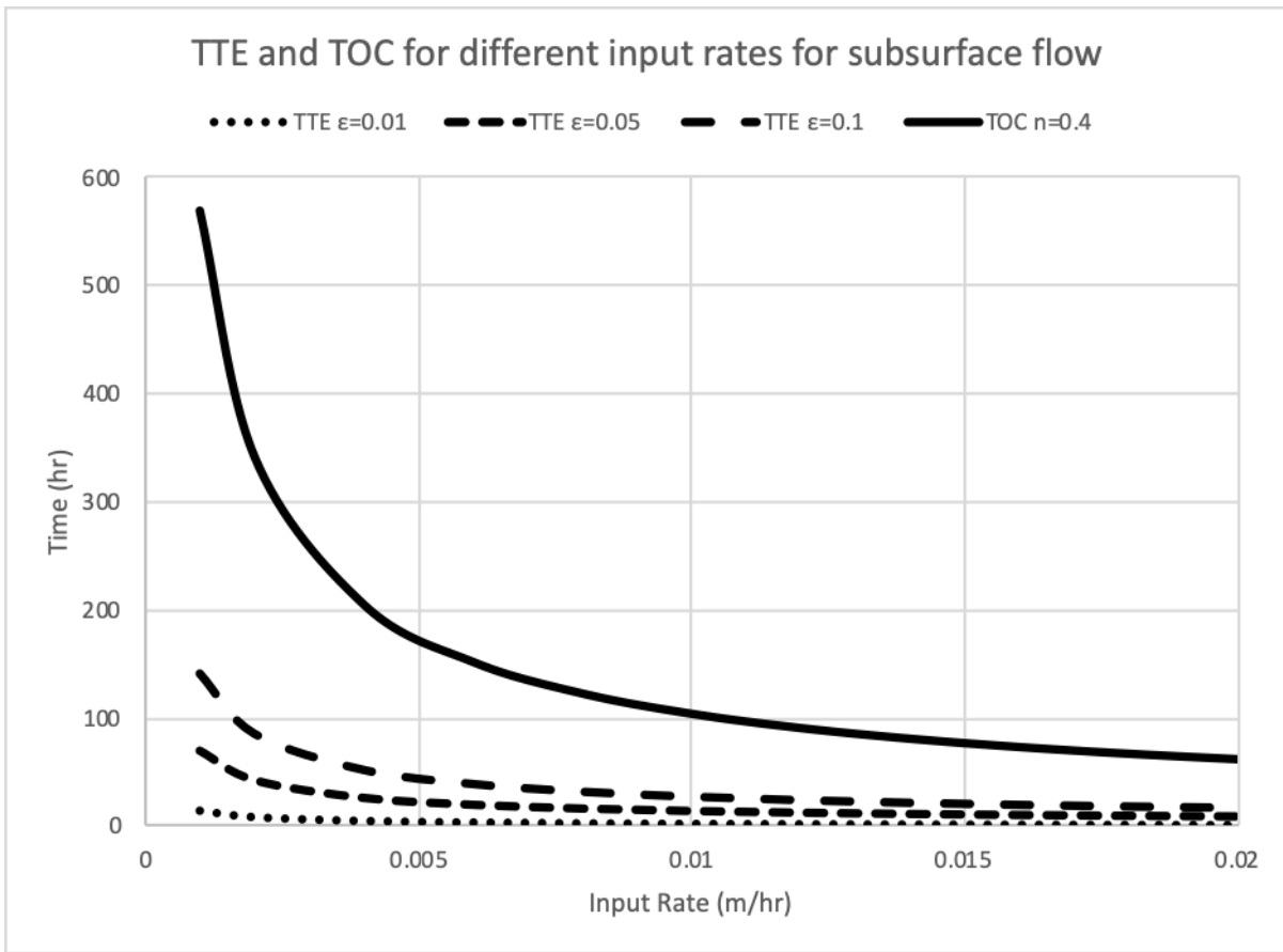
Figure A1. Time of Concentration (TOC solid line) and Time to Equilibrium (TTE dashed lines) for subsurface flow on a hillslope of 100m for different input rates and values of effective porosity (TOC is constant for each input rate) ( K_o = 2 m/hr, \sin \beta = 0.05 ) (Equations [A7] and [A8]).
