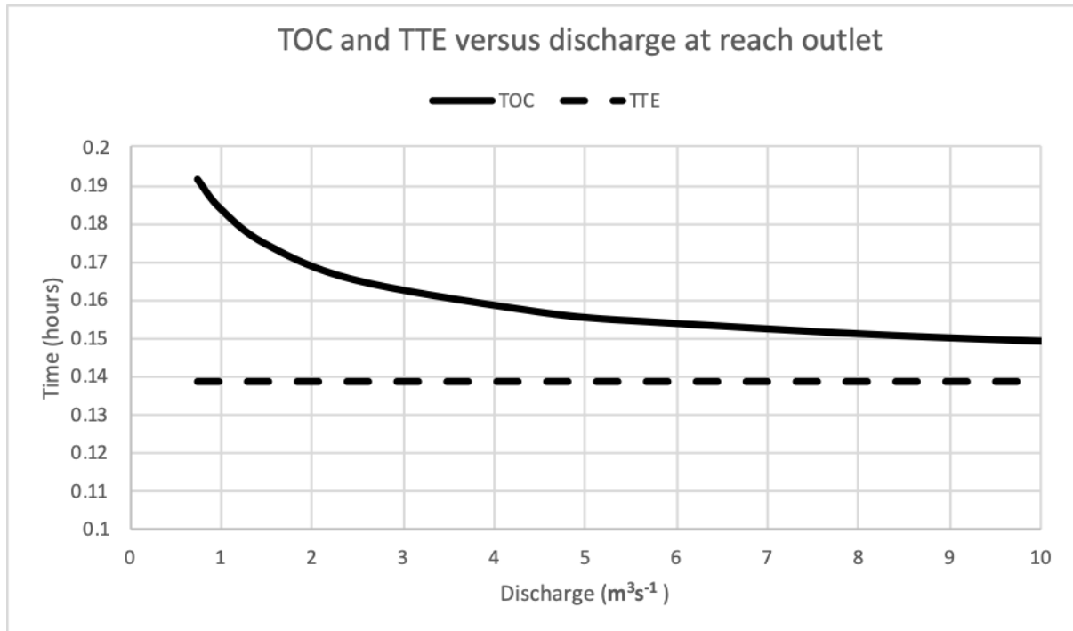
670 Figure A3. Time of Concentration (solid line) and Time to Equilibrium (dashed line) for an upland channel reach of 500m, with parameters from Beven (1979) ( a = 1 \text{ m/s} ; k = 0.233 \text{ m}^3\text{s}^{-1} ). Upstream discharge 0.5 \text{ m}^3\text{s}^{-1} ; lateral inflows from 0.0005 to 0.02 \text{ m}^2\text{s}^{-1} (Equations [A20] and [A21])
