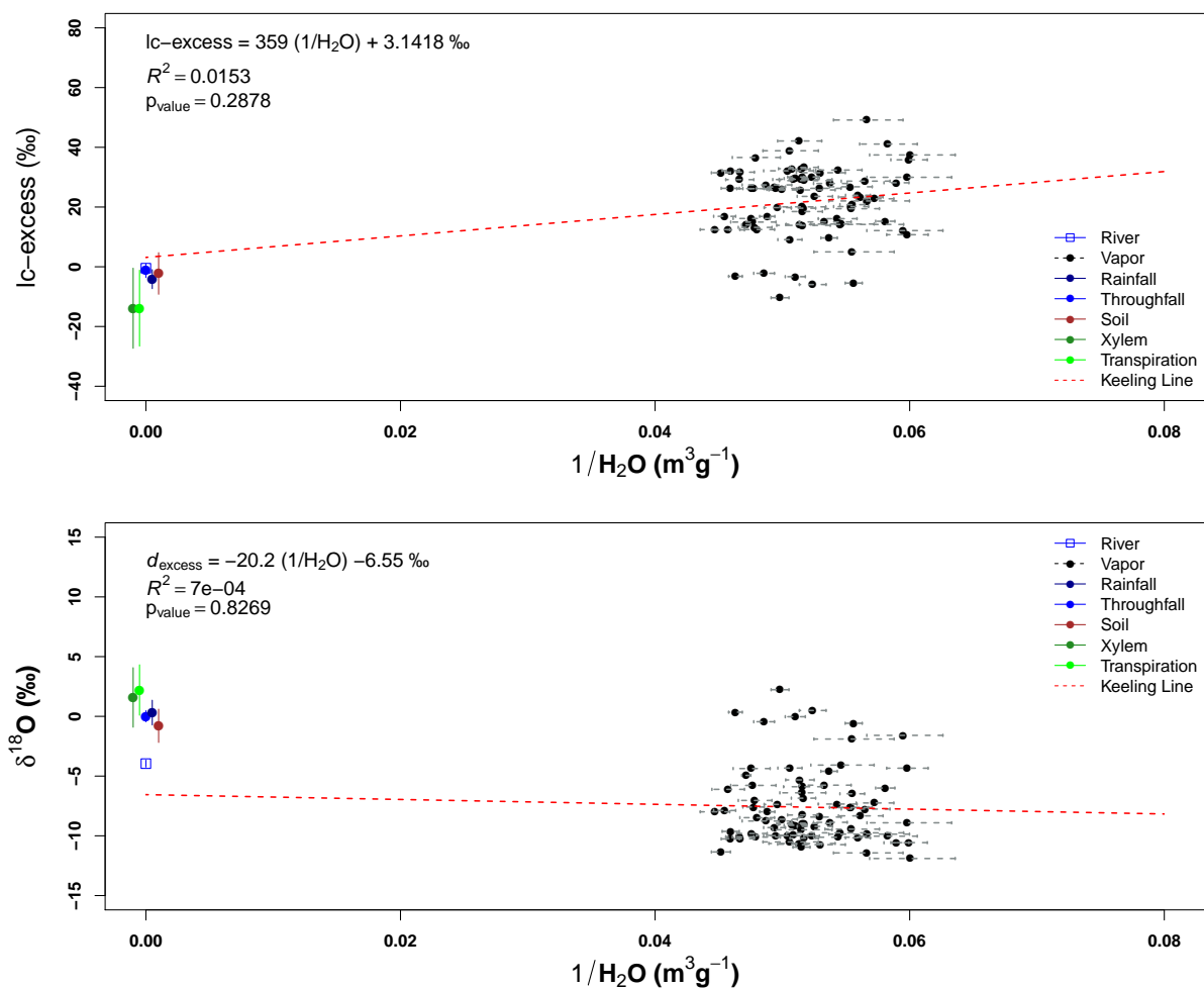
Figure II. Line-conditioned excess ( lc\text{-excess} ) and oxygen-18 ( \delta^{18}\text{O} ) mixing relationships ("Keeling plots") for the monitoring period. Air samples collected at 43 m and 22 m height. The standard deviation of each air sample shows the variation of the absolute humidity of the air ( \rho_v ) for each sampling. NOTE: THIS IMAGE WAS UPDATED
