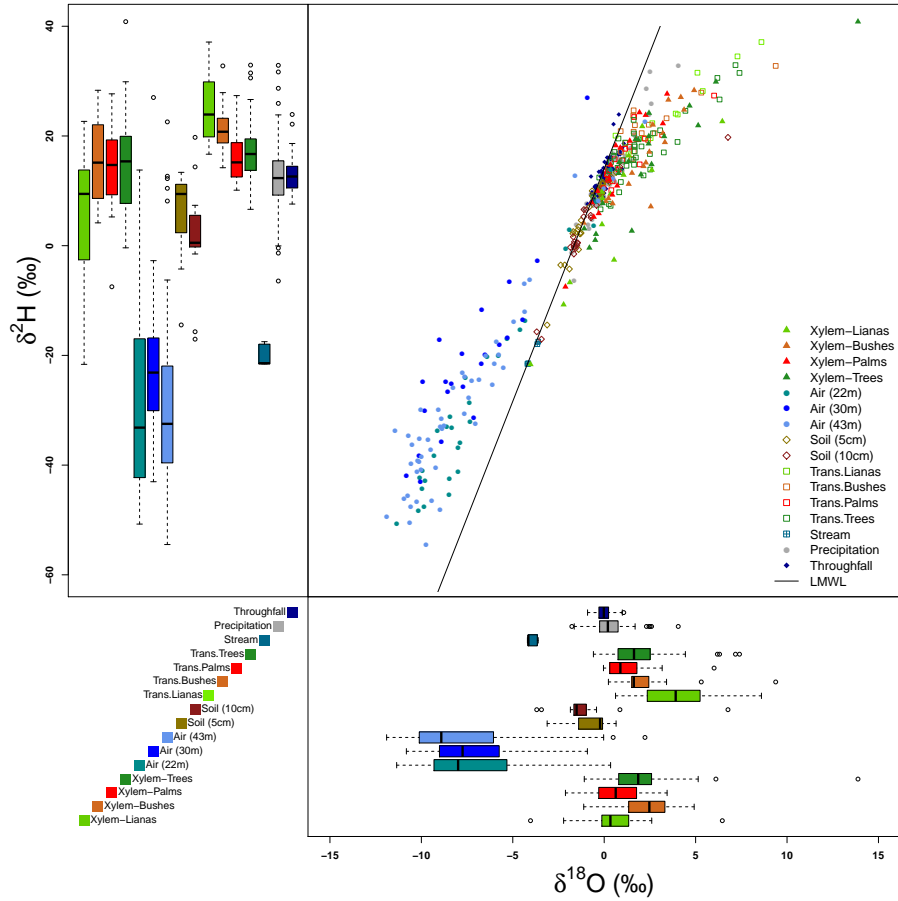
Figure 6. Isotopic signatures of \delta^2H and \delta^{18}O of all the samples collected at the MRI-plot. Dual isotope plot shows the relationship among the local meteoric water line (LMWL) and all the samples. The box plots of \delta^2H (upper-left) and \delta^{18}O (bottom-right) show the distribution of isotope signatures per sample type.
