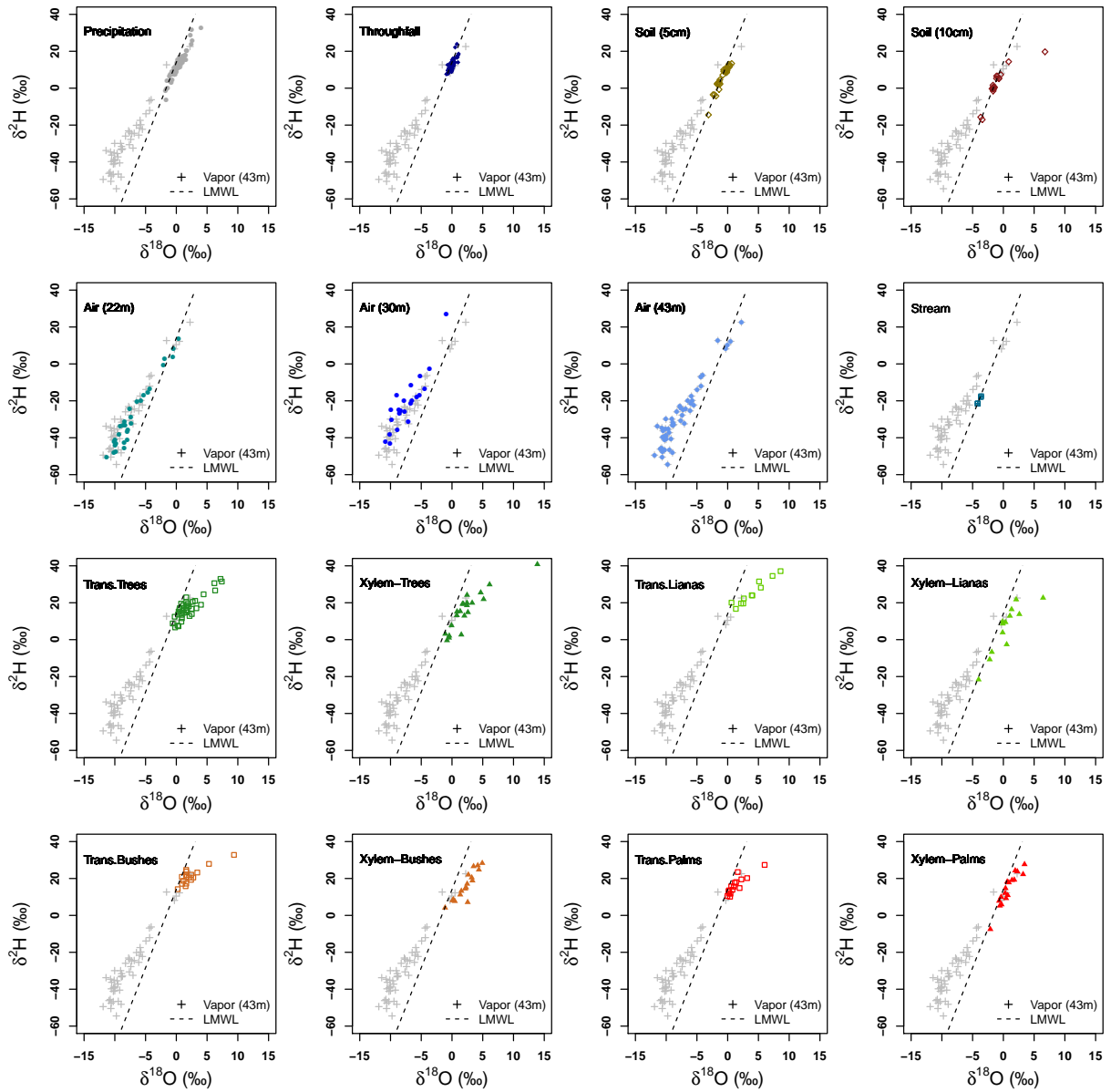
Figure 7. Dual isotope plots of \delta^2H and \delta^{18}O per sample type collected at La Selva Biological Station. Vapor samples collected at 43 m height and local meteoric water line (LMWL) are used in each plot as references.
