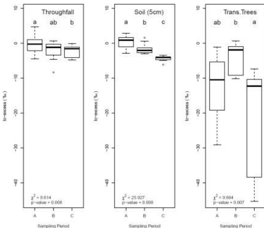
140 Figure 8. Box plots showing the temporal differences in Ic-excess for throughfall, soil water at 5 cm depth, and trees transpiration while the other sample types did not showed significant differences ( p=0.05 ). Sampling periods with the same lower case character per sample type do not differ ( p = 0.05 ).
