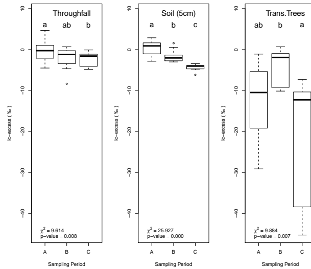
Figure 8. Box plots showing the temporal differences in lc\text{-excess} for throughfall, soil water at 5 cm depth, and trees transpiration. The other sample types did not showed significant differences ( p=0.05 ). Sampling periods with the same lower case character per sample type do not differ ( p=0.05 ).
