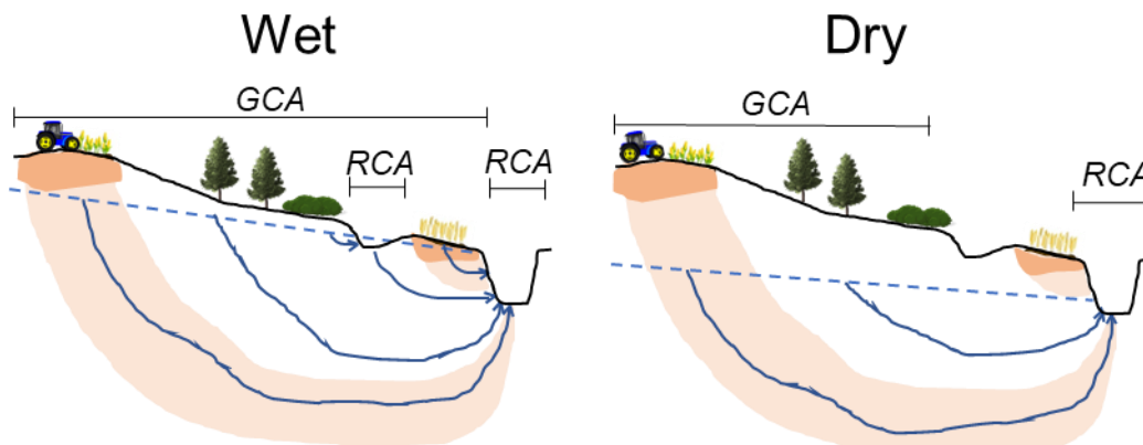
1015 Figure 10. Contributing areas fluctuate with wetness conditions due to changing flow paths. GCA is the Groundwater Contributing Area which is where discharge was infiltrated and RCA is the Runoff Contributing Area which is where discharge is generated. Areas between the two different contributing areas are 'inactive' and do not actively influence stream discharge.
