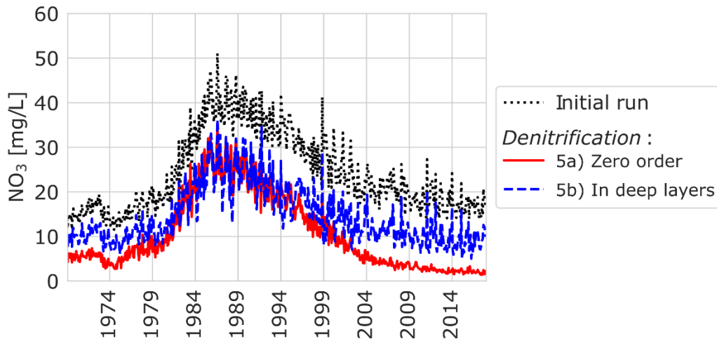
995 Figure 7. Effect of denitrification for the upstream part of the catchment using different conceptualizations: zero order denitrification (5a) and denitrification in deep layers (5b).
