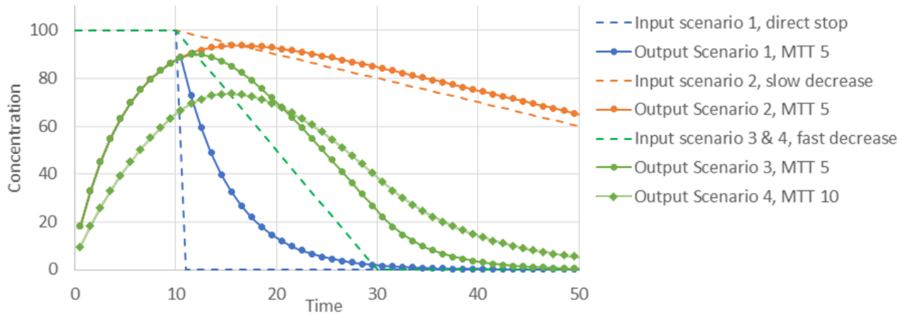
1000 Figure 8. Output concentrations for a hypothetical catchment with an exponential TTD and a MTT of 5 or 10, following three input scenarios: a direct stop of the input, a slow decrease in the input (decrease 1% of maximum per timestep) and a fast decrease of the input (decrease 5% of max per timestep).
