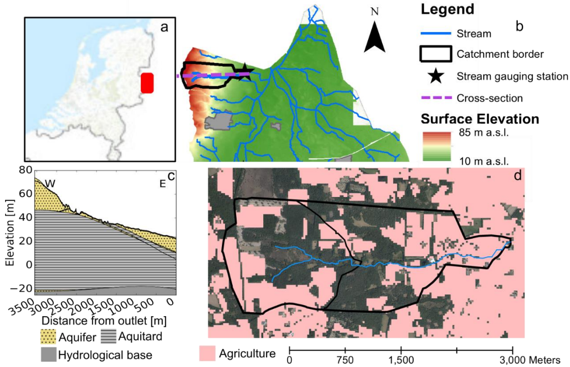
960 Figure 1: Location of the study area (a, b), model conceptualization (c), and the location of agricultural fields in the year 2007 (d). Background maps and DEM from PDOK ( PDOK.nl/datasets ).
