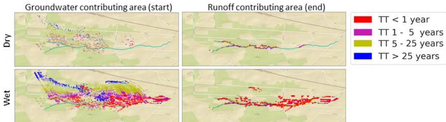
1010 Figure 9. Contributing area in the model for a dry (top; summer 2006) and a wet (bottom; winter 2006/2007) period. Colors represent the travel time towards the stream with blue TT >25 year and red TT < 1 year (similar to Figure 2). Notice the large increase in the runoff contributing area in the downstream part of the catchment during wet periods which results from the extensive agricultural drainage system. Background map ESRI StreetMap World 2D, Sources: Esri, DeLorme, NAVTEQ, USGS, NRCAN, METI, iPC, TomTom, http://services.arcgisonline.com/ArcGIS/rest/services/ESRI_StreetMap_World_2D/MapServer .
