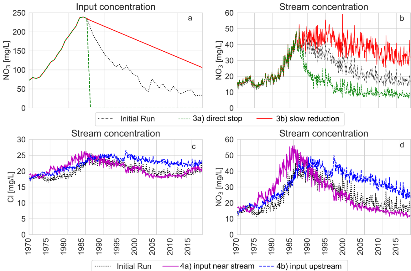
Figure 6. Panel a and b show the effect of two scenarios with changes in the nitrate input for the upstream of the catchment. Note the difference in scale of the y-axis between the left and right panels. Panels c and d show the effect of spatial changes in land-use on both chloride (c) and nitrate (d): only agriculture inside of a 200 m strip around the stream (4a), and only agriculture outside of the
