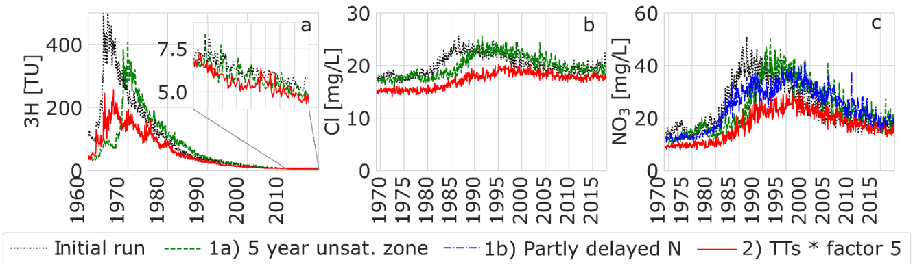
Figure 5. The effect on tritium (a), chloride (b) and nitrate (c) in the upstream part of the catchment of a scenario with a 5-year delay due to an unsaturated zone, a scenario where part of the input of N was delayed and a scenario where all travel times were increased by a factor 5.
