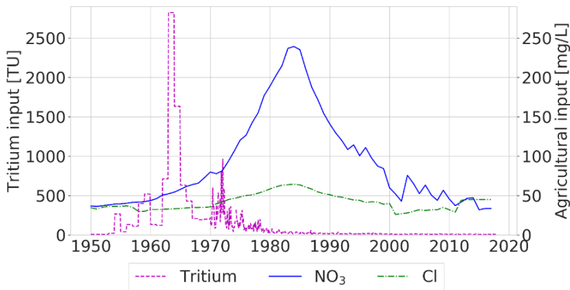
Figure 2. Input time series for tritium (left axis) and the estimated concentrations of nitrate and chloride under farmland (right axis). The tritium input time series is based on precipitation measurements at stations Vienna and Ottawa (before 1970) and Groningen and Emmerich (from 1970). The 1985 peak in chloride and nitrate coincides with the start of the legislations from the Dutch Manure Law that placed restrictions on the applications of N in agriculture.
