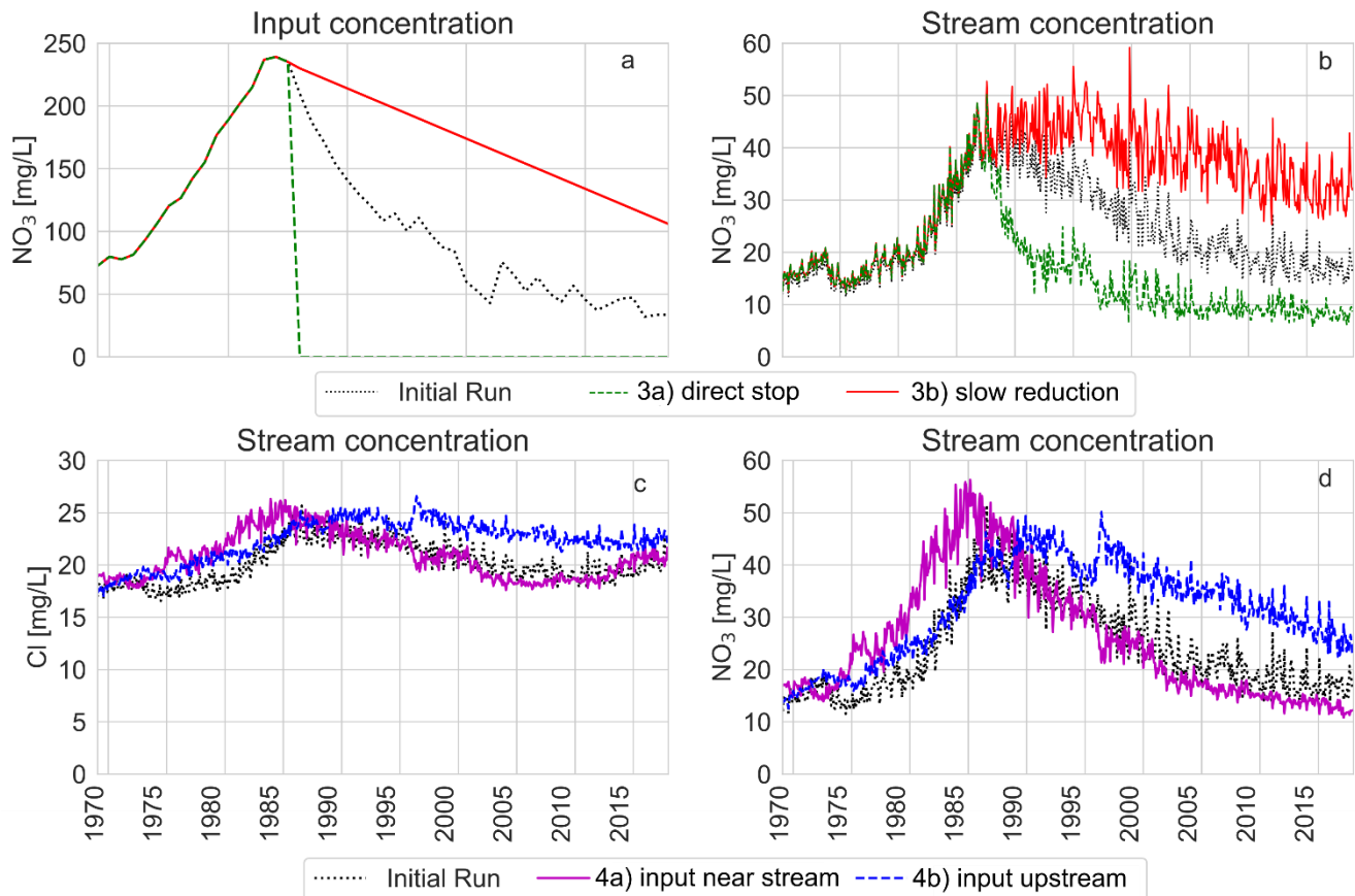
1055 Figure 6. Panel a and b show the effect of two scenarios with changes in the nitrate input for the upstream of the catchment. Note the difference in scale of the y-axis between the left and right panels. Panels c and d show the effect of spatial changes in land-use on both chloride (c) and nitrate (d): only agriculture inside of a 200 m strip around the stream (4a), and only agriculture outside of the same buffer strip (4b). In both scenarios agricultural parts have 50% agriculture and 50% nature, so that the total fraction of fields is approximately equal to that in the real catchment.
