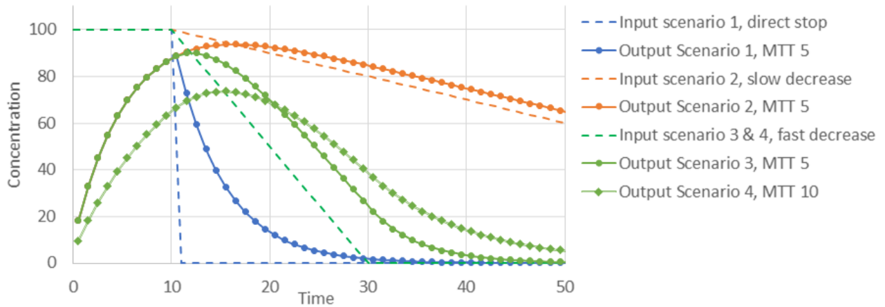
Figure 8. Output concentrations for a hypothetical catchment with an exponential TTD and a MTT of 5 or 10, following three input scenarios: a direct stop of the input, a slow decrease in the input (decrease 1% of maximum per timestep) and a fast decrease of the input (decrease 5% of max per timestep).
