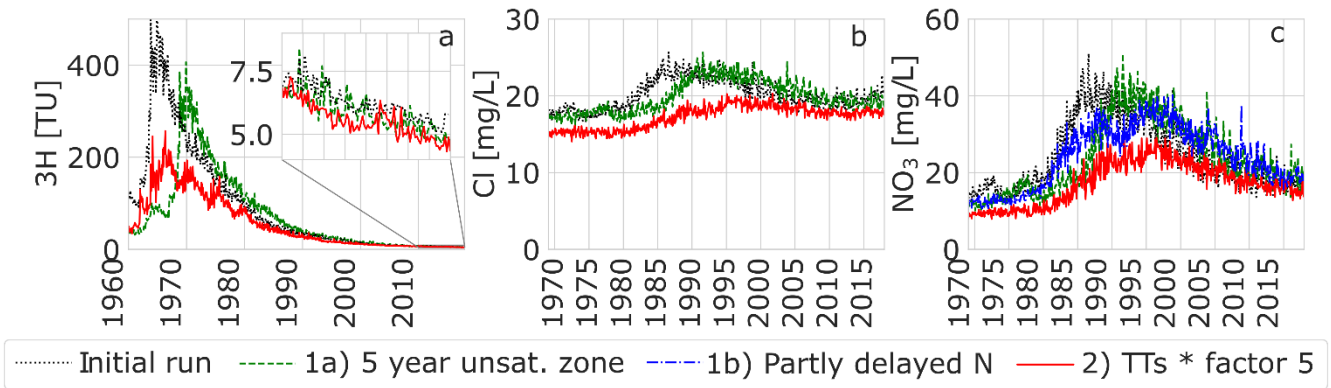
1050 Figure 5. The effect on tritium (a), chloride (b) and nitrate (c) in the upstream part of the catchment of a scenario with a 5-year delay due to an unsaturated zone, a scenario where part of the input of N was delayed and a scenario where all travel times were increased by a factor 5.
