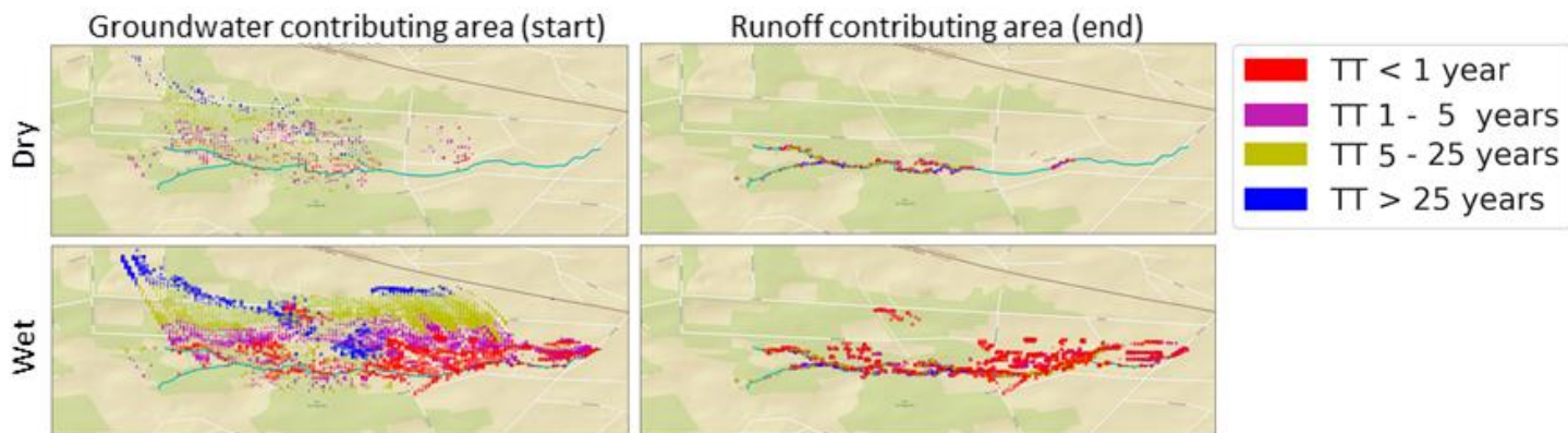
Figure 9. Contributing area in the model for a dry (top; summer 2006) and a wet (bottom; winter 2006/2007) period. Colors represent the travel time towards the stream with blue TT >25 year and red TT < 1 year (similar to Figure 3figure 2). Notice the large increase in the runoff contributing area in the downstream part of the catchment during wet periods which results from the extensive agricultural drainage system. Background map ESRI_StreetMap_World_2D, Sources: Esri, DeLorme, NAVTEQ, USGS, NRCAN, METI, iPC, TomTom, http://services.arcgisonline.com/ArcGIS/rest/services/ESRI_StreetMap_World_2D/MapServer .
