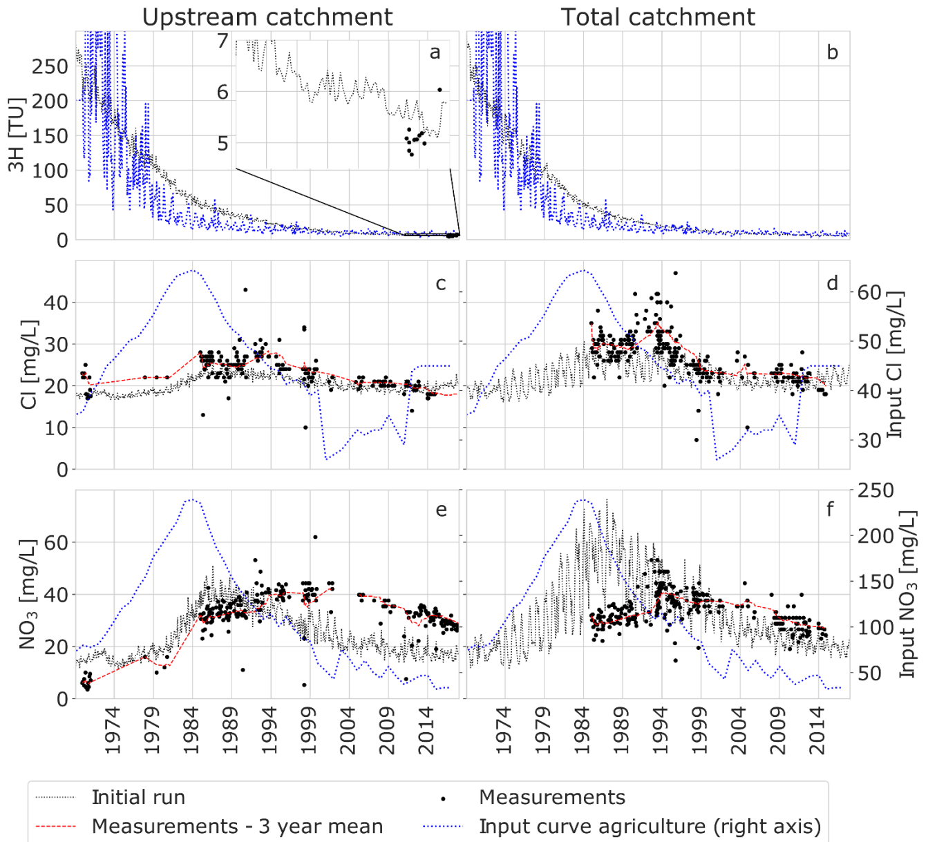
Figure 4. Measurements, agricultural input time series and initial model results based on the TTDs from Kaandorp, et al. (2018) and the solute input time series in Figure 2 Figure 3 . On the left tritium (a), chloride (c) and nitrate (e) for the upstream part of the catchment, on the right tritium (b), chloride (d) and nitrate (f) for the total catchment (downstream). No further processes were added. Note that tritium samples were only available for the upstream part of the catchment (panel a).
