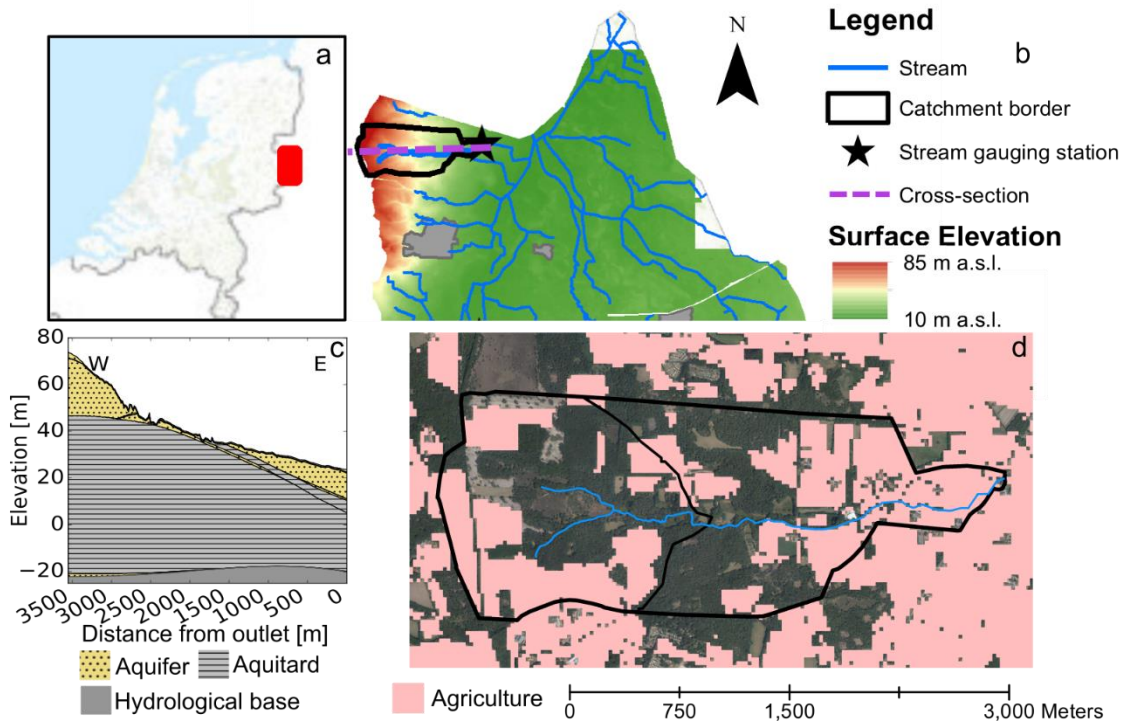
Figure 1: Location of the study area (a, b), model conceptualization (c), and the location of agricultural fields in the year 2007-19 (d). Background maps and DEM from PDOK ( PDOK.nl/datasets ).
