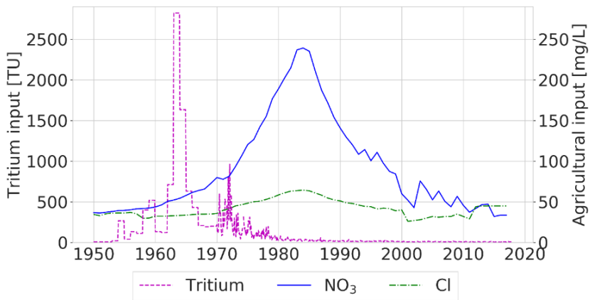
Figure 3. Input time series for tritium (left axis) and the estimated concentrations of nitrate and chloride under farmland (right axis). The tritium input time series is based on precipitation measurements at stations Vienna and Ottawa (before 1970) and Groningen and Emmerich (from 1970). The 1985 peak in chloride and nitrate coincides with the start of the legislations from the Dutch Manure Law that placed restrictions on the applications of N in agriculture.
