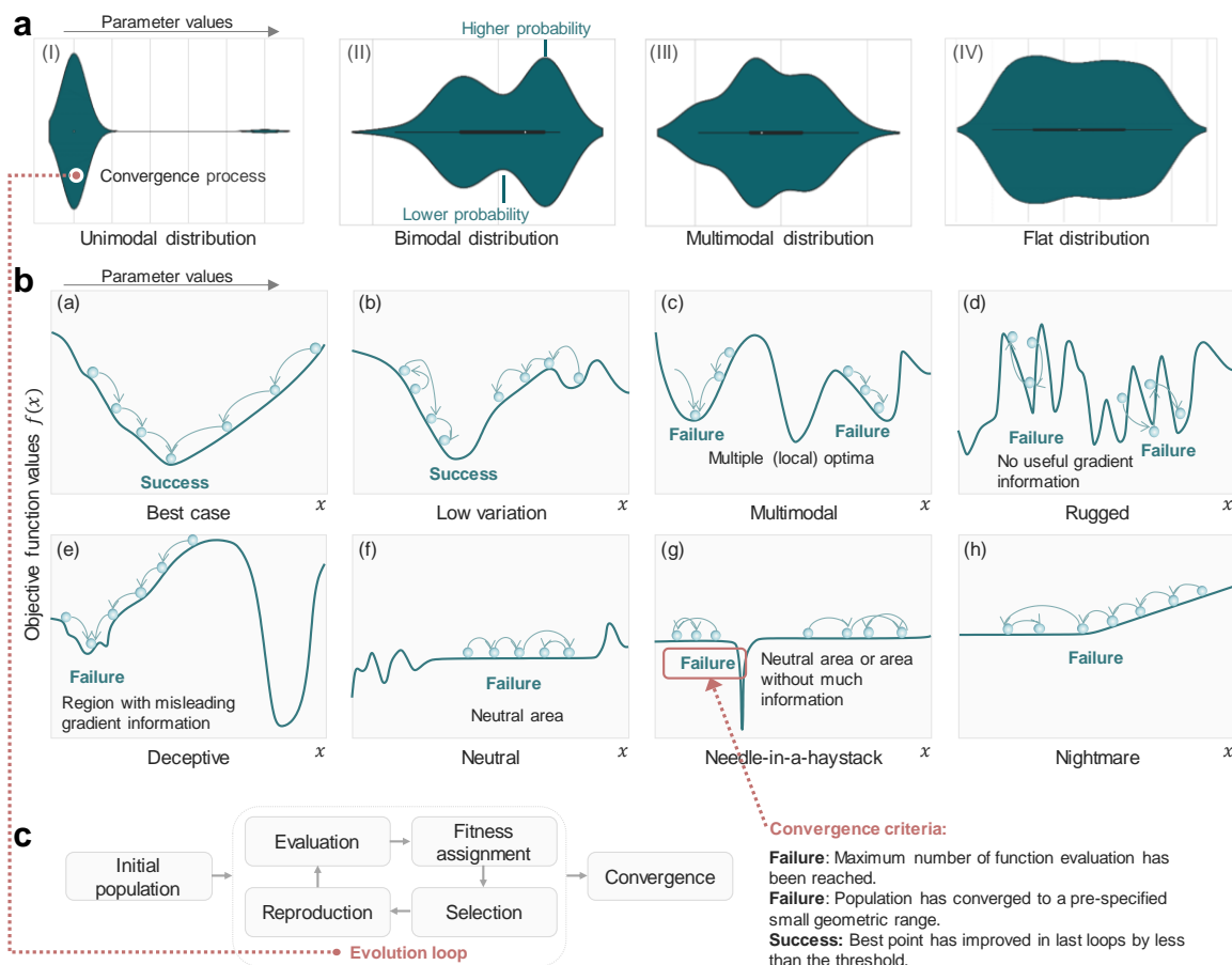
Figure 7: Evaluation of the ability of the dynamic parameters to respond to the catchment dynamics. a , Evaluation of the convergence
