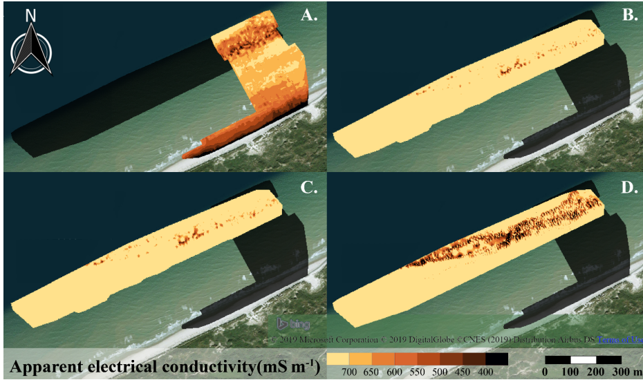
Figure 4: FDEM data. A. rECa (CMD-MiniExplorer) using CMD3, with a pseudodepth approximately 1.8 m (23 February 2018); B., C., and D. rECa (DUALEM-421S) using respectively the HCP1, PRP4, and HCP4 configurations, providing pseudodepths of 1.5, 2, and 6 m (27-28 September 2018). Note that another colour scale is used compared to the other figures. Copyright: Microsoft Corporation, DigitalGlobe, and CNES, 2019.
