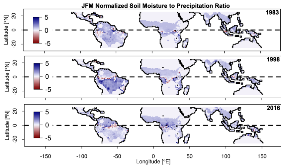
Figure 7b: Same as Figure 7a but for January to March in 1983 (top), 1998 (middle) and 2016 (bottom).
