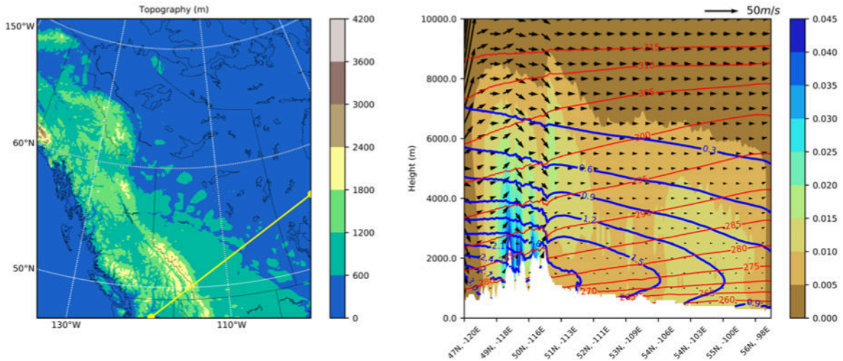
Figure 7. Topography (m) in Western Canada. (b) Cross-section of potential temperature (K, thin red contour), water vapor mixing ratio ( \text{g kg}^{-1} , thick blue contour), the sum of snow, ice and graupel mixing ratio ( \text{g kg}^{-1} , shading), and winds ( \text{m s}^{-1} ) perpendicular to the Canadian Rockies at 115^{\circ}\text{W} , 50^{\circ}\text{N} in December. The vertical component of winds is scaled by 100 for illustration purposes.
