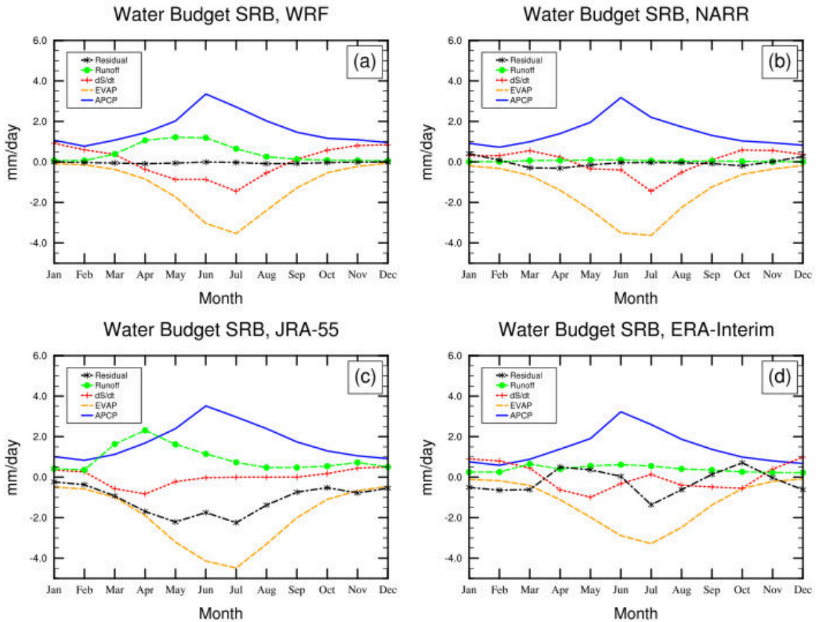
Figure 3. The surface water budget ( \text{mm day}^{-1} ) in SRB from WRF-CTL and the reanalysis datasets: NARR, ERA-Interim, JRA-55. EVAP denotes evapotranspiration. ACP denotes accumulated precipitation per time interval.
