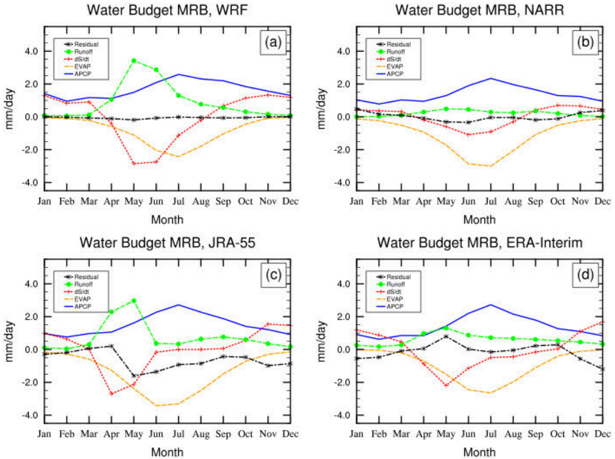
Figure 2. The surface water budget ( \text{mm day}^{-1} ) in MRB from WRF-CTL and the reanalysis datasets: NARR, ERA-Interim, JRA-55. EVAP denotes evapotranspiration. ACP denotes accumulated precipitation per time interval.
