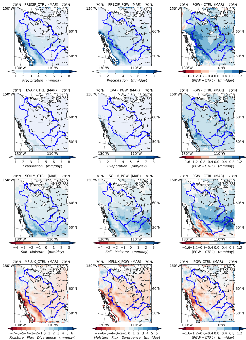
Figure 9. P, ET, changes in soil moisture, and divergence of vertically integrated moisture flux for WRF-CTL (left), WRF-PGW (middle), and differences between WRF-CTL and WRF-PGW (right) in March. The unit of all variables is turned into \text{mm day}^{-1} , which makes it easy for comparisons among variables. All variables are averaged over the simulation period over the calendar month.
