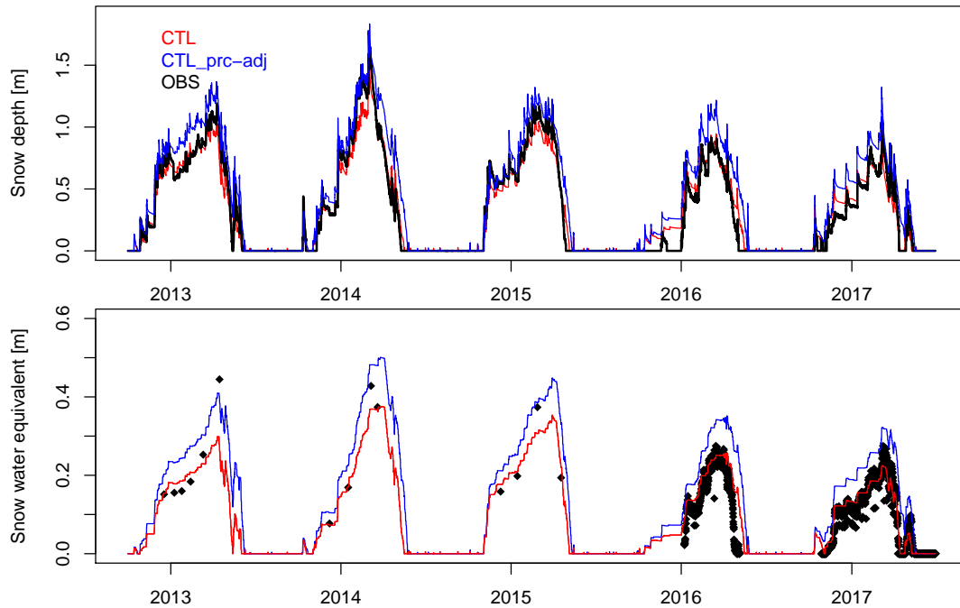
Figure A2. Snow depth (upper panel) and snow water equivalent (lower panel) simulated by the SNOWPACK model when the adjusted total precipitation forcing is employed (CTL_prc-adj) compared to the control run (CTL) and observations.
