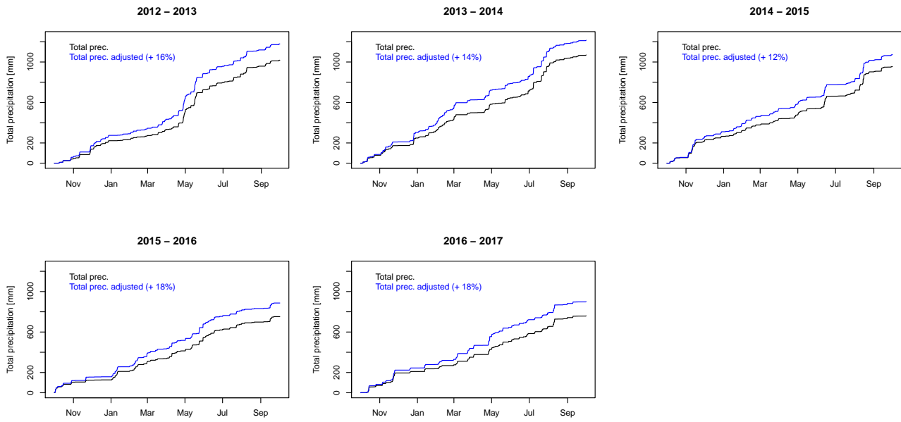
Figure A1. Cumulated total precipitation at the Torgnon site measured by the OTT Pluvio2 precipitation gauge (black) compared to the precipitation adjusted with the method of Kochendorfer et al. (2017a) for the five snow seasons considered (blue).
