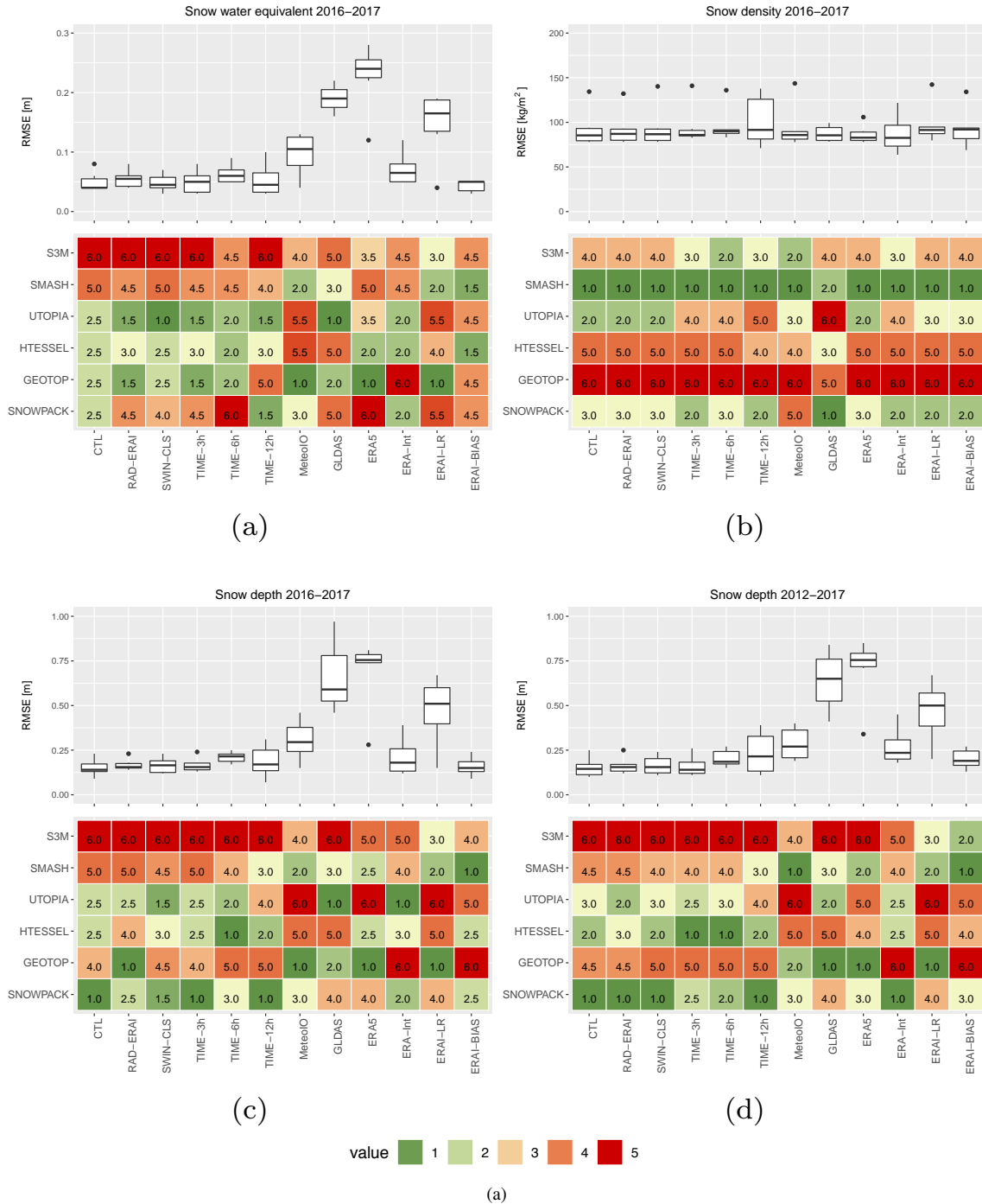
Figure 6. Root Mean Square Error associated to a) snow water equivalent, b) snow density and c) snow depth simulations for each experiment and each model over the period 2016-2017. Panel d) shows the same statistics as c) but on the whole period 2012-2017. Upper panels represent the boxplot statistics, lower panels represent the model rank (1=best model, 5=worst model).
