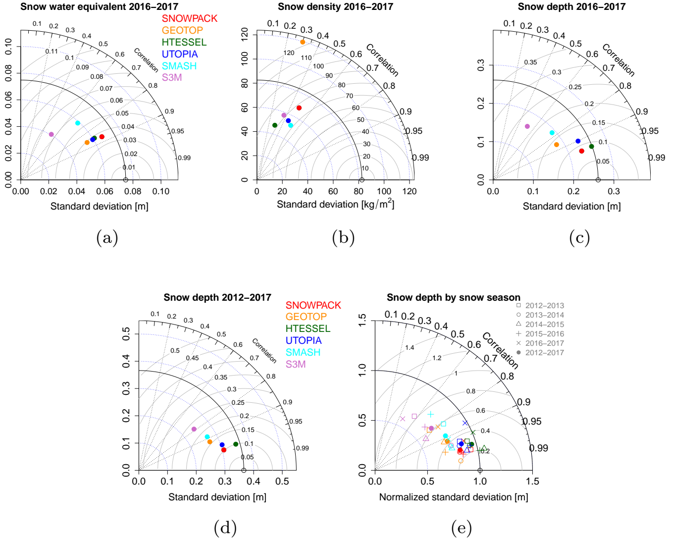
Figure 2. Taylor diagrams of the modeled vs. observed a) snow water equivalent, b) snow density and c) snow depth in the control experiment (CTL) for the period 2016-01-01 to 2017-06-30. Bottom panels represent the statistics of snow depth d) for the whole period 2012-2017 and e) for each snow season in the same period. Differently from other panels, in panel e) model standard deviations are normalized with respect to the observed ones.
