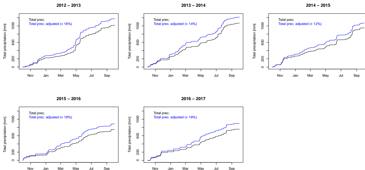
Figure A1. Cumulated total precipitation at the Torgnon site measured by the OTT Pluvio2 precipitation gauge (black) compared to the precipitation adjusted with the Kochendorfer method (blue) for the five snow seasons considered.
