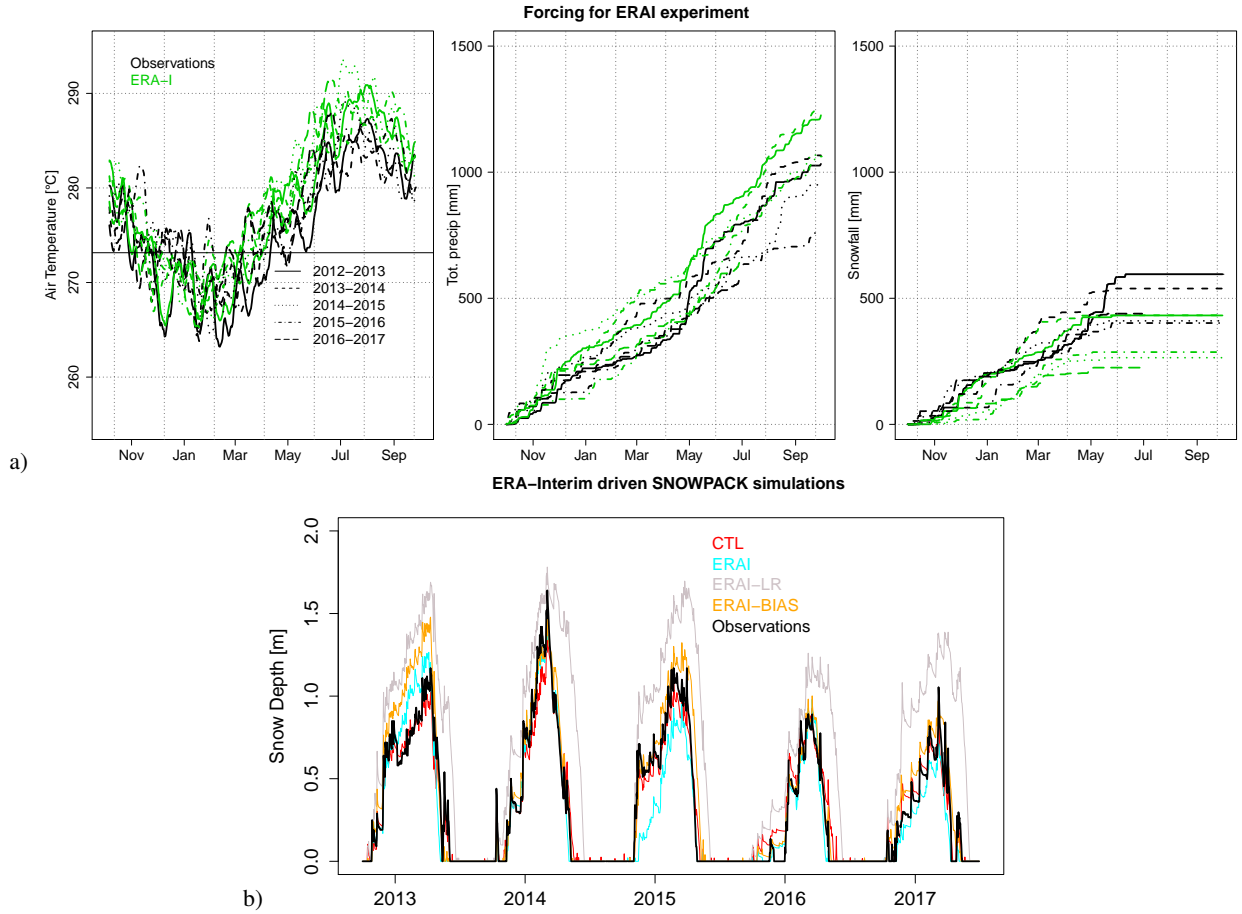
Figure 5. a) ERA-Interim air temperature, total precipitation and snowfall (derived as explained in Sect. 4) at the Torgnon site, compared to the station measurements (black) for each snow season of the period 2012-2017; b) Example of ERA-Interim driven snow depth simulations (ERAI, ERA-LR and ERAI-BIAS experiments), obtained using the SNOWPACK model, compared to CTL run and snow depth observations.
