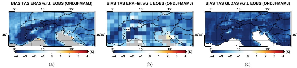
Figure D1. BIAS of ERA5, ERA-Interim and GLDAS air temperatures with respect to EOBS observations over the Greater Alpine Region. Temperatures have been averaged over the months from October to June and over the period 1980-2014 in the case of ERA5 and ERA-Interim, over the period 2000-2014 in the case of GLDAS.
