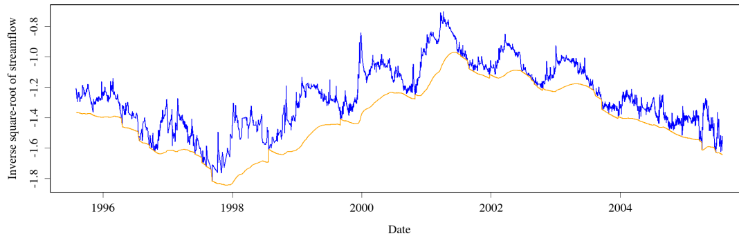
Fig. 3. NISR-transformed separated hydrograph of the Petit Thérain river in Saint-Omer-en-Chaussée
