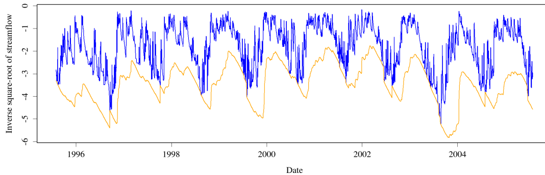
Fig. 1. NISR-transformed separated hydrograph of Vair river in Soullousse-sous-Saint-Élophé
