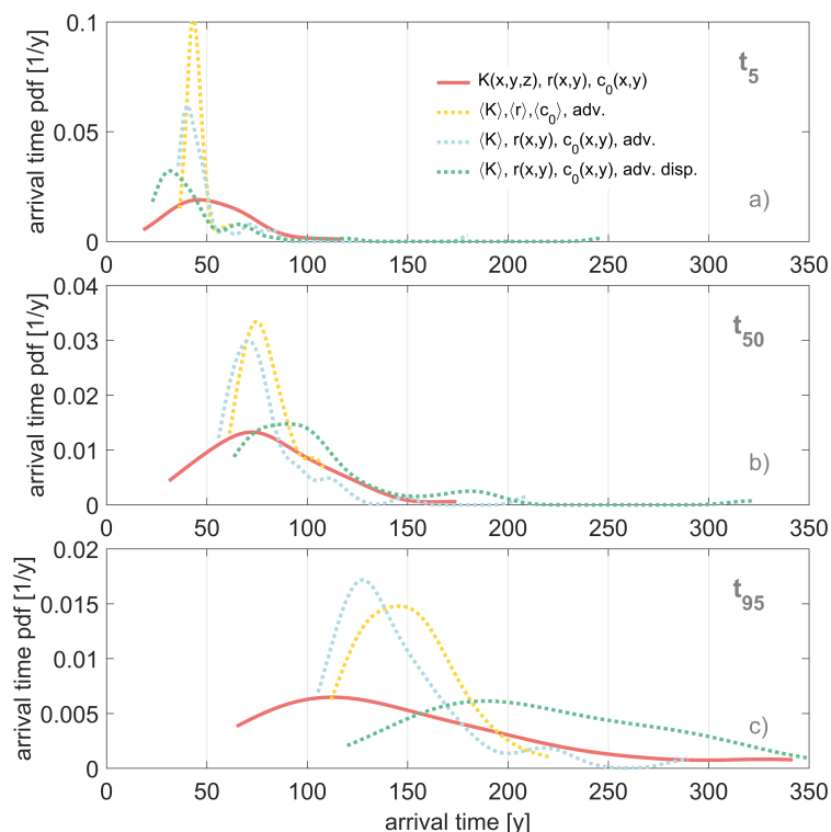
Figure 7. Probability density function of the time required for 5% (a), 50% (b), and 95% (c) of the total recorded mass to reach a well considering a heterogeneous K field, heterogeneous r and heterogeneous c_0 (reference case, red solid line); an upscaled K values, averaged r and averaged c_0 accounting for advection only (yellow dashed line); an upscaled K values, heterogeneous r and heterogeneous c_0 accounting for advection only (blue dashed line); an upscaled K values, heterogeneous r and heterogeneous c_0 accounting for advection and dispersion (green dashed line).
