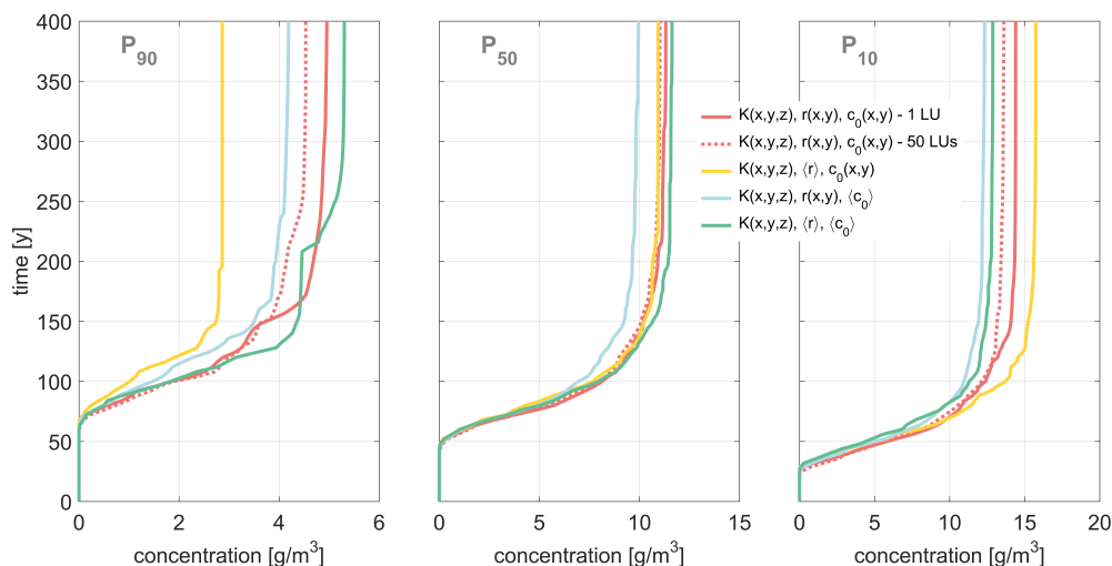
Figure 6. Time ( y -axis) required for a well to exceed a given concentration ( x -axis) with a probability of 90% (left), 50% (middle) and 10% (right) considering a heterogeneous r and heterogeneous c_0 (reference case, red line); a homogeneous r and heterogeneous c_0 (yellow line); a heterogeneous r and homogeneous c_0 (light blue line); a homogeneous r and homogeneous c_0 (green line). For comparison, the red dash lines shows outputs from simulations with a realization-dependent land-use maps.
