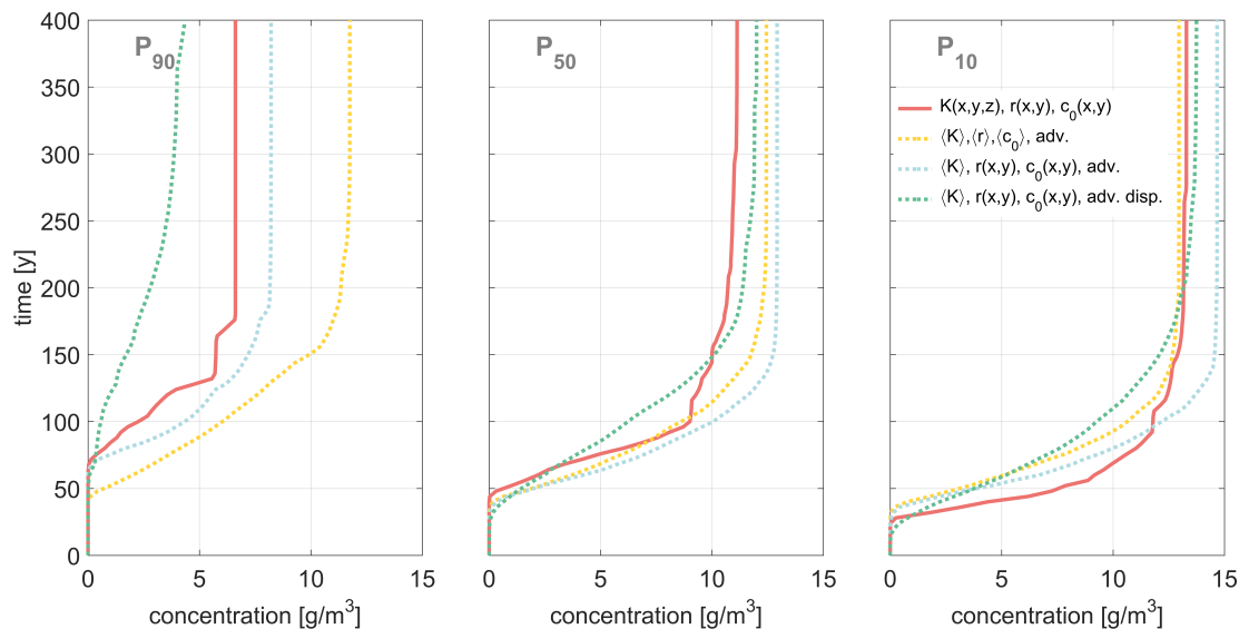
Figure 10. Time ( y -axis) required for a well to exceed a given concentration ( x -axis) with a probability of 90% (left), 50% (middle) and 10% (right) considering a heterogeneous K field, heterogeneous r and heterogeneous c_0 (reference case, red solid line); an upscaled K values, averaged r and averaged c_0 accounting for advection only (yellow dashed line); an upscaled K values, heterogeneous r and heterogeneous c_0 accounting for advection only (blue dashed line); an upscaled K values, heterogeneous r and heterogeneous c_0 accounting for advection and dispersion (green dashed line).
