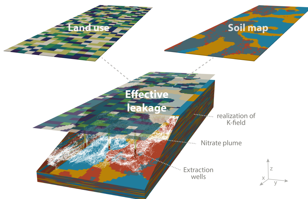
Figure 1. Illustration of the methodology used in the study, considering a representative quadri-lateral subsystem of a highly heterogeneous alluvial aquifer system, 19.2 \times 6 \times 0.25 \text{ km}^3 (12 miles \times 3.75 miles \times 820 feet). A land use map is randomly generated (top-left). Each color represents a different crop. A soil map (top-right) is extracted from the top layer of each geostatistical realization of the hydraulic conductivity ( K ). For each combination soil-type/crop, effective leakage rates of water and nitrate are numerically estimated. White particles represent a snapshot of the NPS pollution (particles) eighty years after a single year of contaminant loading. In each simulation, three extraction wells are explicitly represented at downstream location of the domain. The lower part of each well (in red) represent its screen from where water is extracted and from where mass arrival is recorded. Other wells are implicitly represented by the flux into the lower boundary of the domain.
