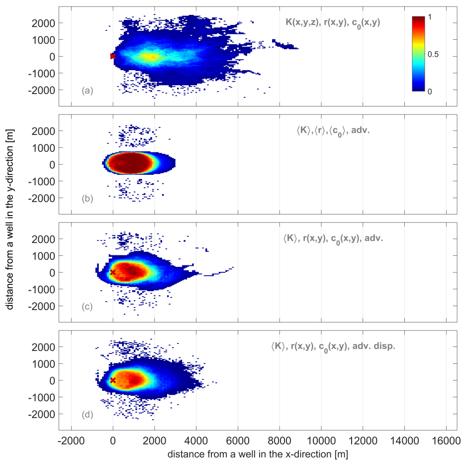
Figure 8. Probability of a particle leaving a given grid-cell to reach a well accounting for a heterogeneous K field, heterogeneous r and heterogeneous c_0 (reference case, a); an upscaled K values, averaged r and averaged c_0 accounting for advection only (b); an upscaled K values, heterogeneous r and heterogeneous c_0 accounting for advection only (c); an upscaled K values, heterogeneous r and heterogeneous c_0 accounting for advection and dispersion (d).
