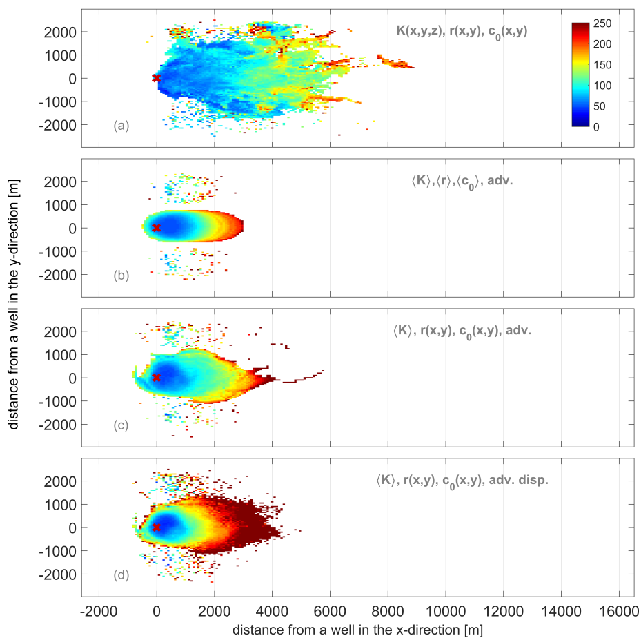
Figure 9. Expected travel time [years] of a particle leaving a given grid-cell and reaching a well for a heterogeneous K field, heterogeneous r and heterogeneous c_0 (reference case, a); an upscaled K values, averaged r and averaged c_0 accounting for advection only (b); an upscaled K values, heterogeneous r and heterogeneous c_0 accounting for advection only (c); an upscaled K values, heterogeneous r and heterogeneous c_0 accounting for advection and dispersion (d).
