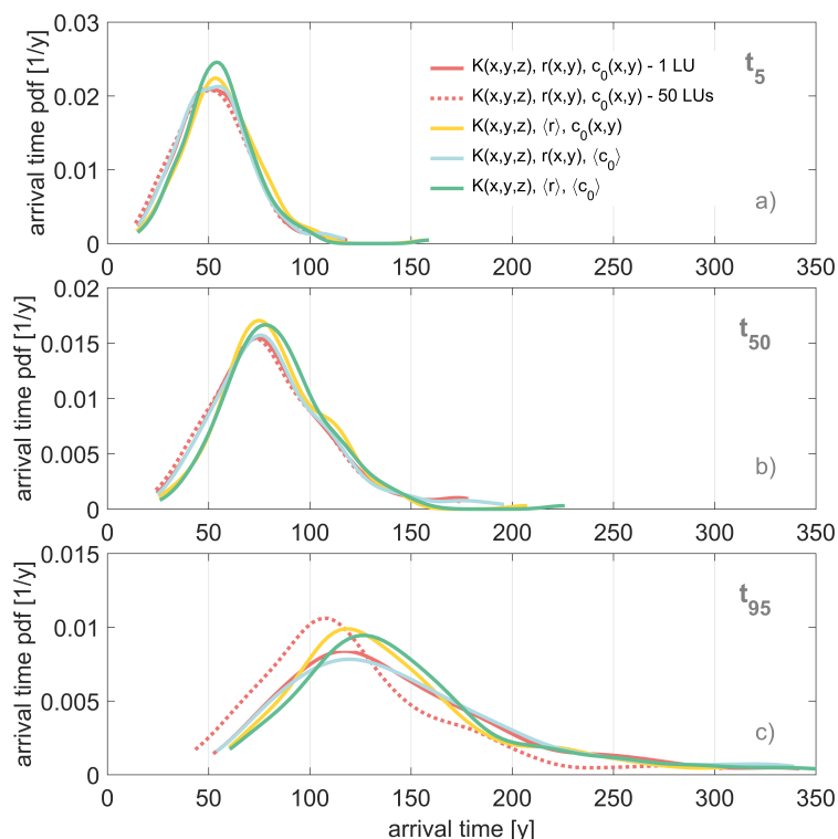
Figure 3. Probability density function of the time required for 5% (a), 50% (b), and 95% (c) of the total recorded mass to reach a well considering a heterogeneous r and heterogeneous c_0 (reference case, red line); a homogeneous r and heterogeneous c_0 (yellow line); a heterogeneous r and homogeneous c_0 (light blue line); a homogeneous r and homogeneous c_0 (green line). Plain lines refers to the consideration of an identical land-use map for all realizations. For comparison, the red dash lines shows outputs from simulations with a realization-dependent land-use maps.
