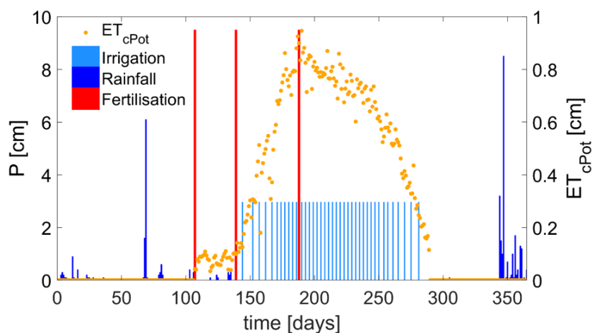
Figure 2. Illustration example of daily values of potential crop evapotranspiration (orange points) used for the description of the upper boundary condition. The blue bars represent rainfall events and the light blue bars irrigation events. The red bar defines fertilization application for an amount equal to 65 Kg/ha (195 Kg/ha/year). Crop is cotton.
