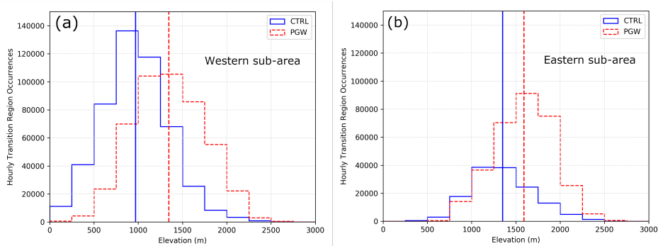
Fig. 2. Figure 10. Transition region occurrences for the (a) western and (b) eastern sub-areas binned according to elevation. Vertical solid blue lines and dashed red lines represent the average elevation ...
