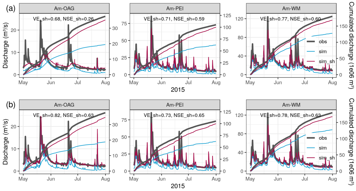
Figure 1: Simulated and observed discharge for calibration period (2015-05-01–2015-07-31). (a) Uniform soil layers throughout domain, (b) reduced soil layer thicknesses for slopes > 50\% .
