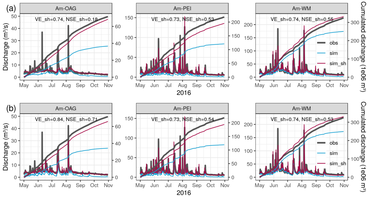
Figure 2: Simulated and observed discharge for calibration period (2016-05-01–2016-10-31). (a) Uniform soil layers throughout domain, (b) reduced soil layer thicknesses for slopes > 50\% .
