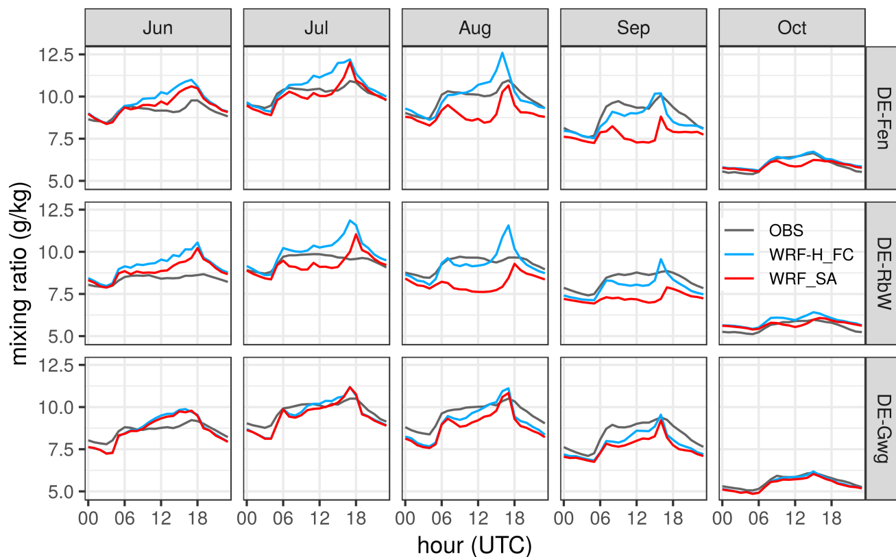
Figure 10. Mean diurnal cycles of simulated and observed 2m mixing ratio for the months June to October 2016 at different TERENO-preAlpine TERENO Pre-Alpine sites.
