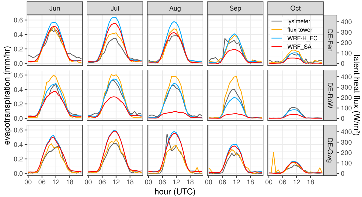
Figure 8. Mean diurnal cycles of simulated and observed latent heat flux / evapotranspiration for the months June to October 2016 at different TERENO-preAlpine TERENO Pre-Alpine sites.
