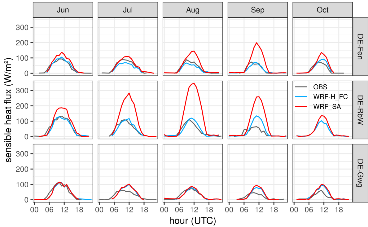
Figure 9. Mean diurnal cycles of simulated and observed sensible heat flux for the months June to October 2016 at different TERENO-preAlpine TERENO Pre-Alpine sites.
