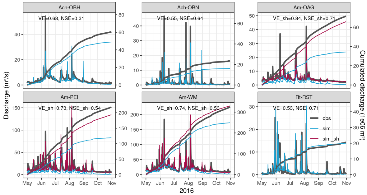
Figure 3: Re-simulated hydrographs for the validation period, 2016-05-01–2016-10-31 with artifact corrected RADOLAN precipitation data.
