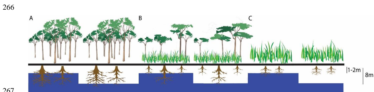
267 268 Figure 2: Diagram showing that forest (A) root depth can reach until the saturated zone in both shallow (< 2 m) and 269 deep (> 8 m) WTD, savanna (B) has a mixed rooting depth with only tree roots reaching deep WTD and crop (C) 270 vegetation have a low maximum rooting depth (crops having a maximum rooting depth of 2 m and savanna having a 271 maximum rooting depth > 10 m (Canadell et al., 1996). Shallow roots can reach the saturated zone in shallow WTD (< 272 2 m); however, they cannot reach the saturated zone in deep WTD (> 8 m).
