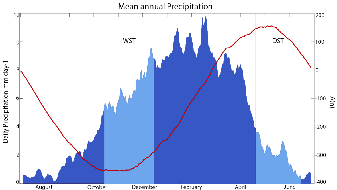
306 Figure 3 Mean annual precipitation of the study area calculated from TRMM with 7 day average for graphical 307 smoothing. wet season transition (WST) and dry season transition (DST) periods are represented in lighter blue. The 308 vertical lines represent the average start and end dates, however exact dates were calculated per year between July 2001 309 and July 2012. Red line represents anomalous accumulation method A(n) from Liebmann et al. (2007).
