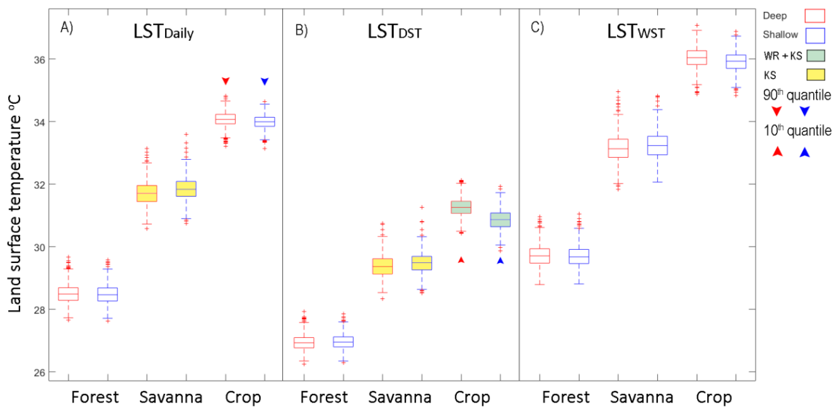
386 Figure 5. (A) Average daily land surface temperature (LST) annually LST_{daily} , (B) during the dry season transition 387 period LST_{DST} , (C) during the wet season transition LST_{WST} . Red boxes represent deep WTD Blue boxes represent 388 shallow WTD. Yellow filled boxes represent a statistical difference in skewness, calculated by Kolmogorov–Smirnov, 389 and green filled boxes represent statistical differences by both Wilcoxon-rank and Kolmogorov–Smirnov. Significant 390 differences in 10 th and 90 th quantile are depicted by the arrows.
