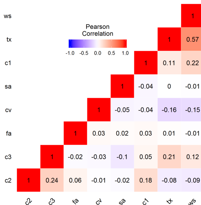
Figure 5. Pearson correlation matrix of the behavioural model parameters identified using the coupled RF and the limits of acceptability approach.
