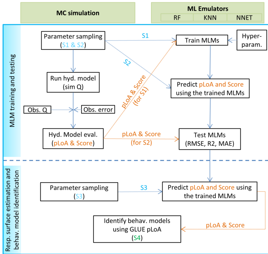
Figure 1. Schematic overview of the MLM training and testing as well as response surface prediction using the MLMs and the identification of behavioural models using the coupled MLM and GLUE pLoA.
