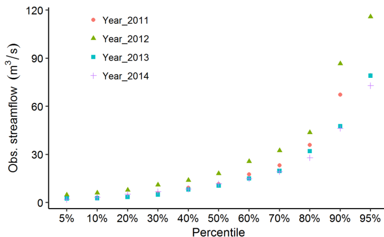
Figure 6. Comparison of the percentile observed streamflow values for the calibration period (Year_2011) and validation periods (Year_2012, Year_2013, and Year_2014)
