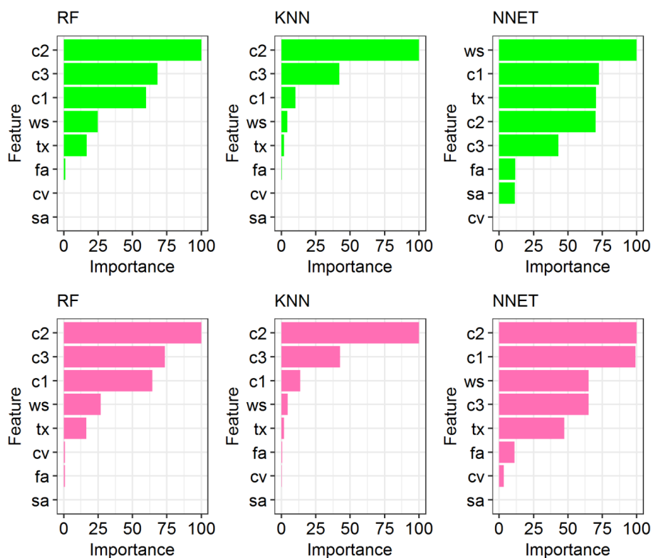
Figure 4. Relative importance of the hydrological model parameters based on the three machine learning models, i.e. RF, KNN, and NNET trained for pLoA (upper row) and Score (lower row)
