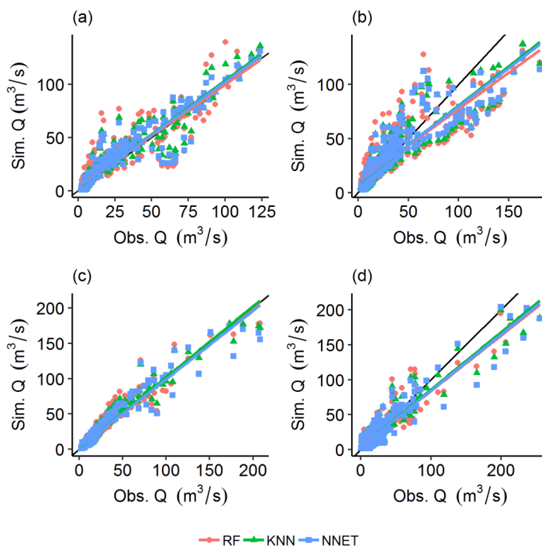
Figure 3. Scatterplots of simulated against observed streamflow values for the calibration period, i.e. year 2011 (a) and validation periods, i.e. years 2012 (b), 2013 (c), and 2014 (d). The behavioural models are identified using the coupled MLMs (RF, KNN, and NNET) and GLUE pLoA.
