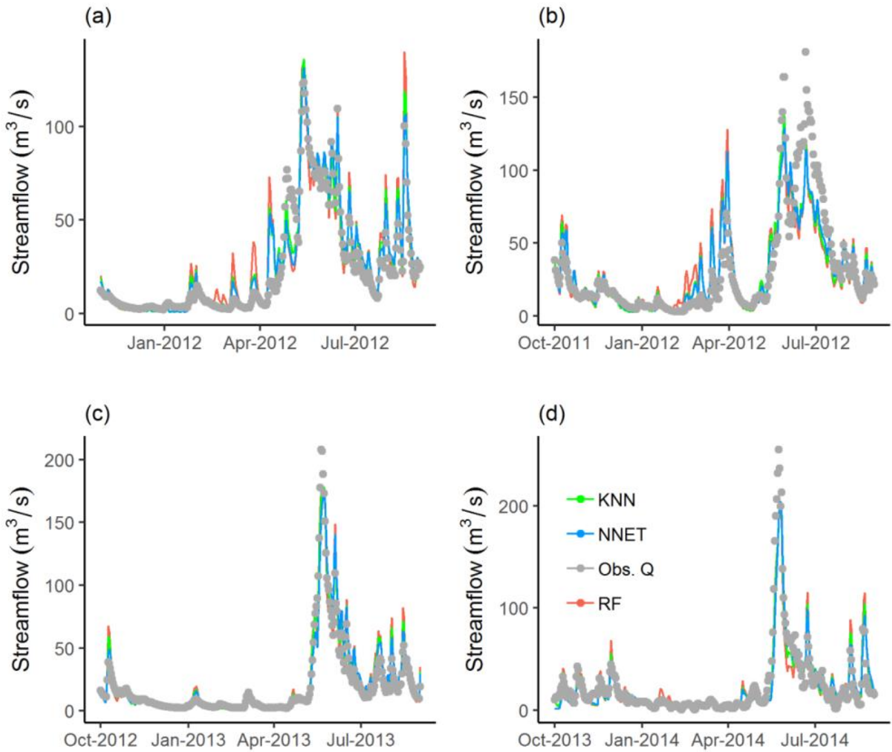
10 Figure 4. Simulated and observed streamflow values for the calibration period, i.e. year 2011 (a) and validation periods, i.e. years 2012 (b), 2013 (c), and 2014 (d). The behavioural models are identified using the coupled MLMs (RF, KNN, and NNET) and GLUE pLoA.
