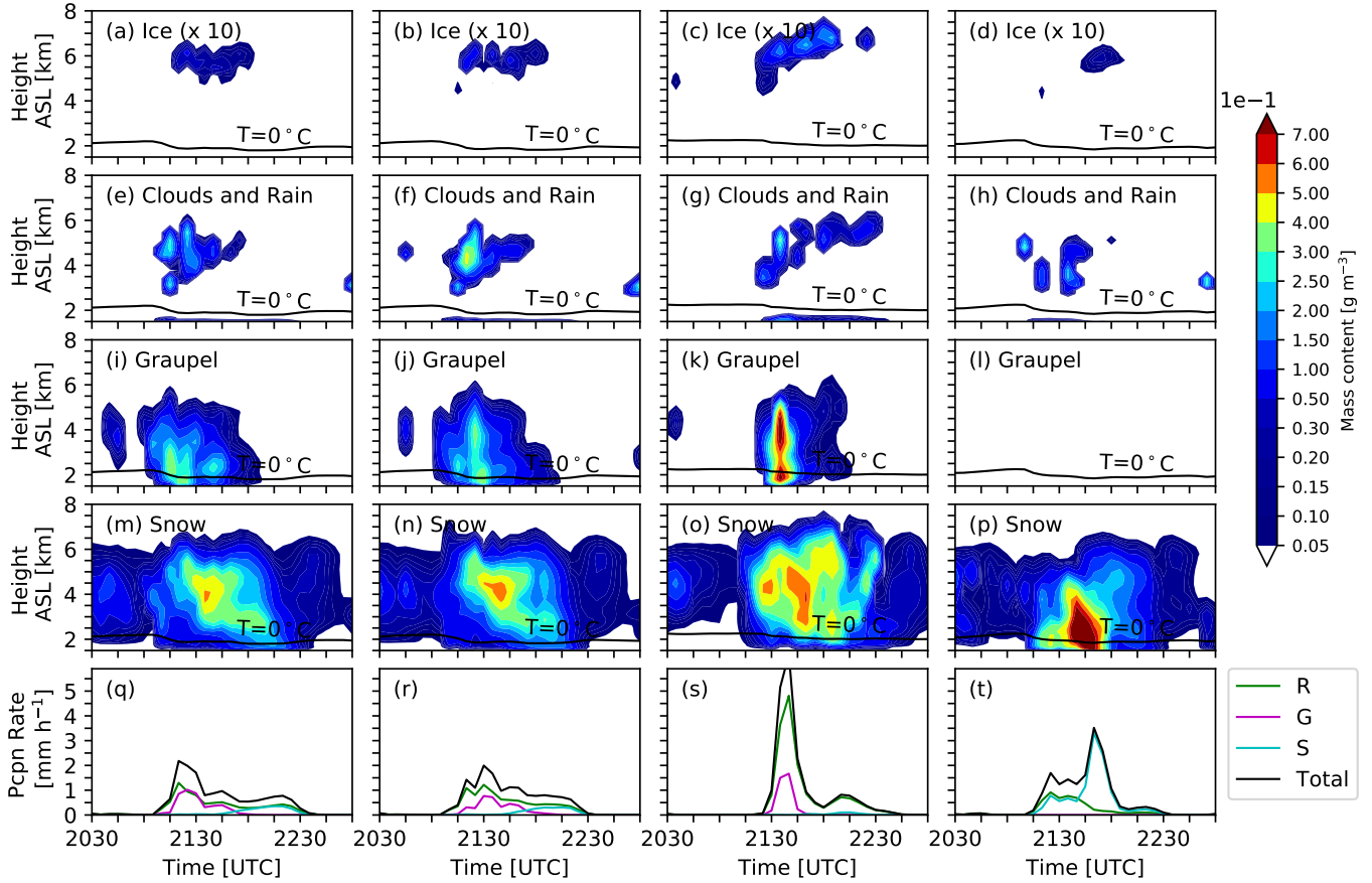
Figure 5. Comparison of the time evolution of hydrometeors mass content ( \text{g/m}^3 ) at the surface and aloft at KES during the 4 simulations conducted for CTR, NO_MLT, NO_SBL and NO_GRPL from left to right. (a-d) is ice mass content ( \times 10 \text{ g/m}^3 ), (e-h) is clouds and rain mass content, where rain is only formed through melting of ice, so it is only present near the surface, (i-l) is graupel mass content, (m-p) is snow mass content and (q-t) is the surface precipitation rate of rain (R), graupel (G) and snow (S). The 0^\circ\text{C} isotherm is indicated by the solid black line on (a-p). Panels a-p have the same colour scale.
