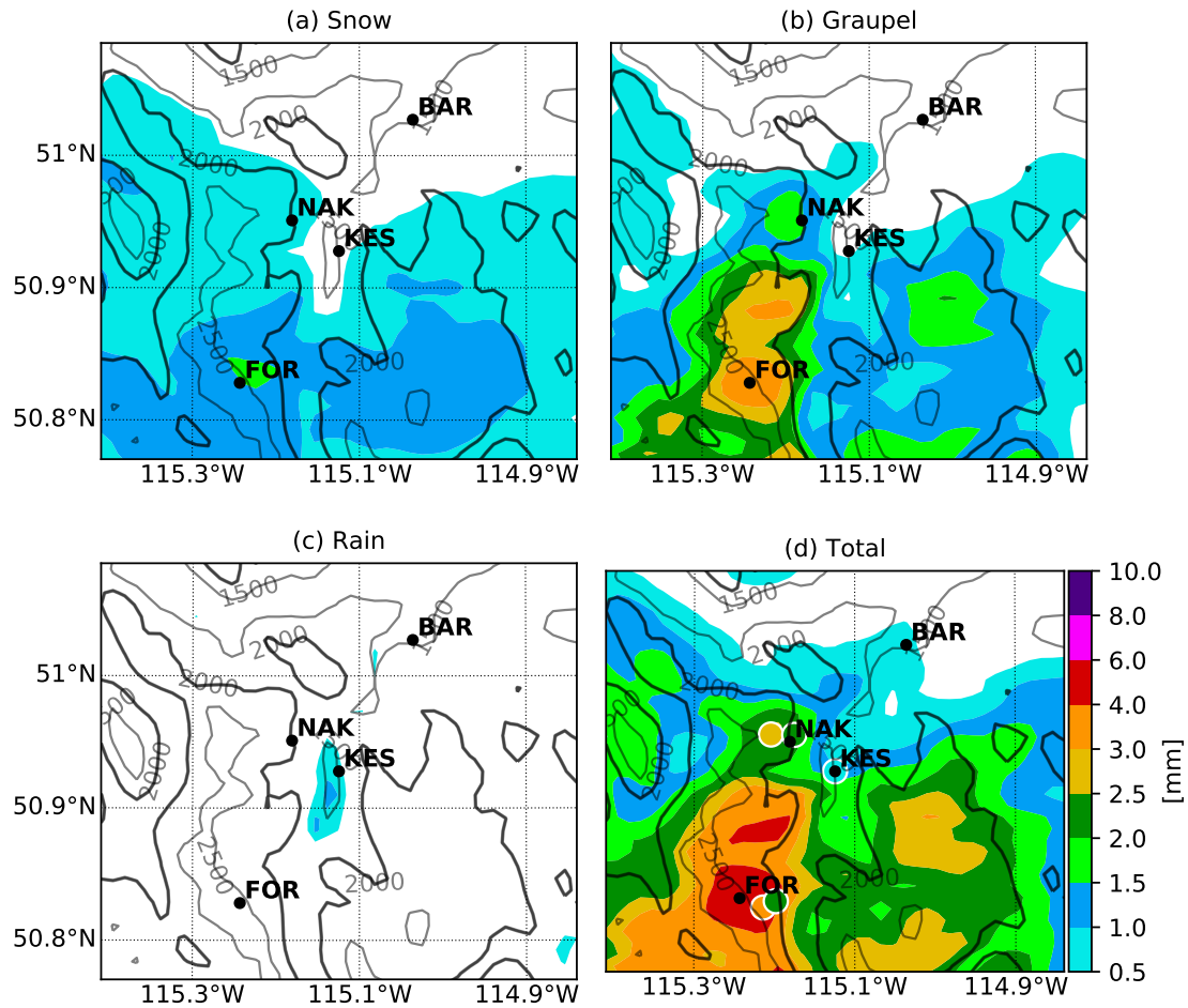
Figure 4. Simulated (a) unadjusted accumulated solid precipitation (mm) including (a) snow and (b) graupel, (c) rain and (d) total accumulated precipitation between 2000 UTC 31 March 2015 and 0000 UTC 1 April 2015. The coloured circles in (d) are the observations at 4 locations. These are KES (2.7 mm), Nakiska (2.2 mm), Fortress (3 mm) and Barrier Lake Station (0.8 mm). Accumulated precipitation is in liquid equivalent. The black lines are the topography in meters.
