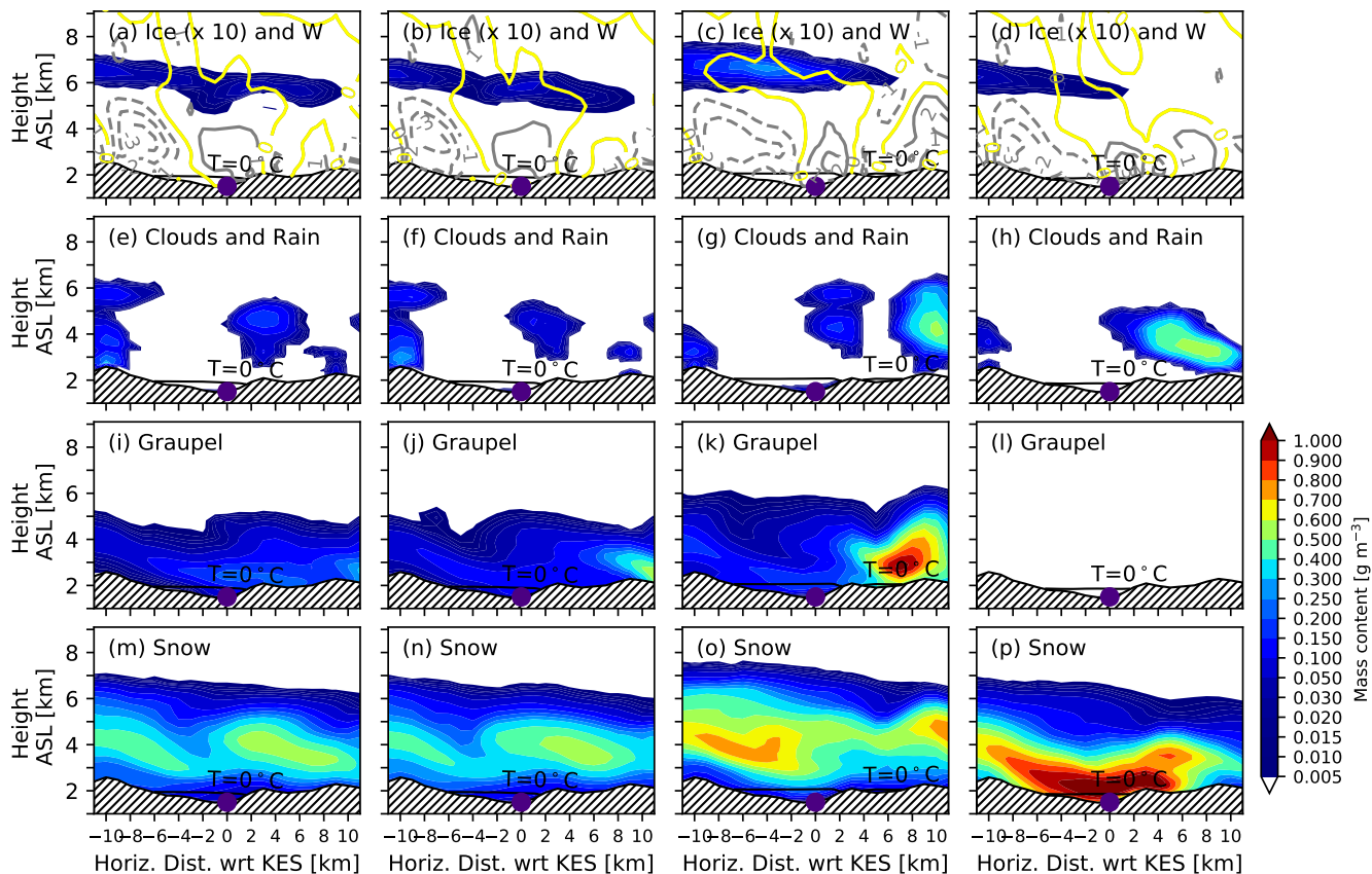
Figure 6. Comparison of the vertical cross-section across the Kananaskis Valley along the red line in Fig. 1 showing the mass content of hydrometeors ( \text{g}/\text{m}^3 during the 4 simulations conducted for CTR, NO_MLT, NO_SBL and NO_GRPL from left to right. (a-d) is ice mass content ( \times 10 \text{ g}/\text{m}^3 ) with vertical velocity ( \text{m}/\text{s} ). The yellow line is 0 \text{ m}/\text{s} , the dashed lines are negative values and solid lines are positive values, (e-h) is clouds and rain mass content, (i-l) is graupel mass content and (m-p) is snow mass content. The 0^\circ\text{C} isotherm is indicated by the solid black line. Panels a-p have the same colour scale. The location of KES is indicated by the purple dot.
