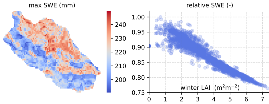
Figure 11. Spatial variability of maximum snow water equivalent ( SWE_{SWE} ) at C3 (left). The SWE_{SWE} relative to open area scales near-linearly with wintertime leaf-area index LAI_{LAI} (right).
