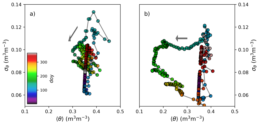
Figure 8. Temporal stability of soil moisture at C3 during wet year (2012) and dry year (2013). Top: Timeseries of The relationship between catchment daily mean root-zone soil moisture \langle \theta \rangle (m 3 m -3 ) and its spatial standard deviation \sigma_\theta over the course a wet (dashed line 2012) and dry (2013) year at C3 Porkkavaara. The gray range color scale shows IQR day of \langle \theta \rangle . Bottom: Relationship of \sigma_\theta and \langle \theta \rangle over the course of year (doy).
