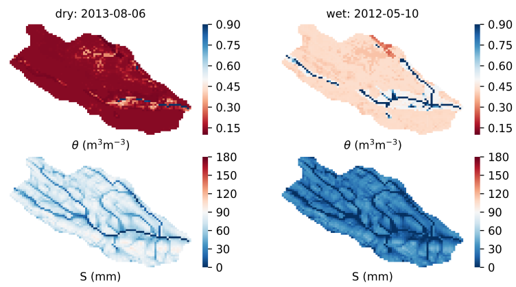
Figure 9. Snapshots of soil moisture patterns during wet and dry conditions ( Fig. 7 ) at C3 Porkkavaara . Water content \theta in the root zone (top) and local saturation deficit S of Topmodel (bottom).
