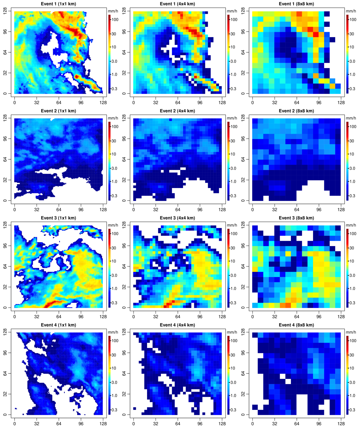
Figure 6. Original 1 \times 1 \text{ km}^2 and upscaled ( 4 \times 4 \text{ km}^2 and 8 \times 8 \text{ km}^2 ) 5-min radar rainfall snapshots for events 1 to 4.
