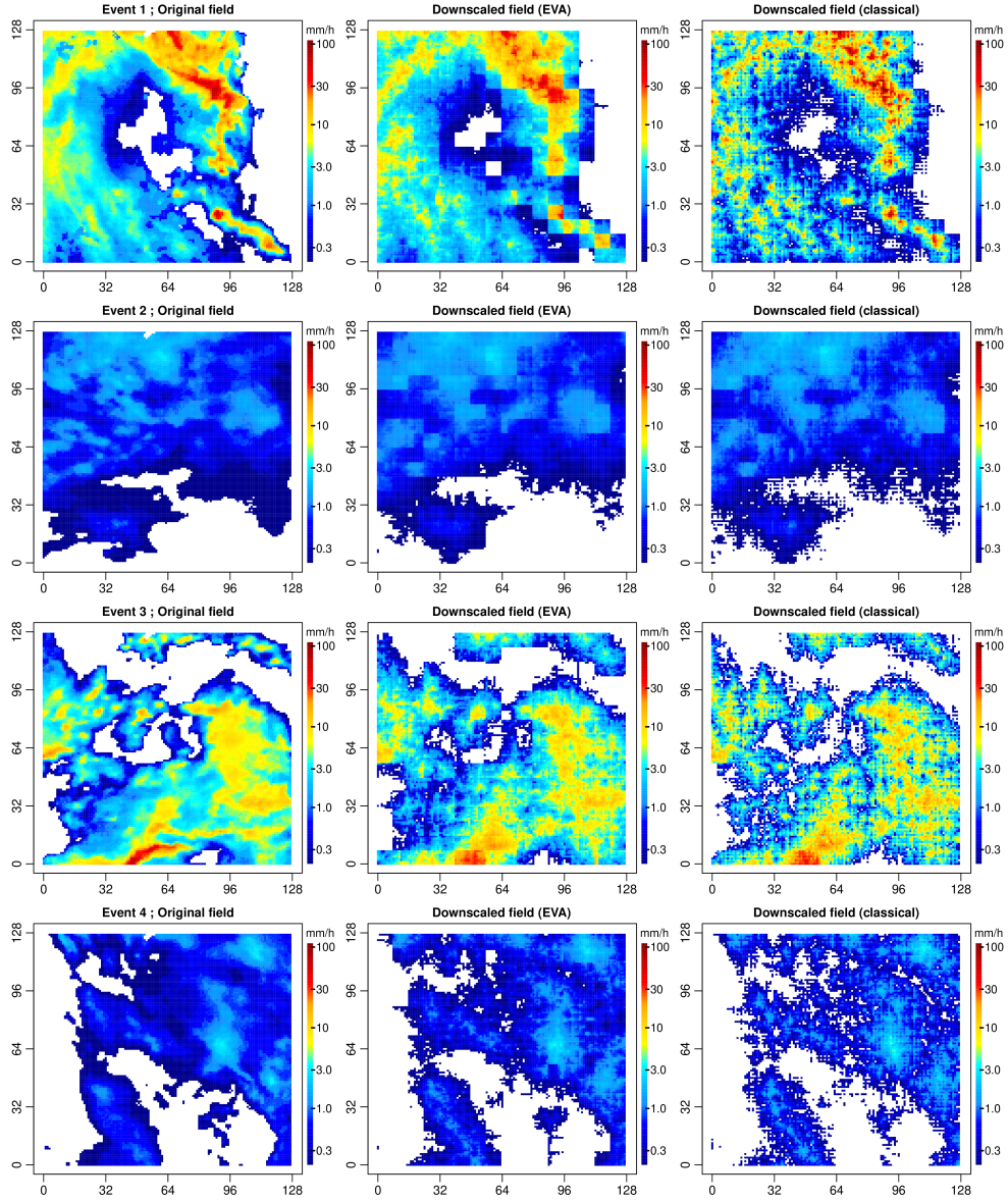
Figure 10. Downscaled rainfall fields for events 1-4 and a downscaling factor of 64 (i.e., input resolution of 8 \times 8 \text{ km}^2 and target resolution of 1 \times 1 \text{ km}^2 ). The left column shows the original radar rainfall snapshots at 1 \times 1 \text{ km}^2 . The middle and right columns show the outputs of the EVA and classical cascade models for the (biased) coarse-scale sample generator. Only the first of 100 different random realizations for each field and cascade model is shown.
