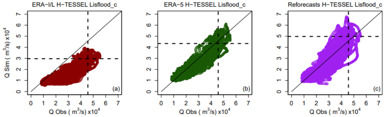
Figure 10: Scatterplots of observed against simulated river flow at the Tamshiyacu gauging site, Peru (4). For (a) ERA-Interim Land, (b) ERA-5 and (c) the European Centre for Medium-range Weather Forecasts (ECMWF) 20-year reforecasts forced through the calibrated Lisflood routing model. Dashed black lines indicate the observed and simulated 90 th percentile of river flow. For the period 1997-2015.
