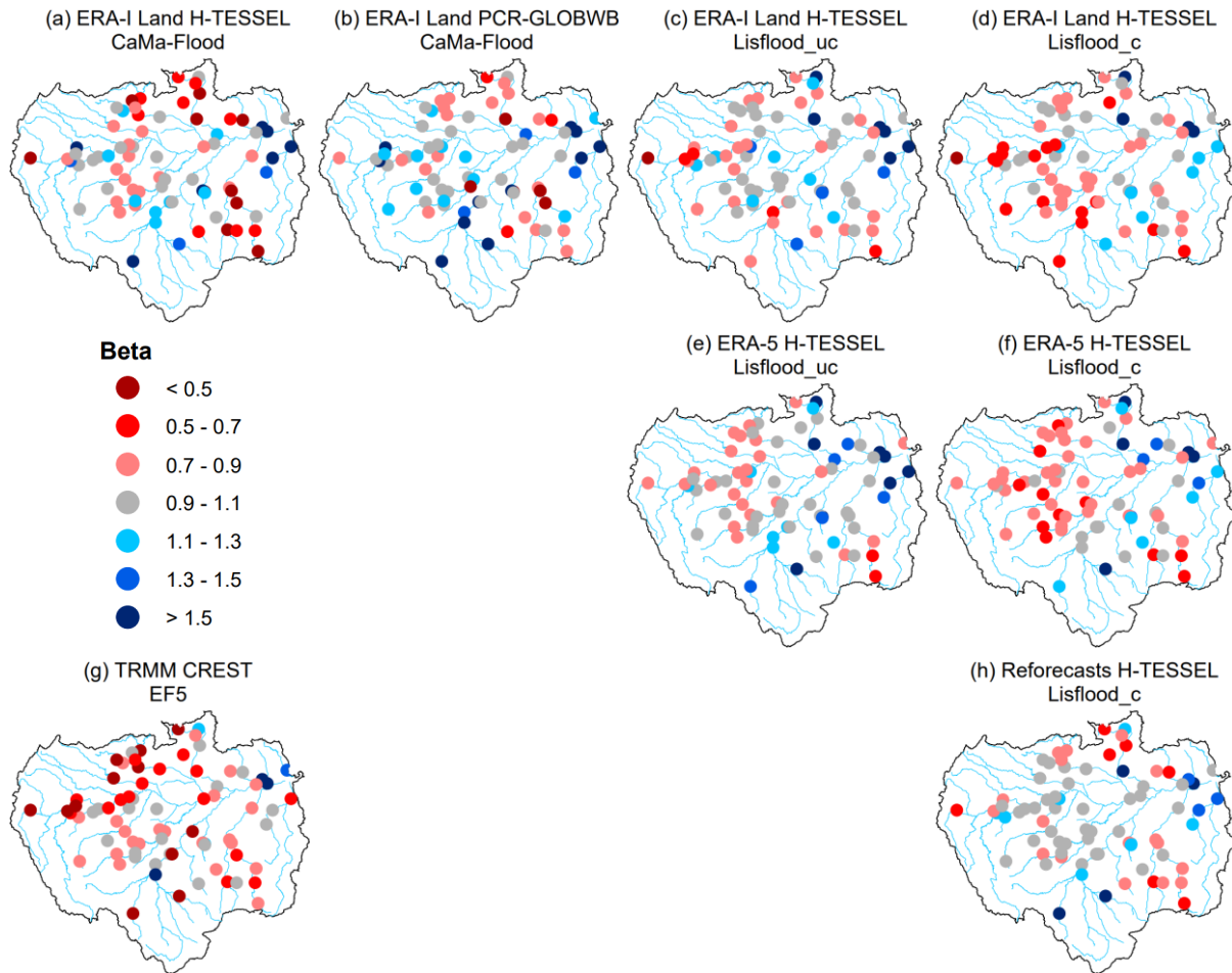
5 Figure 5: Beta (i.e. bias ratio) component of the Kling Gupta Efficiency (KGE) at the 75 hydrological gauging stations for all simulations. For the period 1997-2015 and 2004-2015 for the Coupled Routing and Excess Storage, Ensemble Framework for Flash Flood Forecasting (CREST EF5) run (g). Blue circles indicate that the bias in the simulated time series is higher than that of the observed, while red circles show the opposite effect. Values closer to one indicate better model performance (i.e. grey circles).
