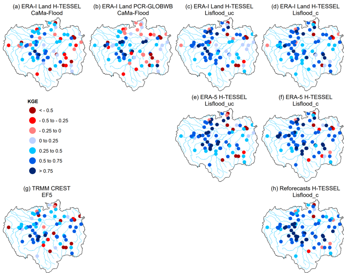
Figure 2: Full Kling Gupta Efficiency (KGE) scores at the 75 hydrological gauging stations for all simulations. For the period 1997-2015 and 2004-2015 for the Coupled Routing and Excess Storage, Ensemble Framework for Flash Flood Forecasting (CREST EF5) run (g). Values greater than 0.75 are considered to indicate good performance (i.e. dark blue circles). To allow for easier model comparisons, plots are arranged by the different precipitation datasets (rows) and routing models (columns) with the exception of CREST EF5 (g). For example, the final column consists of model runs using the calibrated Lisflood routing model.
