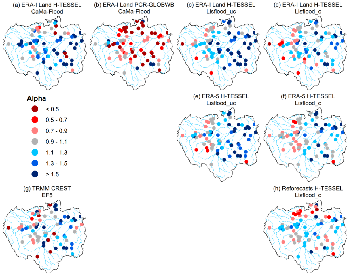
5 Figure 4: Alpha (i.e. variability ratio) component of the Kling Gupta Efficiency (KGE) at the 75 hydrological gauging stations for all simulations. For the period 1997-2015 and 2004-2015 for the Coupled Routing and Excess Storage, Ensemble Framework for Flash Flood Forecasting (CREST EF5) run (g). Blue circles indicate that the variability in the simulated time series is higher than that of the observed, while red circles show the opposite effect. Values closer to one indicate better model performance (i.e. grey circles).
