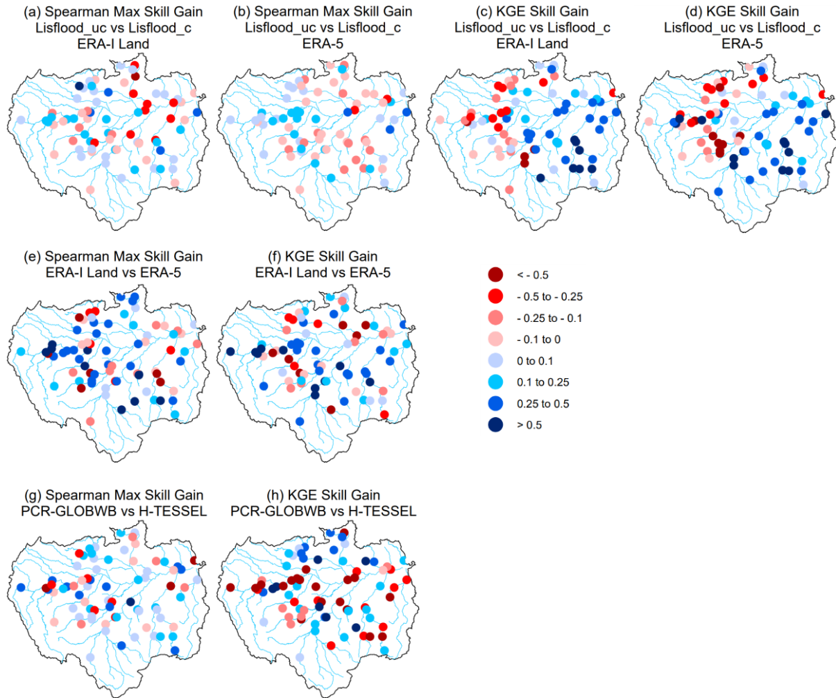
Figure 9: Relative improvement in skill at each gauging station for Spearman annual maximum correlations and Kling Gupta Efficiency (KGE) values (i.e. skill scores). (a-d) show relative gain or loss in skill when using the calibrated Lisflood run (Lisflood_c) relative to the uncalibrated model run (Lisflood_uc), using precipitation forcing from both ERA-Interim Land and ERA-5. (e-f) shows the relative gain or loss in skill when using ERA-5 as opposed to ERA-Interim Land. (g-h) shows the relative gain or loss in skill when using the Land Surface Model (LSM), the Hydrology-Tiled ECMWF Scheme for Surface Exchanges over Land (H-TESEL) compared to the hydrological model, PCRaster Global Water Balance (PCR-GLOBWB). All scores are calculated using the skill scores in Eq. (1). Red circles indicate a decrease in skill, whereas blue circles represent an increase.
