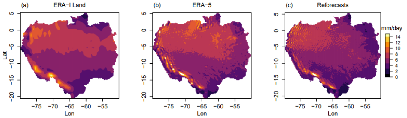
Figure 8: Mean daily precipitation totals throughout the Amazon basin. For (a) ERA-Interim Land, (b) ERA-5 and (c) the European Centre for Medium-range Weather Forecasts (ECMWF) 20-year reforecasts. For the period 1997-2015.
