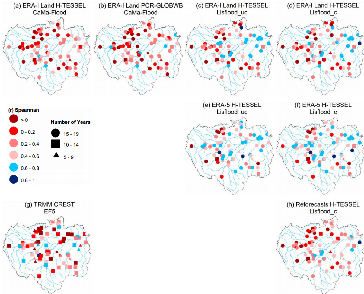
Figure 6: Spearman's ranked correlation coefficients for observed against simulated annual maximum discharge values at the 75 hydrological gauging stations for all simulations. For the period 1997-2015 and 2004-2015 for the Coupled Routing and Excess Storage, Ensemble Framework for Flash Flood Forecasting (CREST EF5) run (g). Values exceeding 0.6 are considered skillful (i.e. blue shapes). Number of overlapping years of data between observations and simulations are denoted by different shapes. A triangle represents 5-9 years, a square 10-14 years and a circle 15-19 years of overlapping data.
