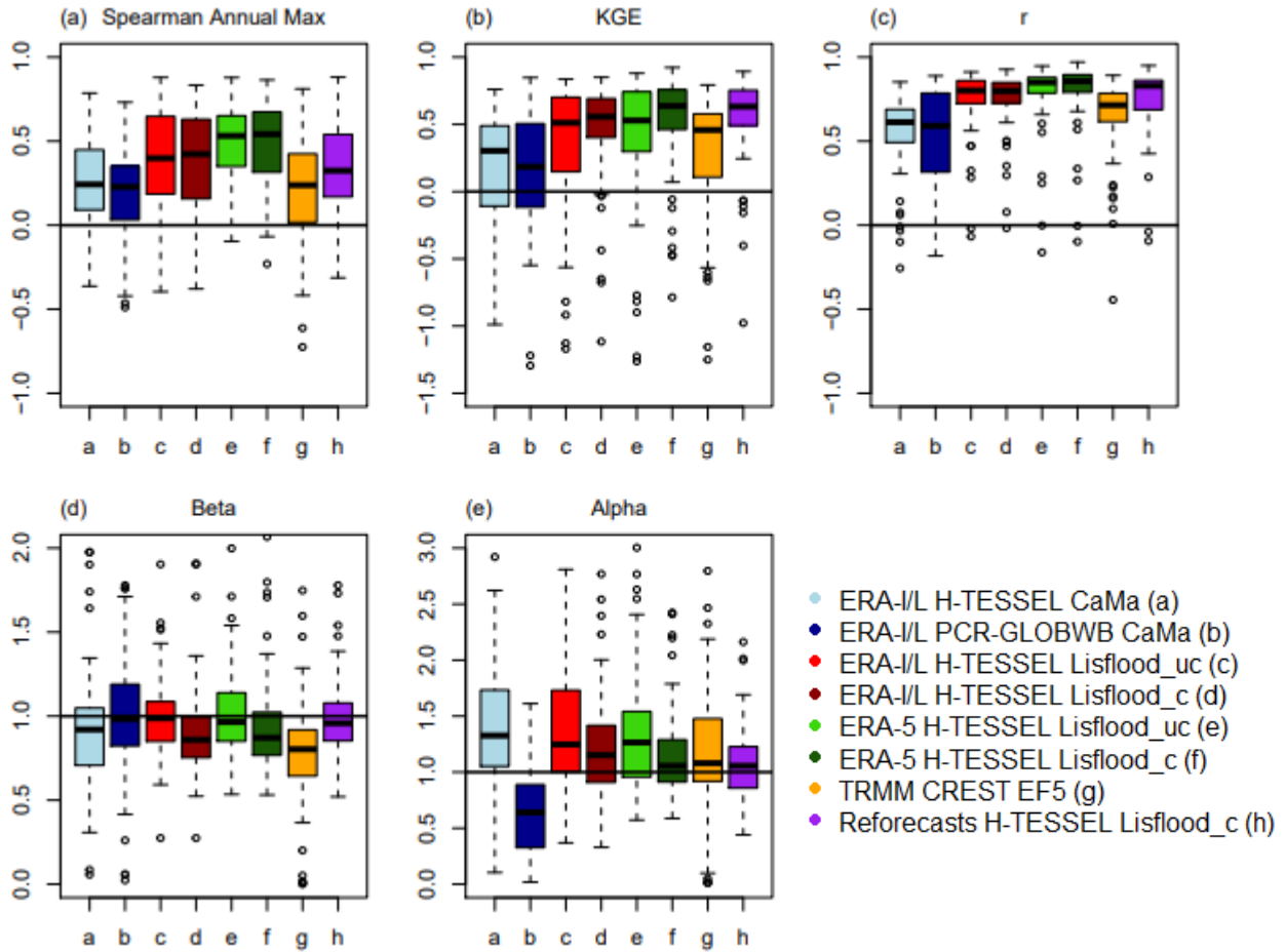
Figure 7: Boxplots showing the distribution of scores for the (a) Spearman annual maximum correlation (b) Kling Gupta Efficiency (KGE), (c) KGE Pearson's coefficient, (d) KGE beta and (e) KGE alpha, for all simulations. For the period 1997-2015.
