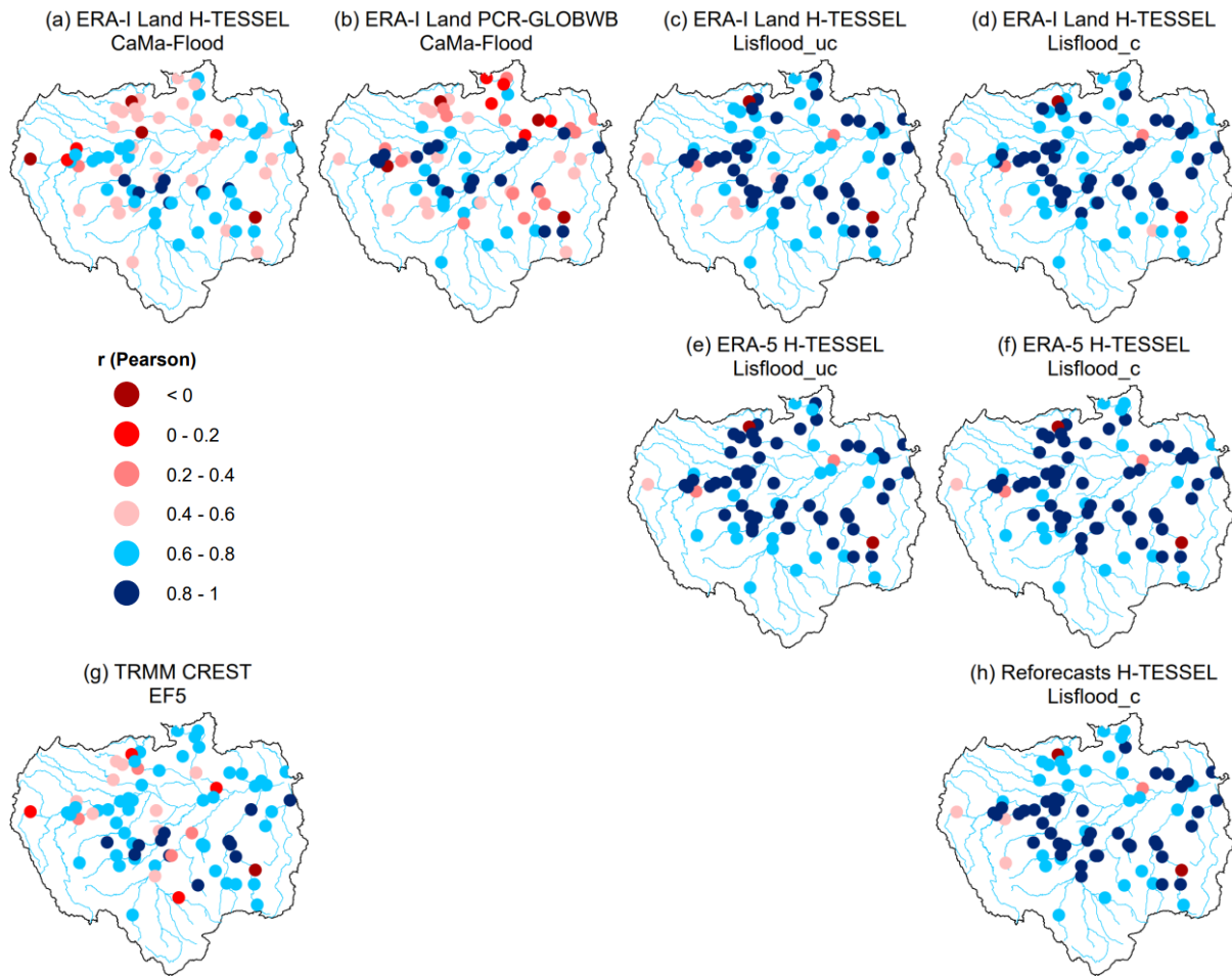
Figure 3: Correlation component (Pearson's) of the Kling Gupta Efficiency (KGE) at the 75 hydrological gauging stations for all simulations. For the period 1997-2015 and 2004-2015 for the Coupled Routing and Excess Storage, Ensemble Framework for Flash Flood Forecasting (CREST EF5) run (g). Values greater than 0.6 are considered skilful (i.e. blue circles).
