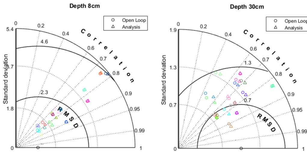
Figure 7. Taylor Diagrams (TD) drawn from the comparison between in situ -observed and SFX-simulated (background and analysis) soil moisture for the two different soil depth.
