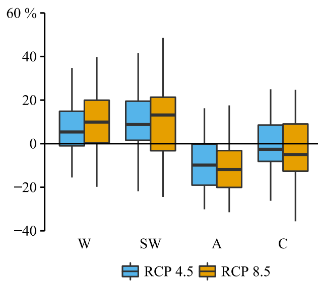
Figure A3. Changes in the winter WT occurrences for RCP 4.5 and RCP 8.5. The changes are obtained using the climate model output for 2071-2100 with respect to the output for 1961-1990.
