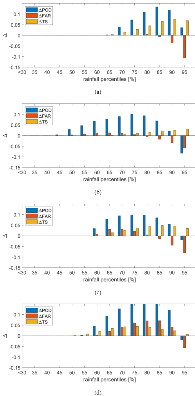
Figure 7. Difference in categorical indices (Probability of detection, POD, False Alarm Ratio, FAR and and Threat Score, TS) between the integrated product P_{R+SM} and the IMERG-ER as a function of the rainfall classes for Australia (a), CONUS (b), Europe (c) and India (d). Period 2015-2017.
