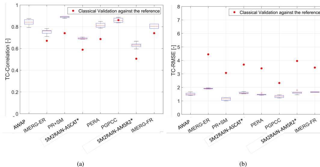
Figure 8. Box plots of TC correlation R_{TC} (a) and root mean squared error RMSE_{TC} (b) obtained in Australia by considering the different outcomes of the 15 triplets compared with the classical correlation and RMSE scores (red dots) obtained by comparing the different rainfall products against AWAP.
