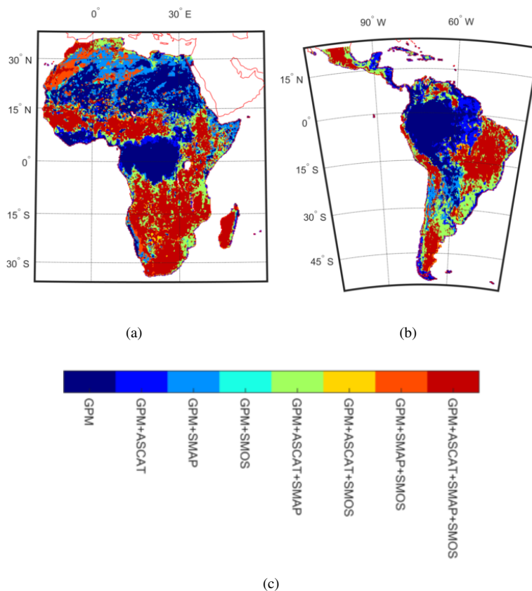
Figure 9. Products used to integrate IMERG-ER with SM2RAIN products derived from the setup during the calibration period in South America. When low correlation was found between the reference dataset (ie., GPCC) and the SM2RAIN product, the latter was excluded from the analysis and only IMERG-ER was retained.
