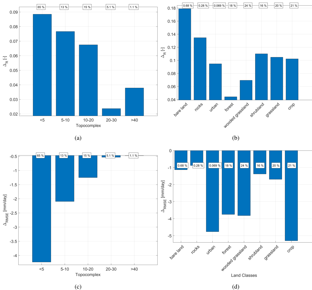
Figure 6. Difference in correlation ( \Delta_R ) and in root mean square error ( \Delta_{RMSE} ) between the integrated product P_{R+SM} and IMERG-ER as a function of the topographic complexity (panels a and c) and as a function of the Land Cover type (panels b and d) over CONUS. The results refer to 2015-2017 period. The text boxes on the top show the percentage of the area occupied by the specific topographic complexity or land cover type.
