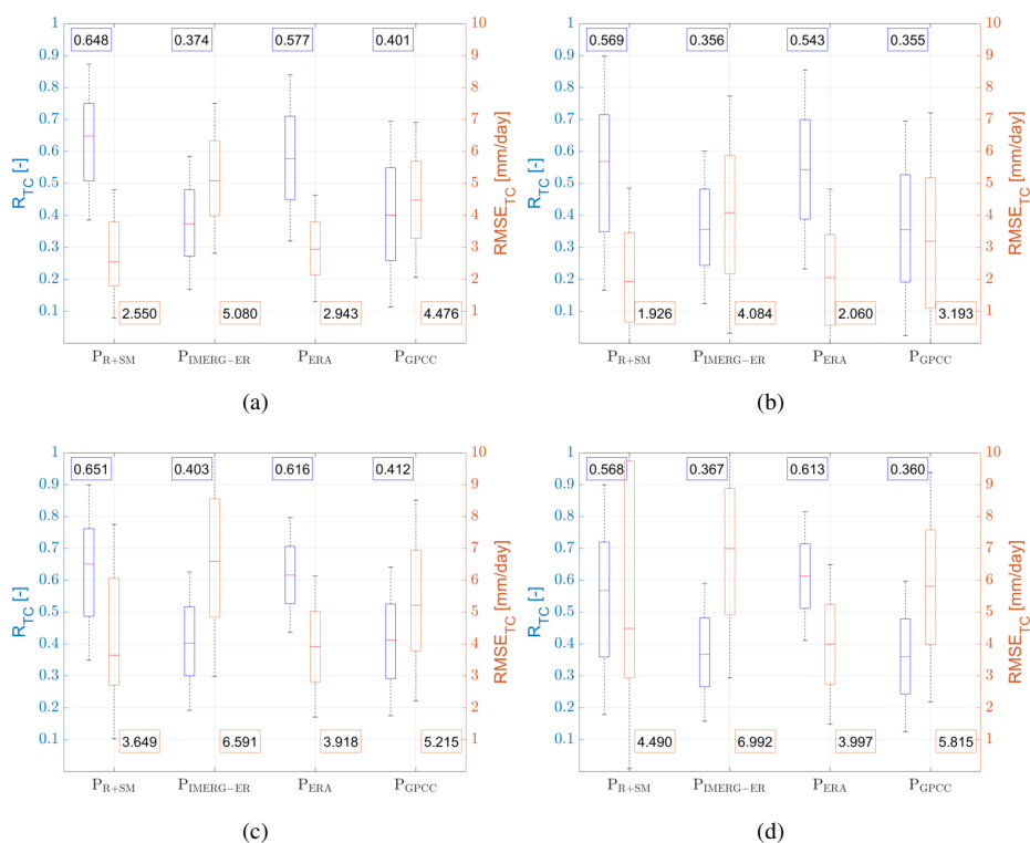
Figure 12. Box plots of Triple collocation squared correlation ( R_{TC}^2 , left axis in blue) and Root Mean Square error ( RMSE_{TC} , right axis in red) in mm/day obtained during validation period (i.e., 2018) in Africa over the committed area mask (a) and over all the study area (b). (c) and (d) refer to the same results but in South America. The box plot refer to the 25 th and 75 th percentiles while the whiskers refer the minimum and maximum values.
