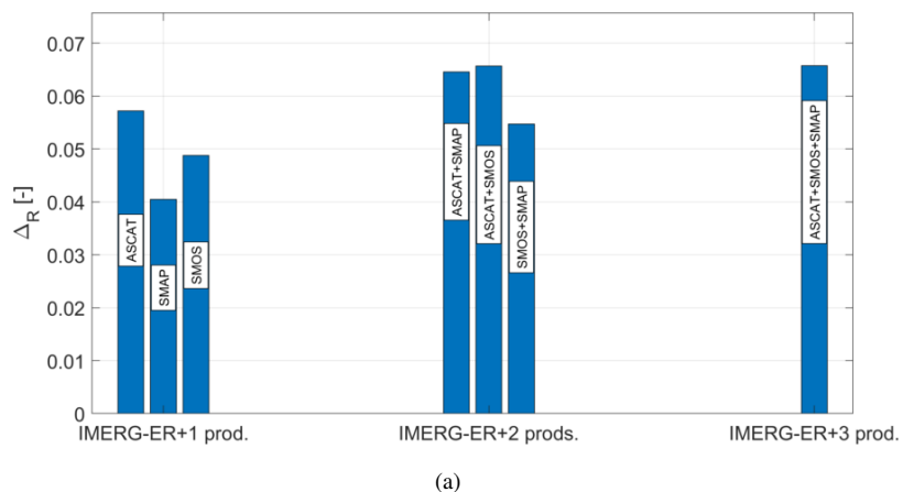
Figure 4. Increments obtained in terms of correlation against AWAP after the inclusion of more satellite soil moisture products via SM2RAIN in the integration scheme.
