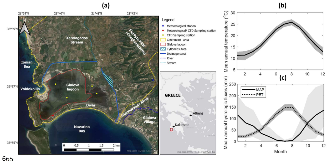
Fig. 1. a) Map of the study area; b) long-term mean annual temperature; c) long-term mean annual precipitation (MAP) and potential evapotranspiration (PET). In panels (b) and (c), shaded areas indicate the variability around the mean (5 th and 95 th percentiles). Sources for panel (a): AeroGRID, CNES/Airbus DS, DigitalGlobe, Earthstar Geographics, Esri, Garmin, GeoEye, GIS user community, HERE, IGN, © OpenStreetMap contributors 2019 (distributed under a Creative Commons BY-SA License), USDA, USGS.
