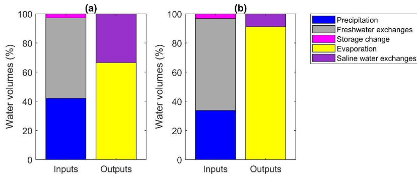
Fig. 5. Water budgets over the whole study period for a) current conditions and b) future conditions (scenario C3: reduced precipitation and increased evaporation rate, see Table 2). Water volumes are expressed as percentage of the total volume entering or leaving the lagoon, and only the net saline water exchanges are included in the budgets.
