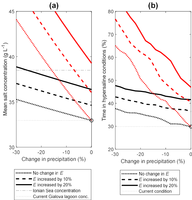
780 Fig. 6. Effect of climatic changes on a) the mean salt concentration in the Gialova lagoon and b) the percentage of time under hypersaline conditions. Different line styles refer to three scenarios for changes in evaporation rate; red lines refer to scenarios where freshwater fluxes are reduced as a result of climatic changes. Percentage time is calculated for the two simulation years; for visual reference, the grey horizontal dotted lines indicate current salinity and duration of hypersaline conditions in the Gialova lagoon, and the 785 grey dot-dashed line in a) indicates salt concentration in the Ionian Sea as of today; current conditions are indicated by open circles.
