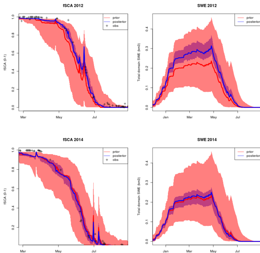
Figure 8. Assimilation of fSCA at grid level which targets bias in grid level forcing. Two contrasting seasons, WY2012 (top row) and WY2014 (bottom row) are shown. Vertical dashed lines give the assimilation window. Grid level biases in WY2012 are compensated for by DA. Grid level forcing was much more accurate in WY2014 and resulting effect of DA was negligible.
