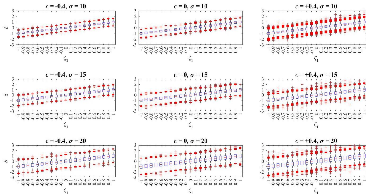
Figure 7: Empirical distributions of \delta evaluated from samples with L = 30 , vs trend coefficient \zeta_1
