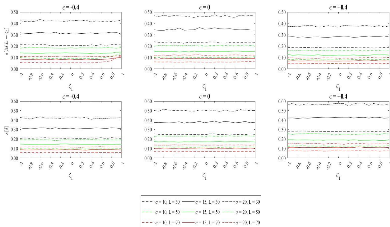
Figure 6: Sample variability of ML-\zeta_1 and \delta vs trend coefficient \zeta_1
