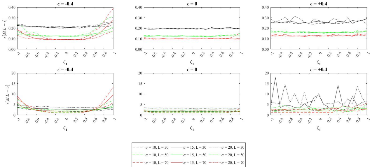
Figure 9: Sample variability of ML- \epsilon and ML- \sigma vs trend coefficient \zeta_1
