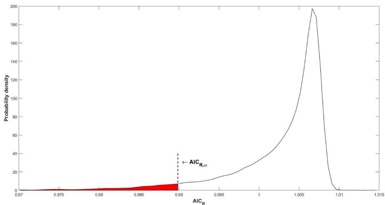
Figure 1: Empirical distribution of AIC_R and rejection threshold AIC_{R,\alpha} of the null hypothesis (stationary GEV parent)
