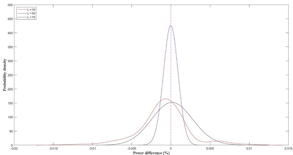
Figure 2: Distributions of the differences between power of AIC_R evaluated with AIC and AIC_c for \epsilon = 0.4
