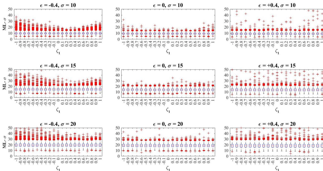
Figure 12: Empirical distributions of ML-\sigma evaluated from samples with L = 30 vs trend coefficient \zeta_1
