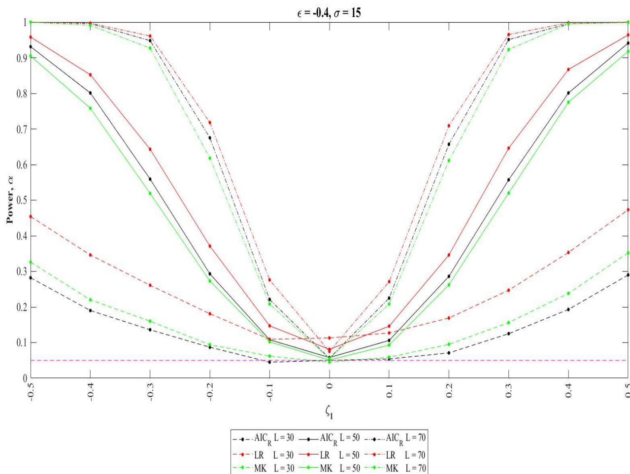
Figure 4: Focus on the actual level of significance reported for \zeta_1 = 0 .
