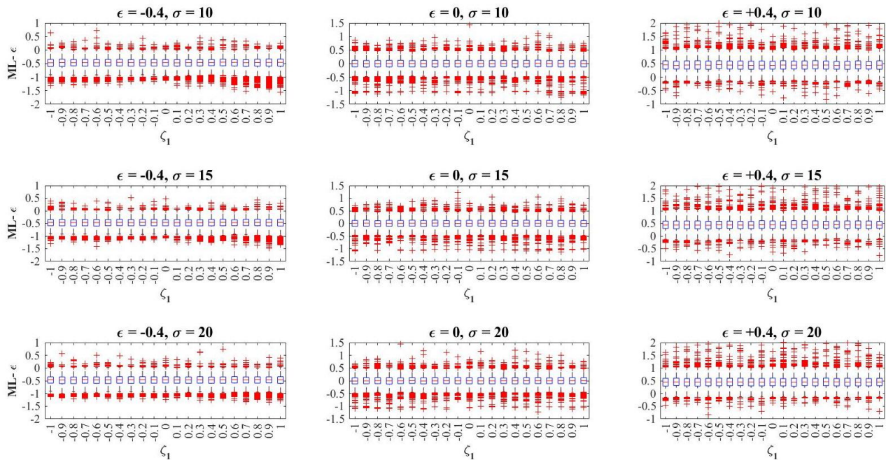
Figure 10: Empirical distributions of ML- \epsilon evaluated from samples with L = 30 vs trend coefficient \zeta_1
