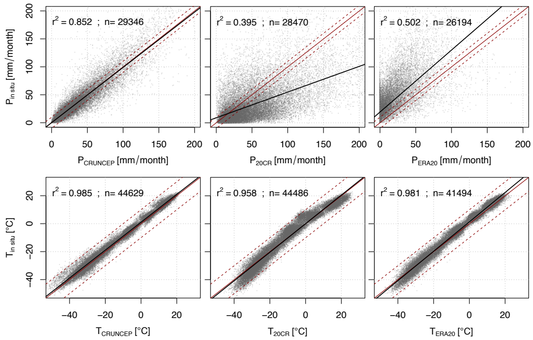
Figure 5: Comparison of three reanalysis datasets with in situ records (RIHMI-WDC) for monthly values. Red solid line is the 1:1-line; red dashed line is \pm 10\text{mm} for precipitation and \pm 10^\circ\text{C} for temperatures.
