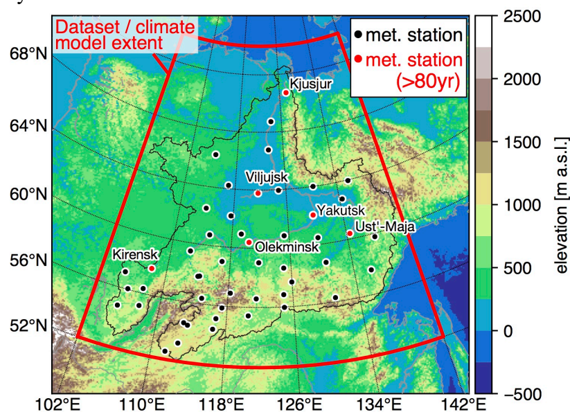
Figure 1: Lena River catchment (black outline) on topographic map (colour-code) and position of short-, and long-term meteorological stations used to test reanalysis and interpolated datasets. From the long-term stations, Kjusjur has the lowest temporal coverage (less than 10 years) in the reference period 1901-1921.
