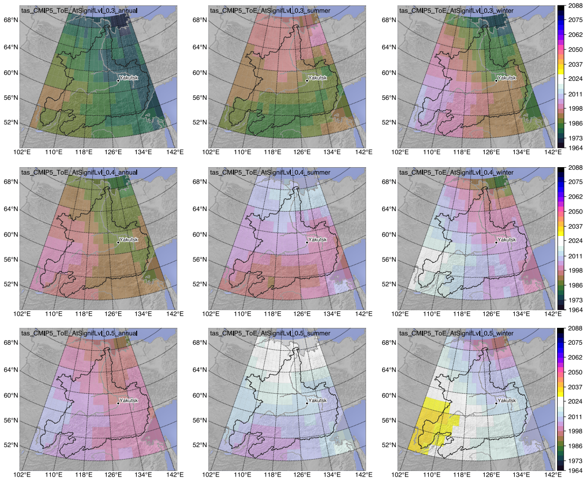
20 Figure 8: Time of emergence for temperature according to 30% (top), 40%(middle), and 50%(bottom) emergence for annual (left), summer (middle), and winter (right) values. Values are the mean over all individually determined ToE for each of the 65 climate simulations.
