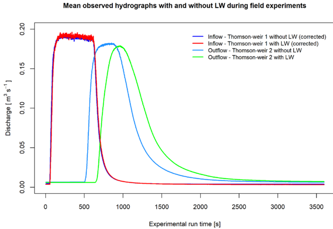
Figure 5: Average measured and corrected flood hydrographs observed during field experiments with and without stable in-channel large wood at both Thomson-weirs (after Wenzel et al., 2014).
