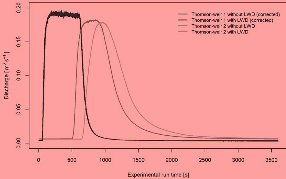
Mean observed hydrographs with and without LWD during field experiments
