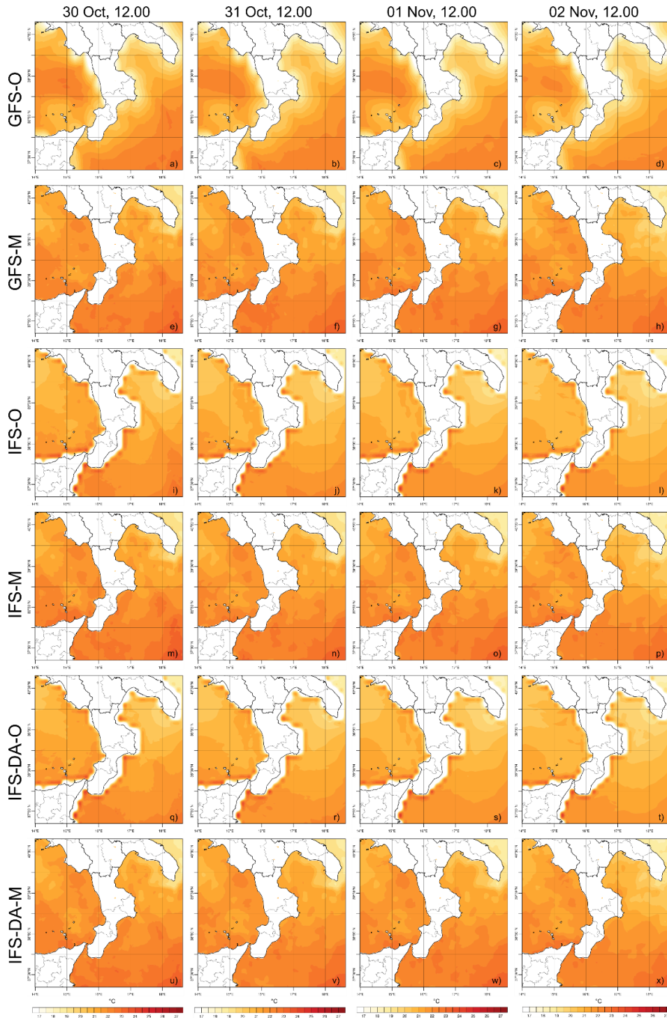
Fig. S2: Case study 2: maps of SSTSK ( ^{\circ}\text{C} ) in the domain D02, for the six simulations listed in Table 2, from 12 UTC 30 October 2015 to 12 UTC 02 November 2015, every 24 hours.
