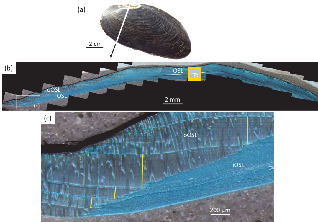
835 Figure 2: Sclerochronological analysis of Margaritifera margaritifera . (a) Left valve of a freshwater pearl mussel. Cutting axis is indicated with white line. (b) Mutvei-immersed shell slab showing the outer and inner shell layers (OSL, ISL) separated by the myostracum (white line). The OSL is further subdivided into an outer and inner portion (oOSL, 840 iOSL). ISL and iOSL consist of nacreous ultrastructure, the oOSL of prismatic ultrastructure. (c) Enlargement of B shows annual growth patterns. Annual increment width measurements (yellow) were completed as perpendiculars from the intersection of the oOSL and iOSL toward the next annual growth line.
