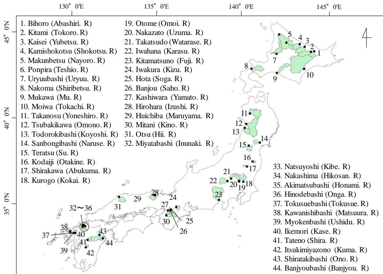
540 Figure 1: Location of the study site. The 44 observation stations in the Japanese archipelago were considered.
