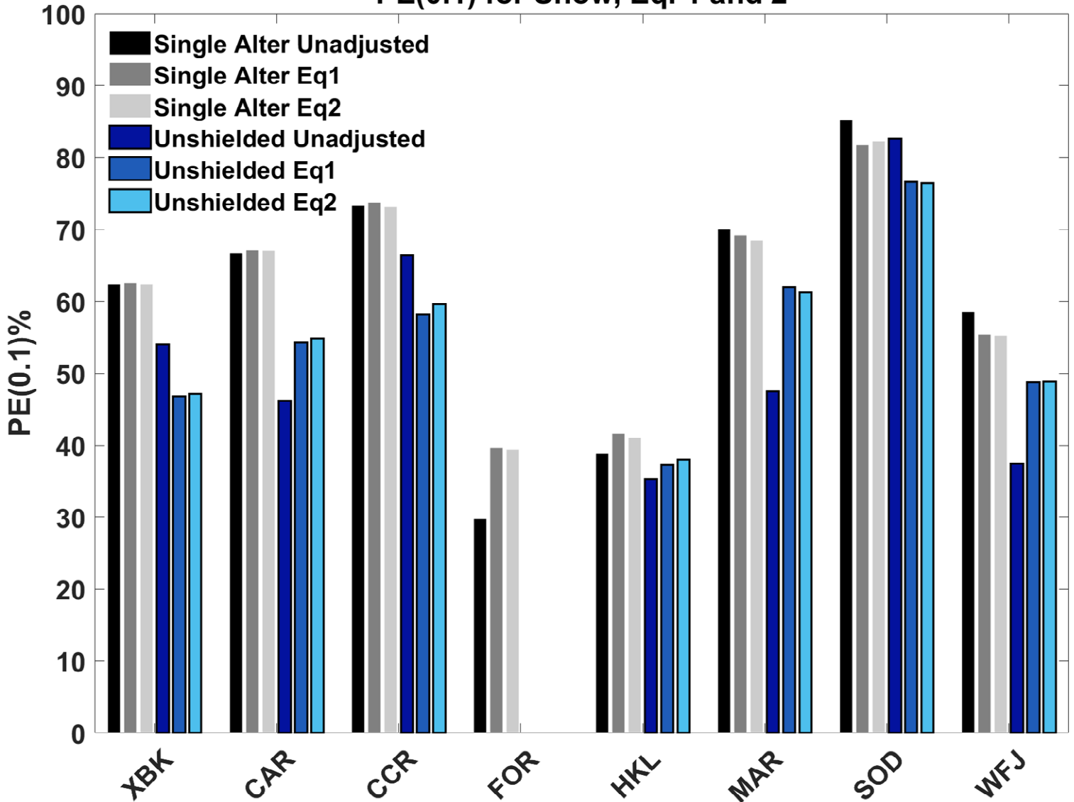
Figure 8: Percentage of events that differ from the DFAR by less than 0.1 mm for single Alter and unshielded gauges for unadjusted measurements and for adjustments using Equations 1 and 2 at each of the eight SPICE sites, combining 2015/2016 and 2016/2017 winter seasons.
