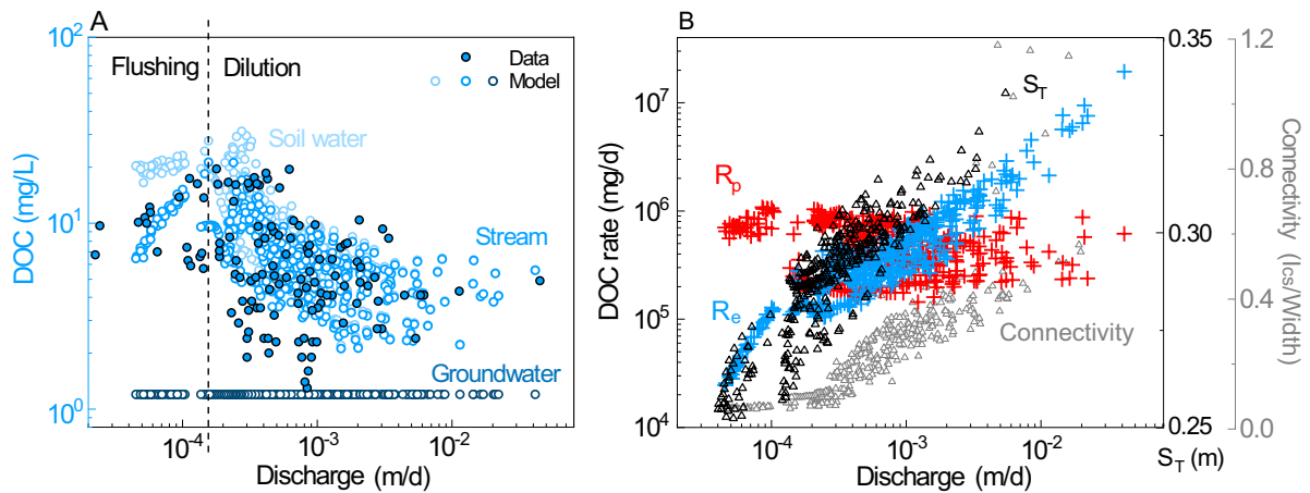
Figure 7. Relationships of daily discharge ( Q ) with: (A) stream DOC concentration; open circles are simulations; filled circles with a black outline are data; (B) soil water storage S_T , connectivity ( I_{cs}/Width ), and catchment-scale DOC export rate R_e , and DOC production rate R_p . At low Q , the stream water
